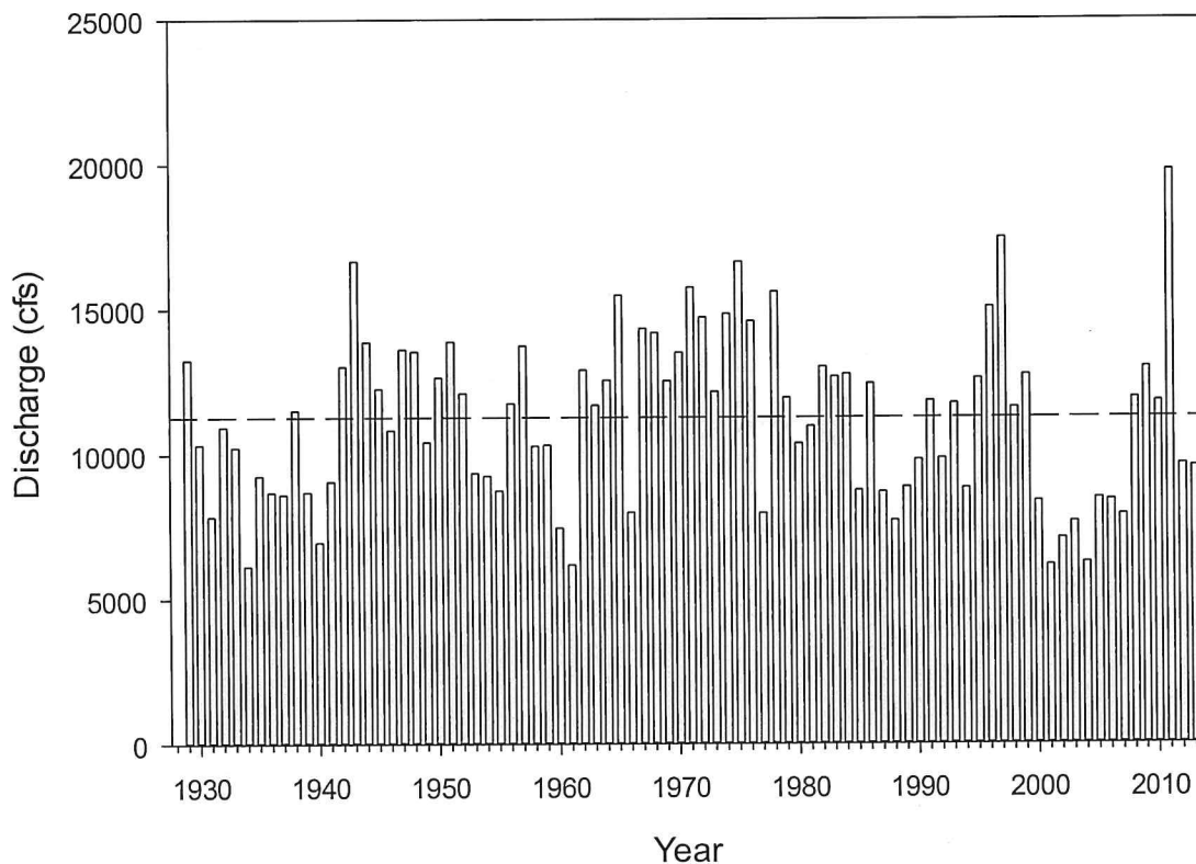
Figure 2. Mean annual discharge of the Yellowstone River at Miles City, 1929-2013. Dashed line represents mean annual discharge (11389 cfs) calculated since 1928. Data for 2013 is provisional data subject to revision.
