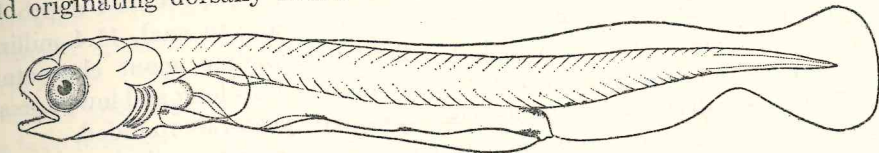
FIGURE 99.— Percina caprodes zebra , 6.6 millimeters
