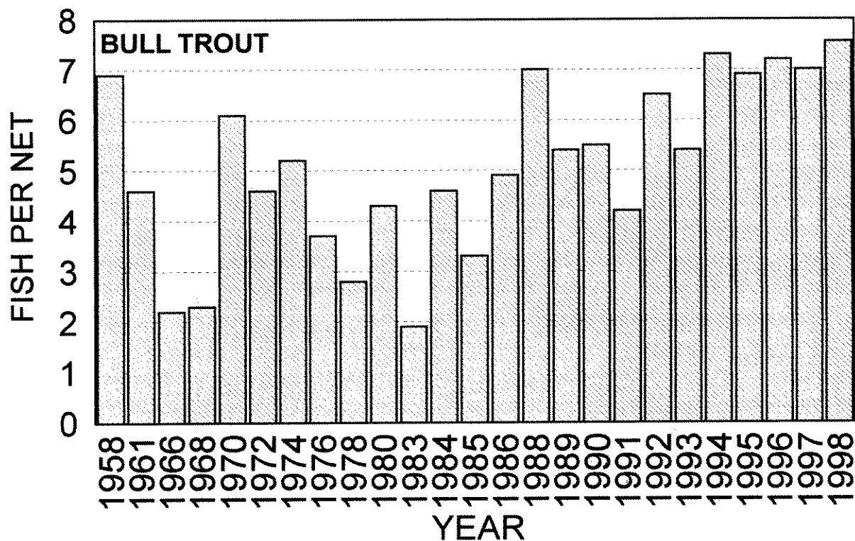
Figure 31. Fall gill net time series for westslope cutthroat trout and bull trout in Hungry Horse Reservoir. Bull trout were caught in sinking nets and cutthroat were caught in floating nets.
