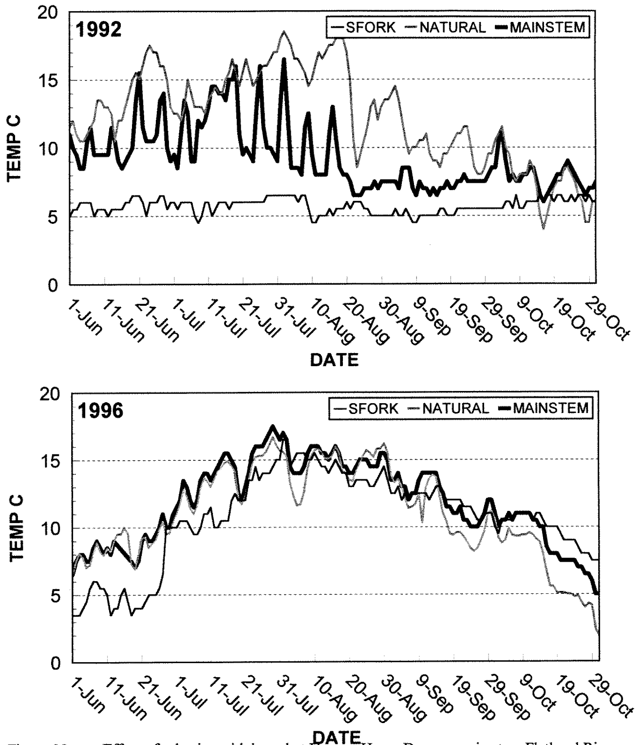
Figure 39. Effect of selective withdrawal at Hungry Horse Dam on main stem Flathead River. Conditions prior to selective withdrawal (1992, top) are compared with conditions during operation (1996, bottom). Thermograph stations were positioned in the South Fork Flathead River downstream of the dam (SFORK), at Glacier Rim in the North Fork (NATURAL), and at Columbia Falls (MAINSTEM).
