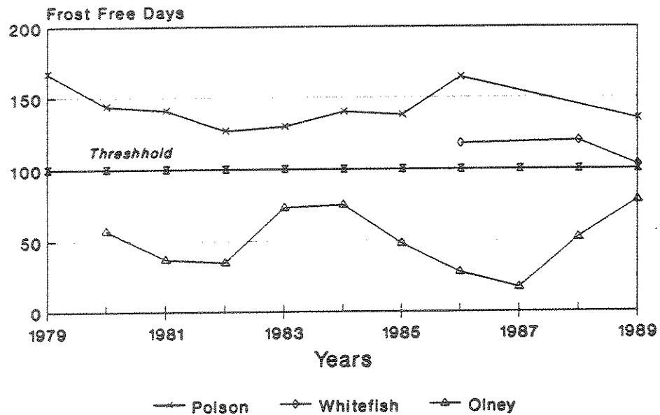
Figure 5. Comparison of number of frost-free days ( >32^{\circ}\text{F} ) from 1979-1989 for Libby and Eureka, and Polson, Whitefish, and Olney, Montana. The reported threshold for smallmouth at 100 days is indicated.
