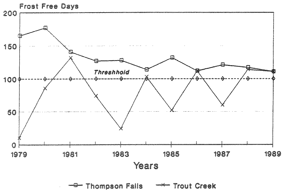
Figure 6. Comparison of number of frost-free days ( >32^{\circ}\text{F} ) from 1979-1989 for Missoula and St. Regis, and Thompson Falls and Trout Creek, Montana. The reported threshold for smallmouth at 100 days is indicated.
