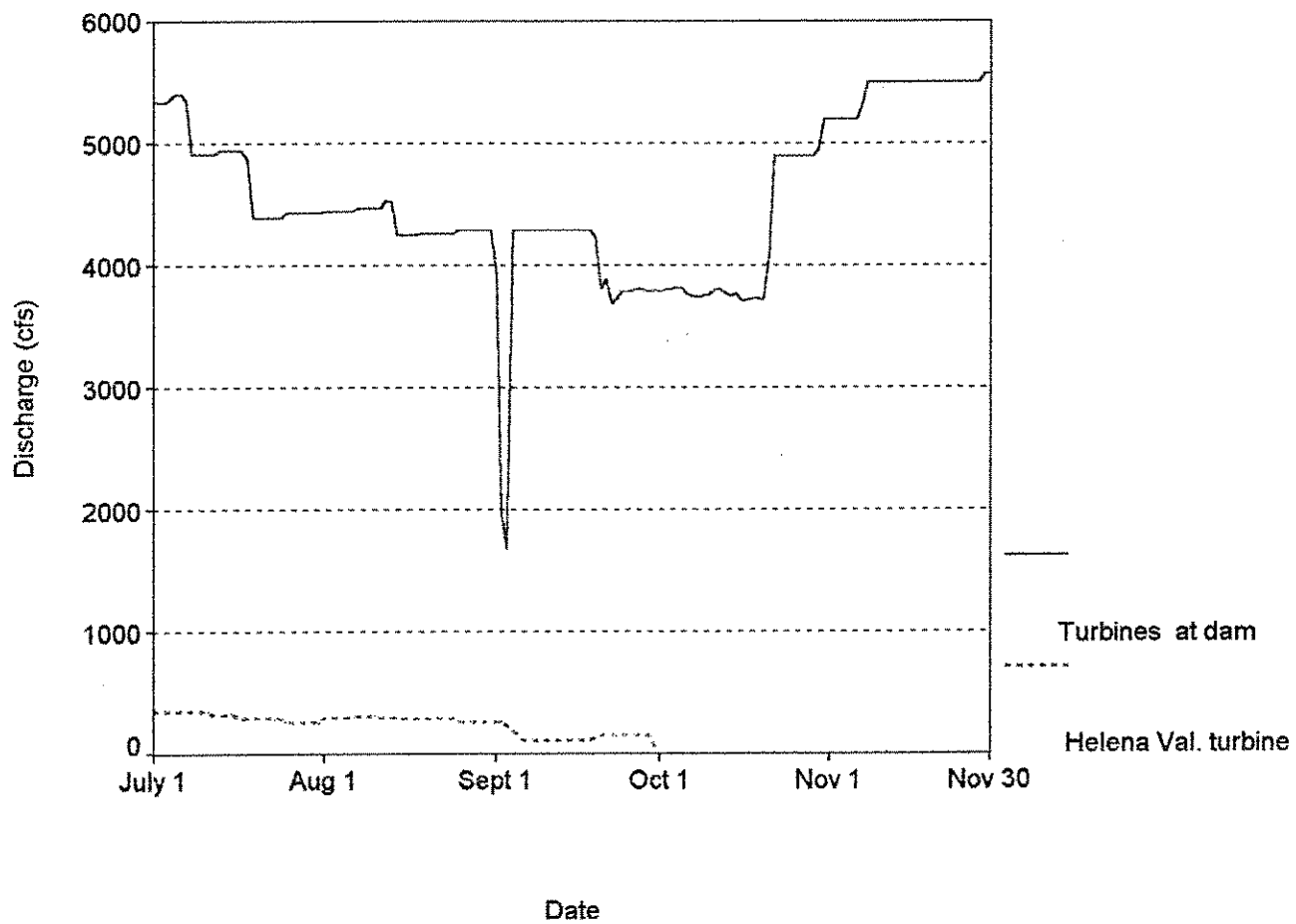
Figure 13. Discharge from Canyon Ferry Dam turbines and Helena Valley turbines, July - December, 1986.
