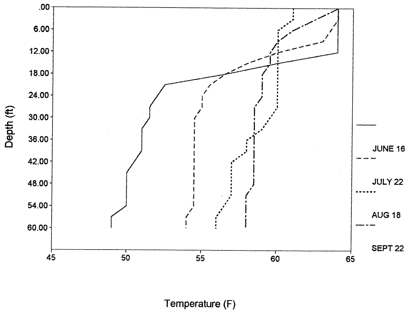
Figure 7. Temperature profiles in Hauser Reservoir, 1987.
