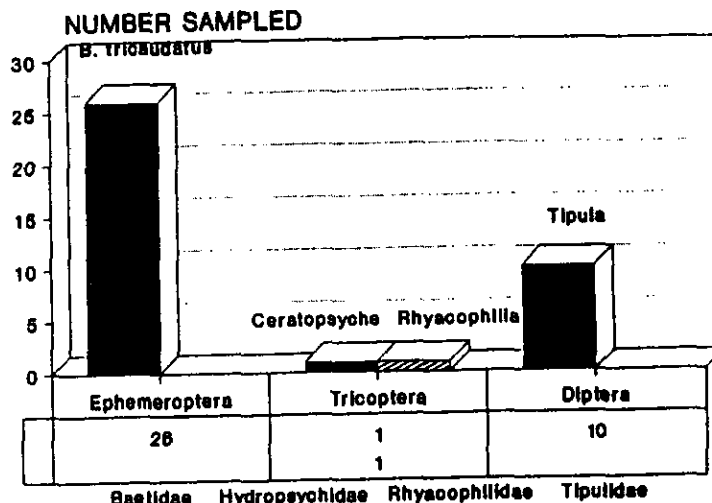
Figure 11. Insect fauna collected at the Nevada Spring Creek source, October 1989.
