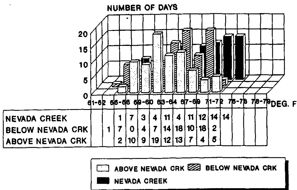
Figure 15. Maximum stream temperatures: temperature frequency distribution
