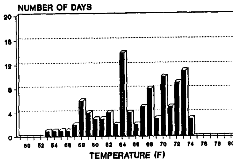
Figure 16. Maximum temperatures for Nevada Creek near the mouth, 6/22/90 - 10/1/90.
