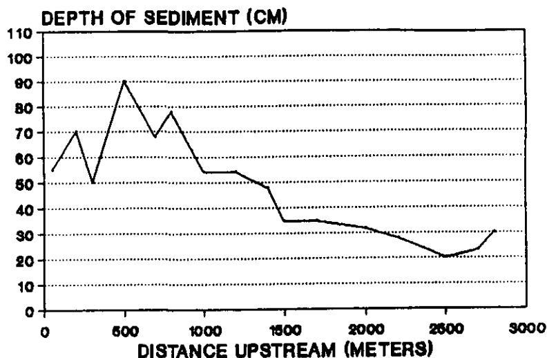
Figure 7. Depth of sediment in Nevada Spring Creek above the culvert.
