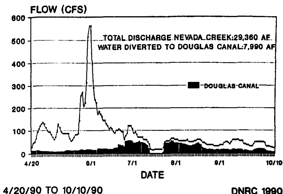
Figure 5. Discharge from Nevada Reservoir and diversion to Douglas Canal.
