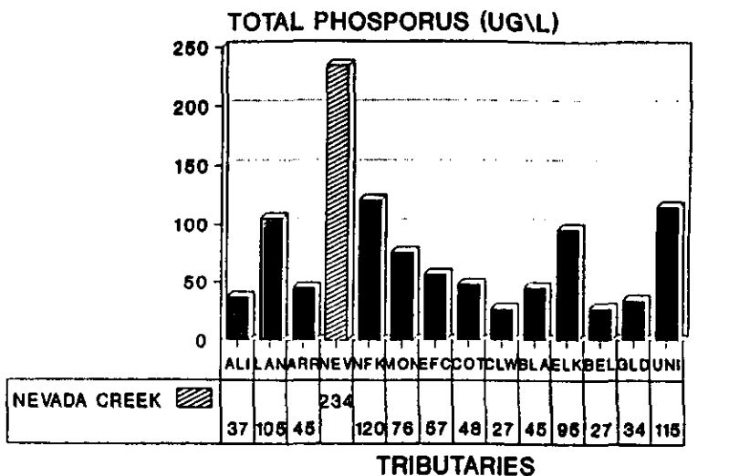
Figure 8. Tributary phosphorus concentrations.
