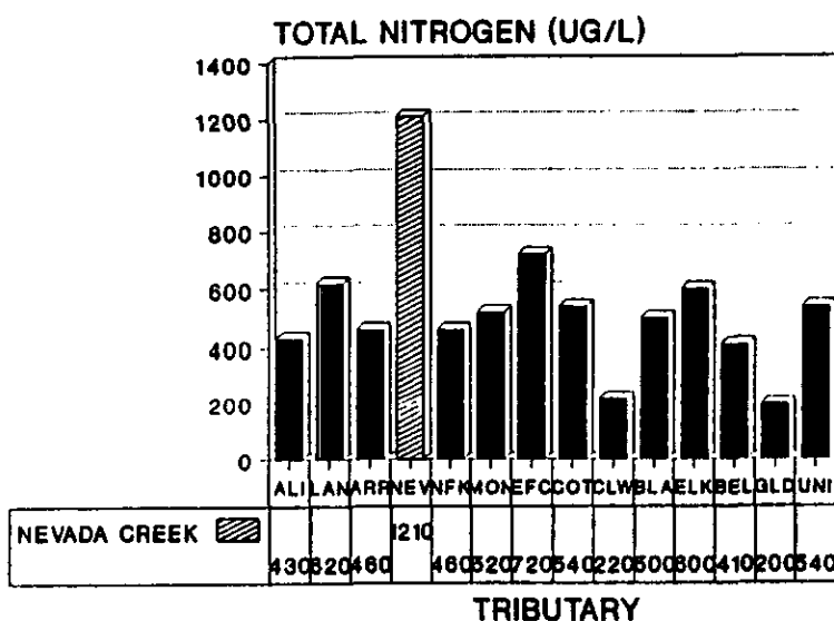
Figure 9. Tributary nitrogen concentrations.
