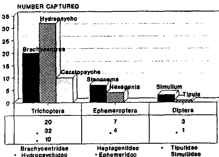
Figure 10. Insect fauna collected near the mouth of Nevada Creek, October 1990.
