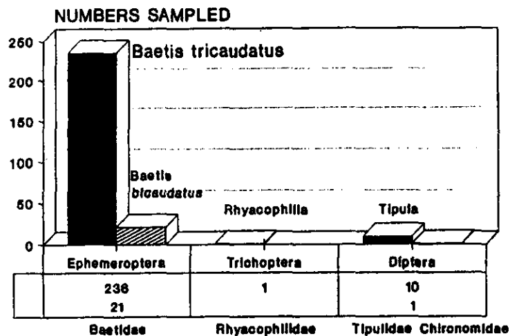
Figure 12. Insect fauna collected 200 feet below the spring source, October 1990.
