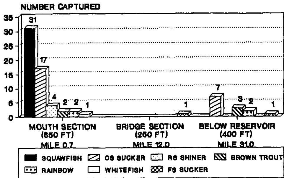
(figure 14). Figure 18. Species composition for three sections of Nevada Creek. Sculpins were observed.
