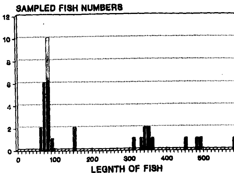
Figure 19. Length-frequency distribution for brown trout in Nevada Spring Creek.
