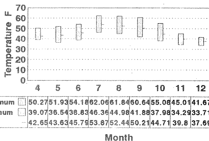
Figure 37. Summary of Water Temperatures at USFS Bridge on North Fork of Blackfoot River, 8/94 to 9/96.
