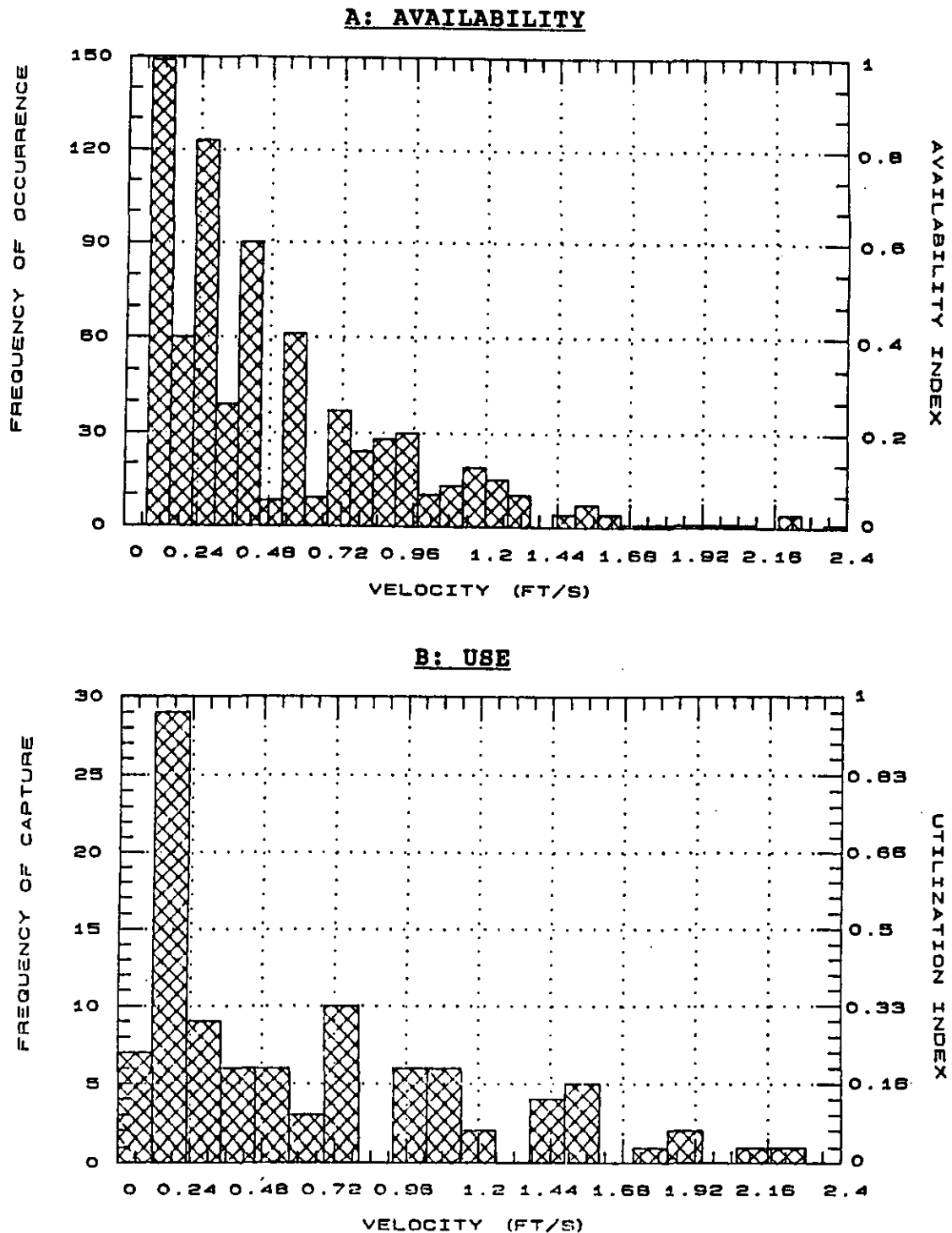
Figure 9. A. Frequency of mean velocities for macrohabitat areas of young-of-the-year Arctic grayling in the Big Hole River. B. Frequency of mean velocities at capture sites of young-of-the-year Arctic grayling in the Big Hole River.
