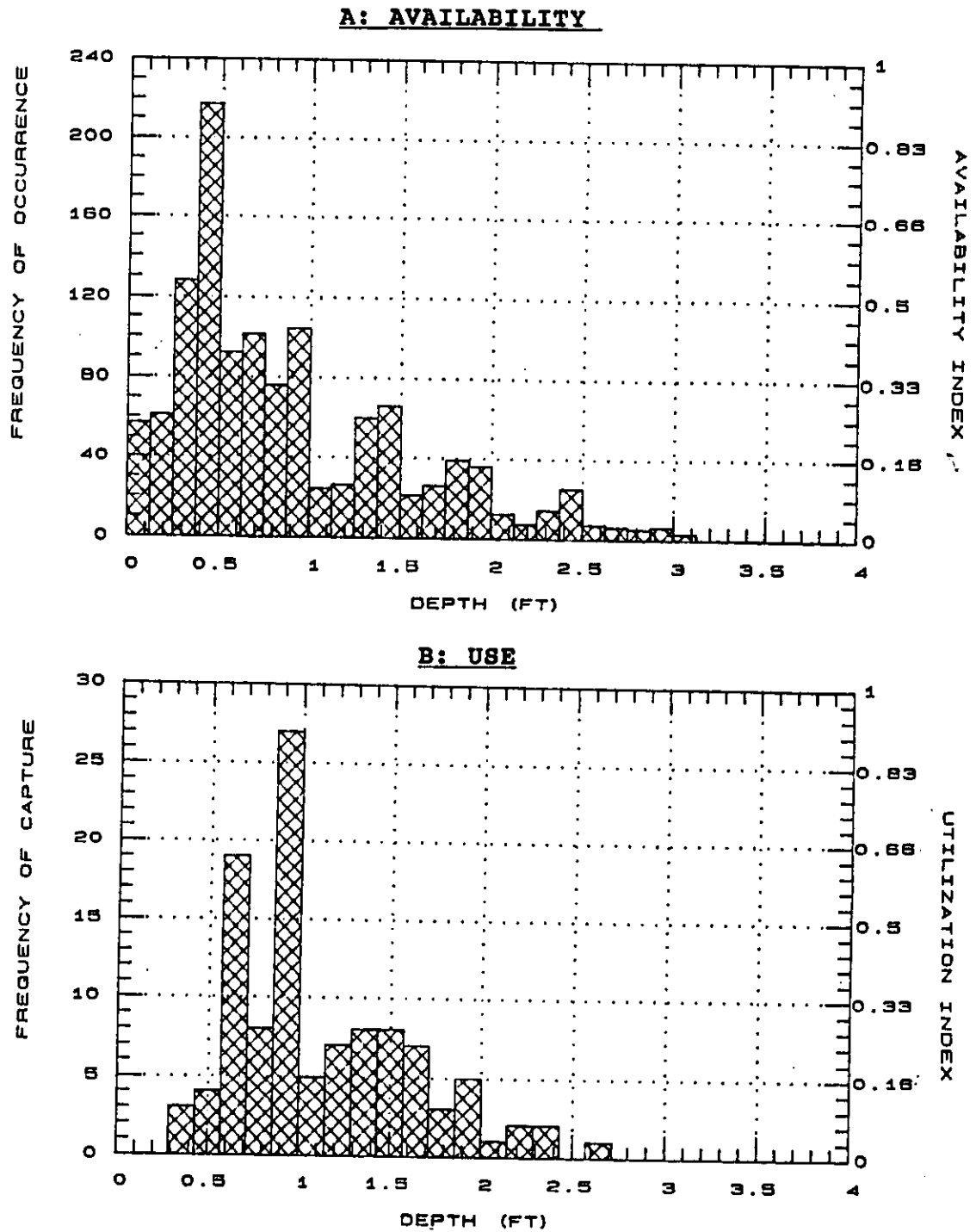
Figure 8. A. Frequency of depth measurements in macrohabitat areas of young-of-the-year Arctic grayling in the Big Hole River. B. Frequency of depth measurements at capture sites of young-of-the-year Arctic grayling in the Big Hole River.
