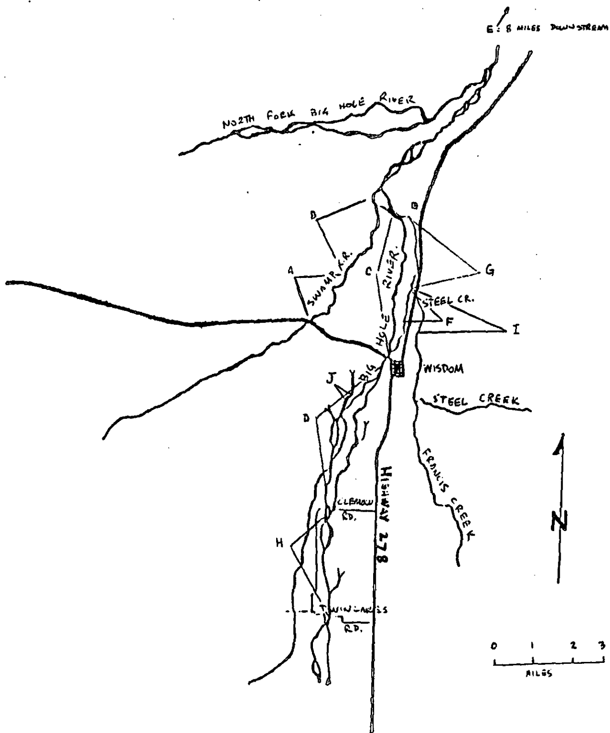
Figure 1. Map of the upper Big Hole River drainage, showing sample sections where electrofishing surveys were conducted.
