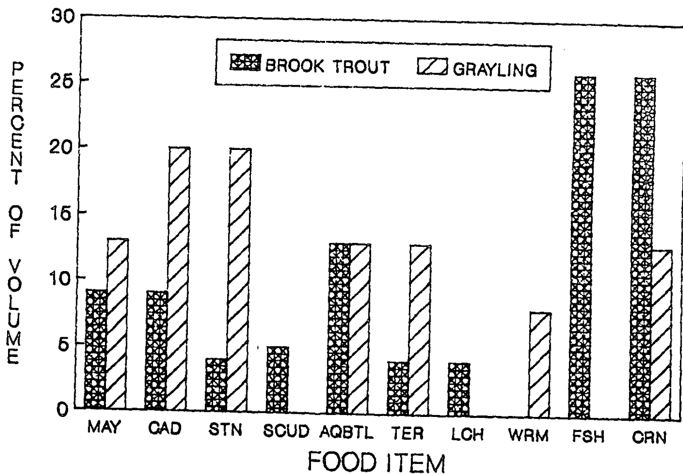
Figure 15. Percent volume of stomach contents of 10 inch and larger Arctic grayling and brook trout from the Big Hole River and its tributaries made up of various food items.
