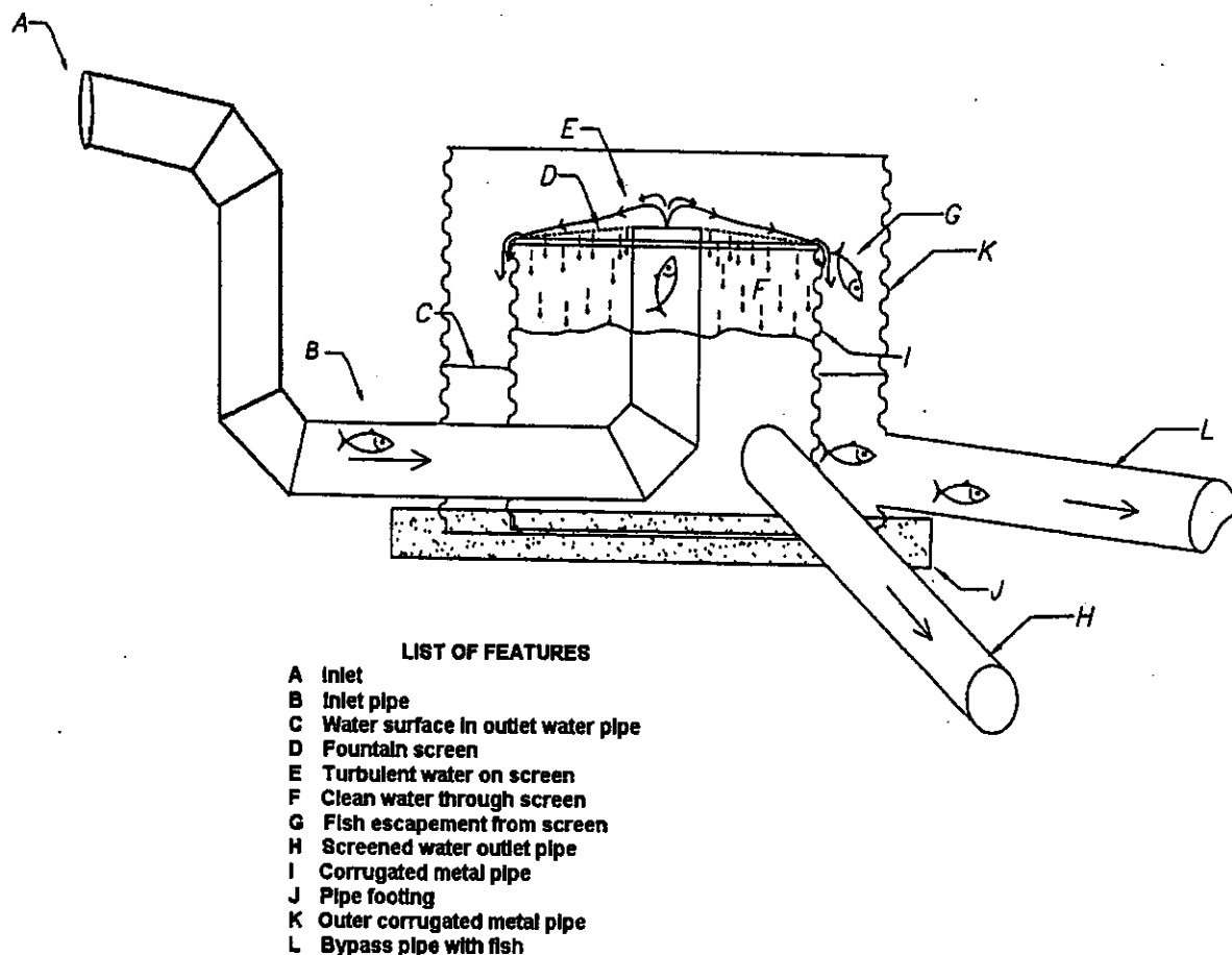
Figure 54. Conceptual design of a turbulent fountain fish screen with bypass to stream.
