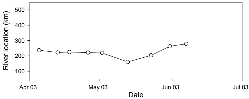
Figure 93. Movements of sauger 48.851 (N=9) during 2003 in the Yellowstone River, Montana.
