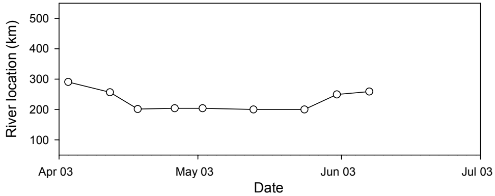
Figure 95. Movements of sauger 48.957 (N=9) during 2003 in the Yellowstone River, Montana.
