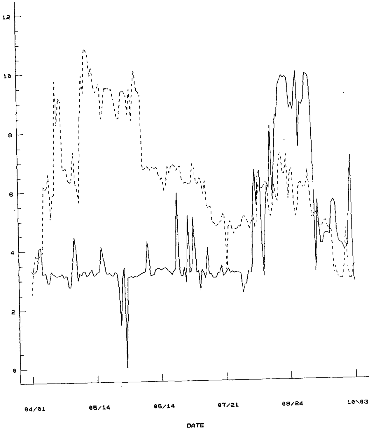
Figure 4. Representative patterns of minimum discharge at Fort Peck in an historic (1983) and a favorable (1985) year.
