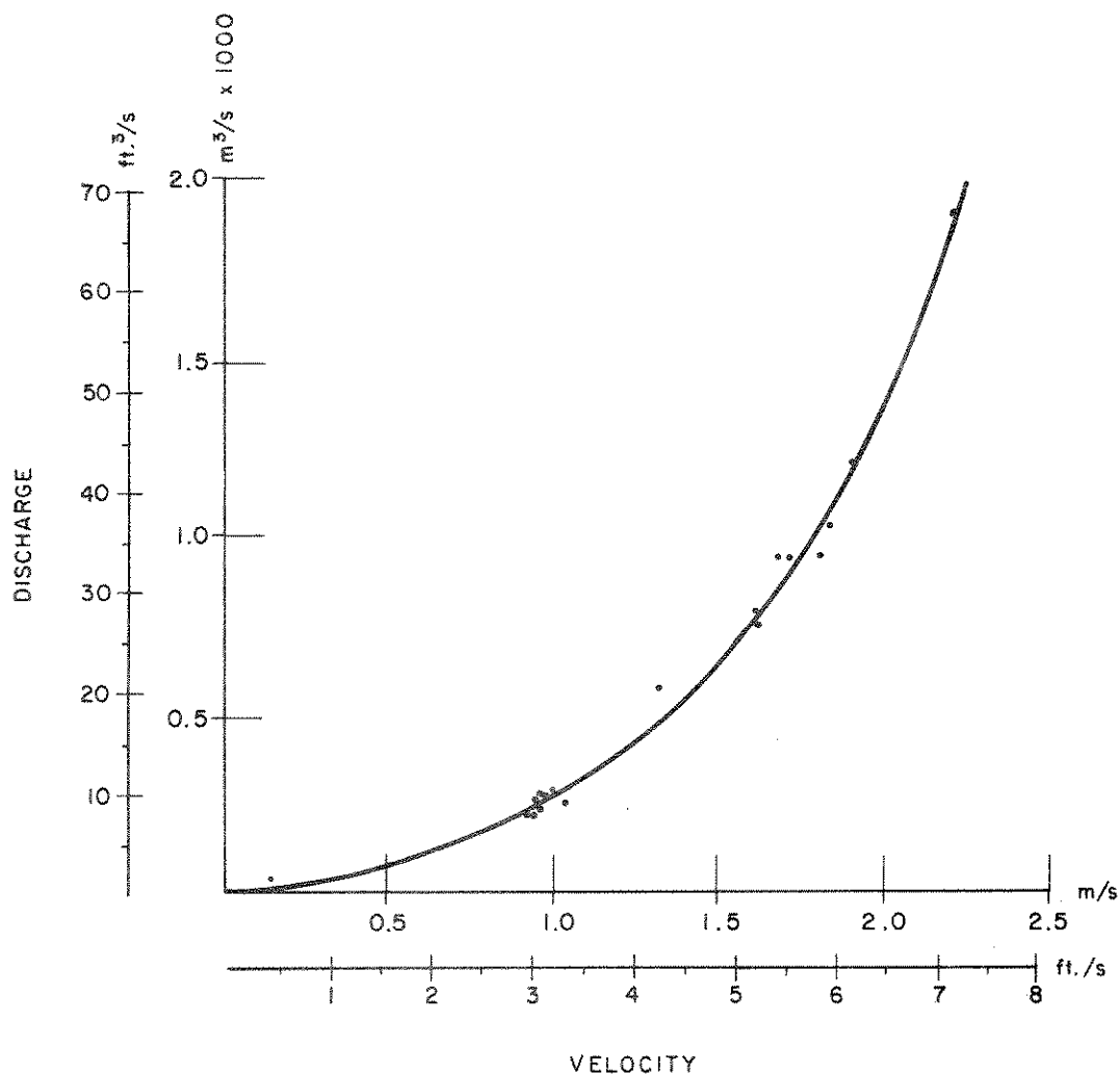
Figure B-1.-Curve illustrating the average water velocity for a cross section of the Yellowstone River at Miles City at a given flow.
