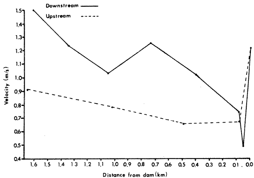
Figure 36.-Mean velocity of transects upstream and downstream from Intake diversion, Yellowstone River, at the mean annual discharge of 368.1 m³/s.
