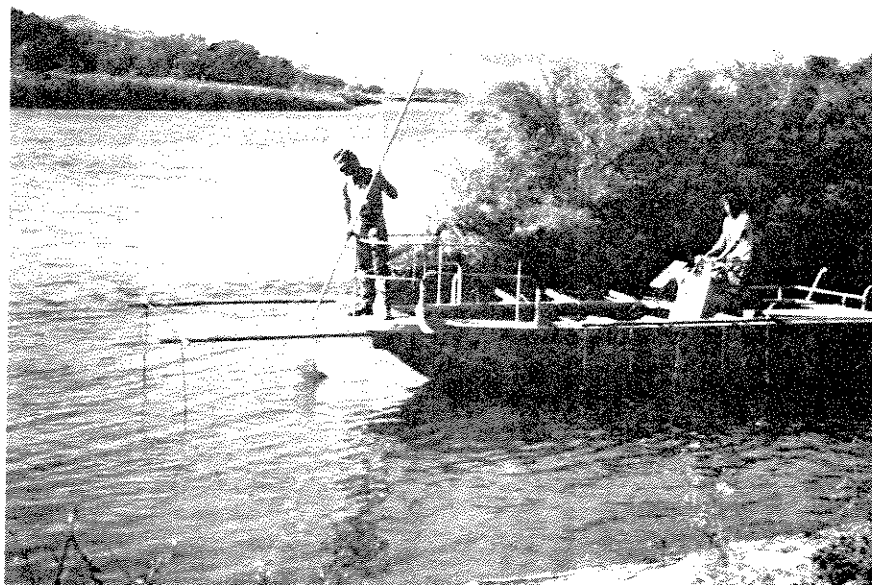
Figure B-6.-A 6.7-m (22-ft) inboard jet adapted for electrofishing on Missouri River. Photo P1279-D-79210
