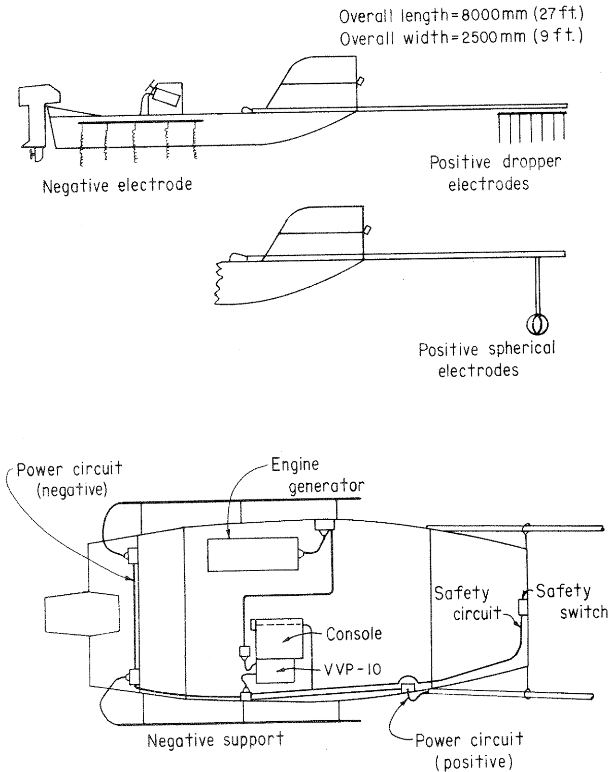
Figure B-2.-Major component location and electrode configuration.
