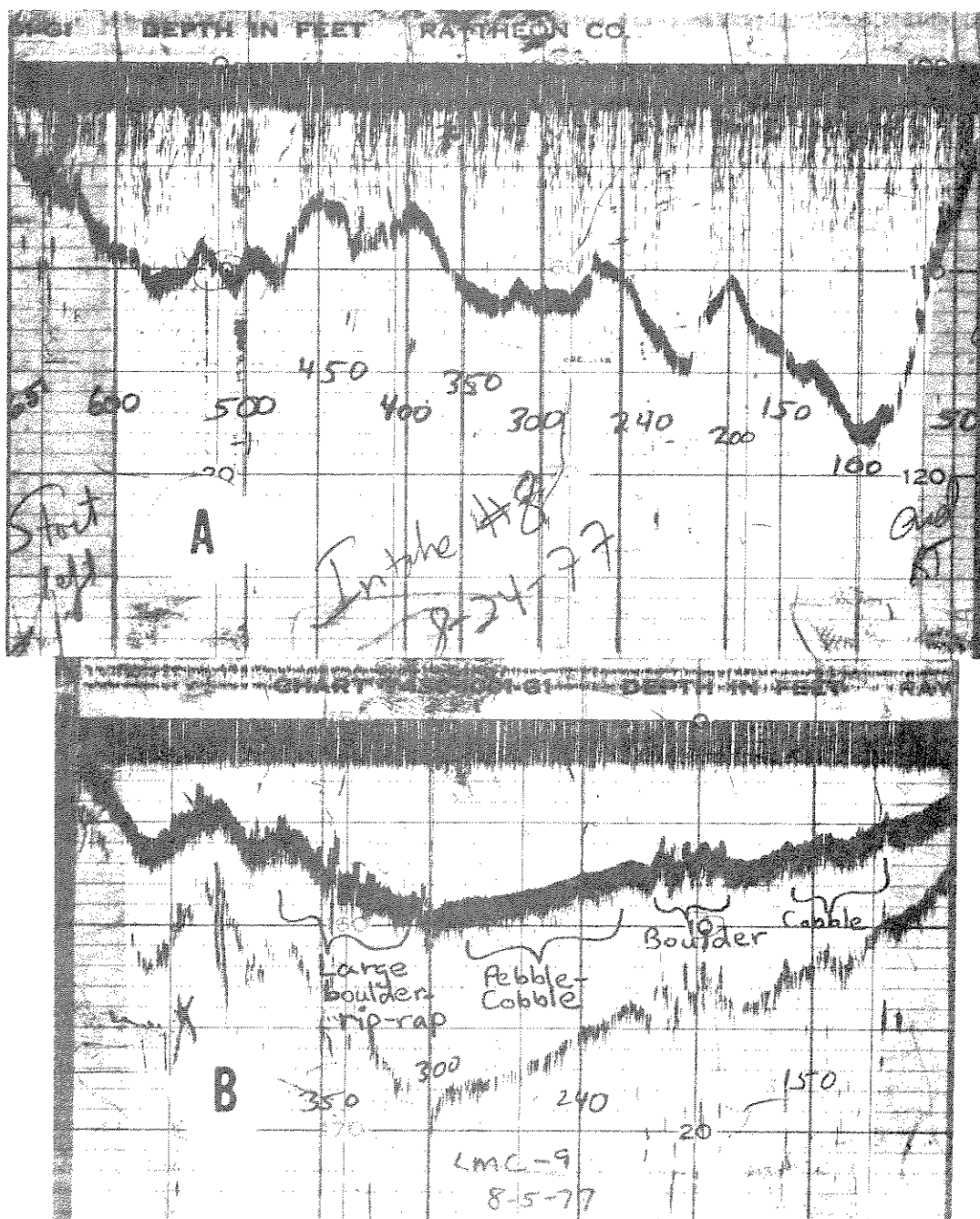
Figure 26.-Original printouts of bottom profiles taken with a constant-recording Fathometer. Each horizontal line represents 0.3 m in depth and vertical lines were automatically marked at predetermined distances from the water's edge by the boat driver. Profile A is lower Intake transect 8 and B is lower Miles City transect 9.
