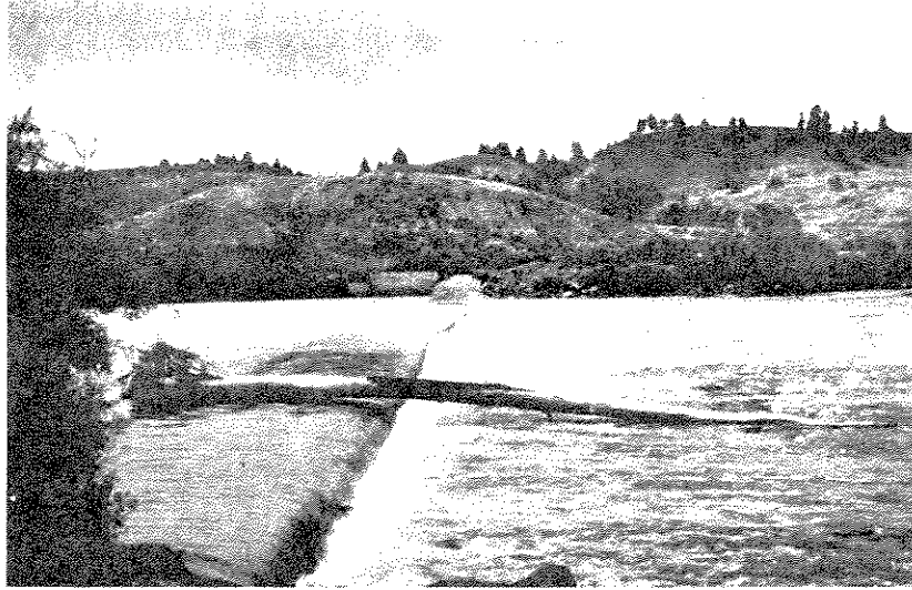
Figure 2.-Forsyth or Cartersville diversion is a concrete structure which creates approximately a 0.5-m drop in the Yellowstone River during normal summer flows. Photo P1279-D-79151
