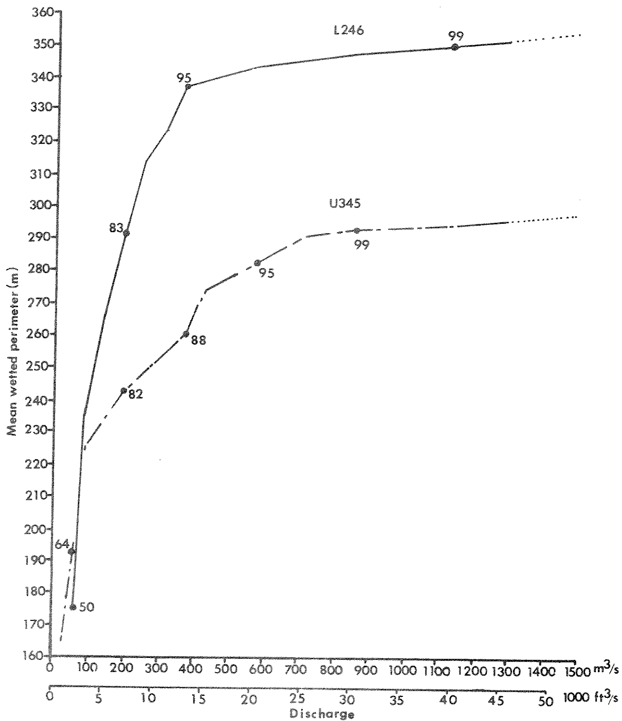
Figure 34.-Mean wetted perimeter versus discharge of three transects upstream (U345) and downstream (L246) from Intake diversion on the Yellowstone River. Percentages of projected maximum wetted perimeter during bank-full flow are given.
