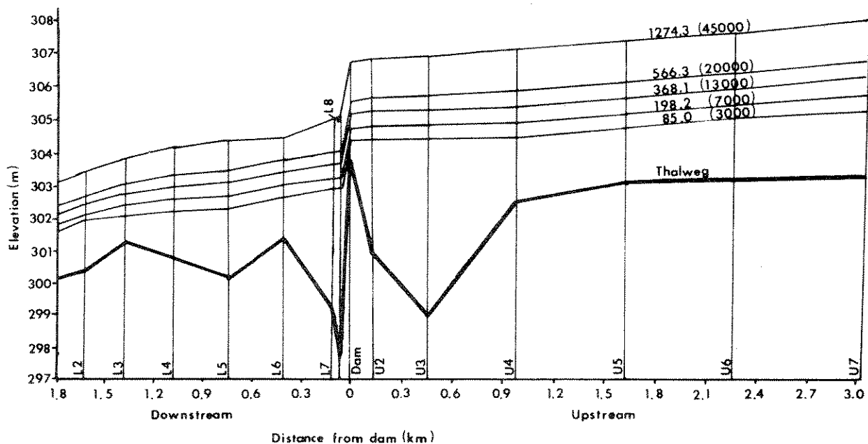
Figure 29.-Thalweg and predicted water surface elevations at various discharges in \text{m}^3/\text{s} for transects upstream (U) and downstream (L) from Intake diversion dam, Yellowstone River.
