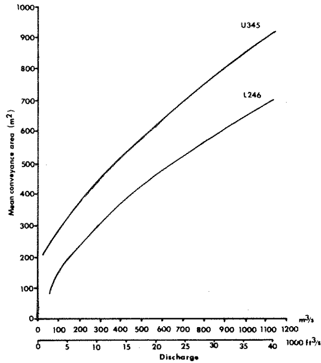
Figure 35.-Mean conveyance area of upper transects 3, 4, and 5 (U345) above Intake diversion and lower transects 2, 4, and 6 (L246) below Intake diversion, Yellowstone River.
