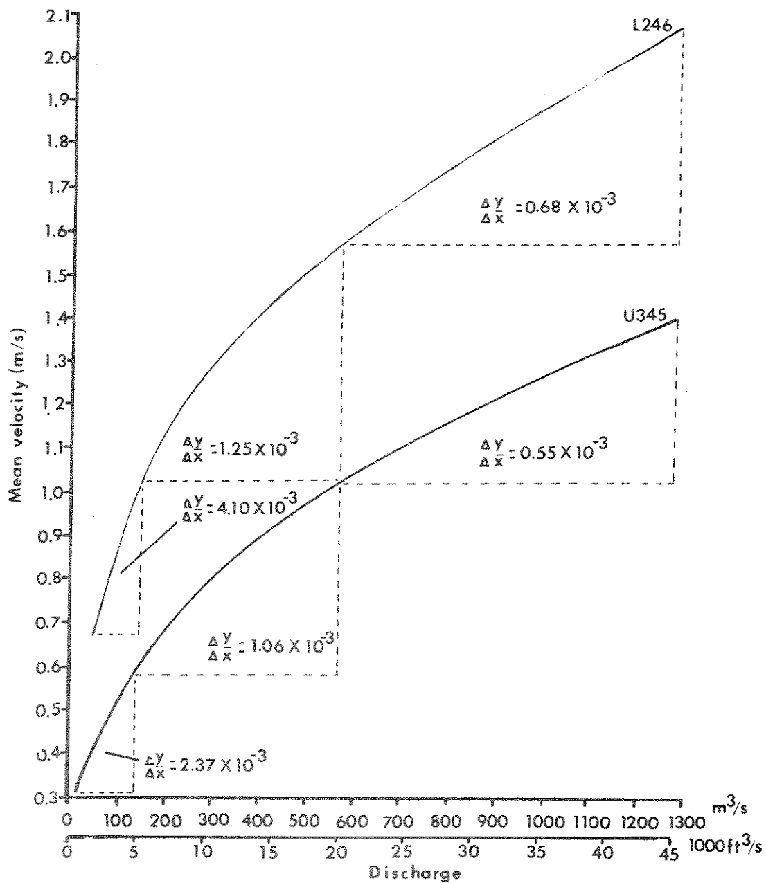
Figure 37.-Grand mean velocity versus discharge of three cross sections upstream (U345) and downstream (L246) from Intake diversion, Yellowstone River.
