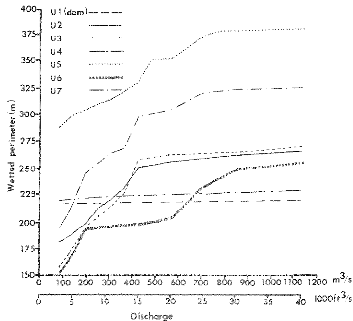
Figure 32.-Wetted perimeter versus discharge for seven transects (U1 through U7) on the Yellowstone River above Intake diversion.
