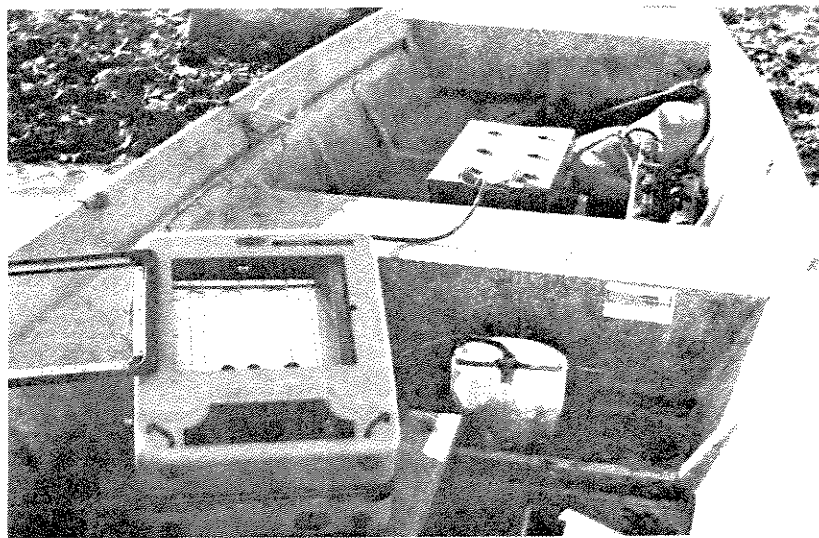
Figure 25.-This portable, constant-recording Fathometer had a variable depth scale and a fix marker. The transducer was submerged inside the cylinder and could transmit through the hull. A large 12-V diesel truck battery was used for the power source. Photo P1279-D-79209
