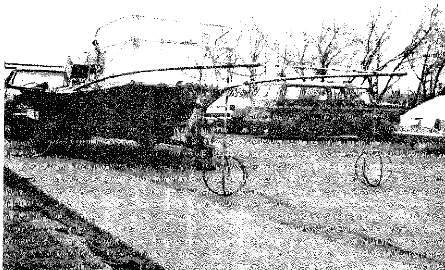
Figure B-5.-Positive spherical electrodes. Photo P1279-D-79205
