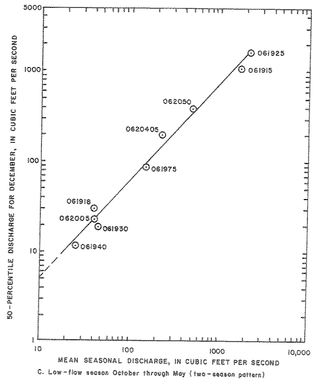
Figure 4.--Regression equations relating monthly percentile discharge to mean seasonal discharge at nine gaged sites.
