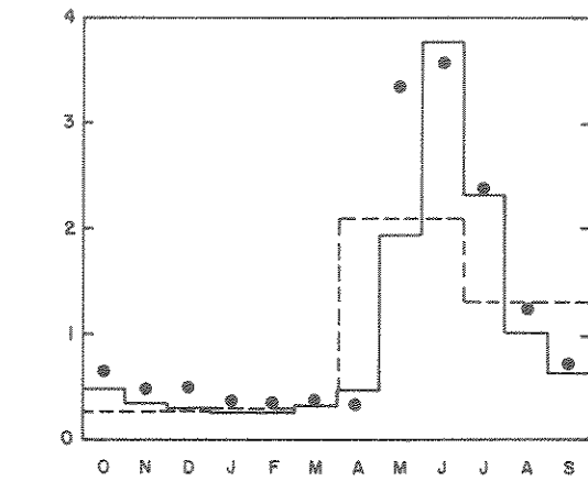
A. Yellowstone River at Corwin Springs (station 06191500) Drainage area = 2623 square miles
