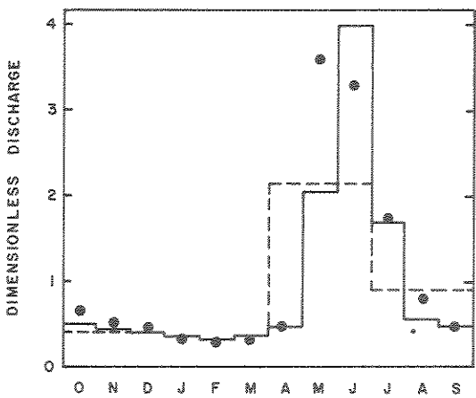
B. Big Creek near Emigrant (station 06191800) Drainage area = 60.9 square miles
