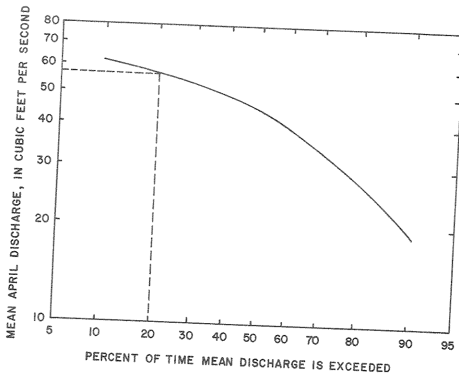
Figure 3.--Flow-duration curve of mean April discharge for Big Creek near Emigrant.
