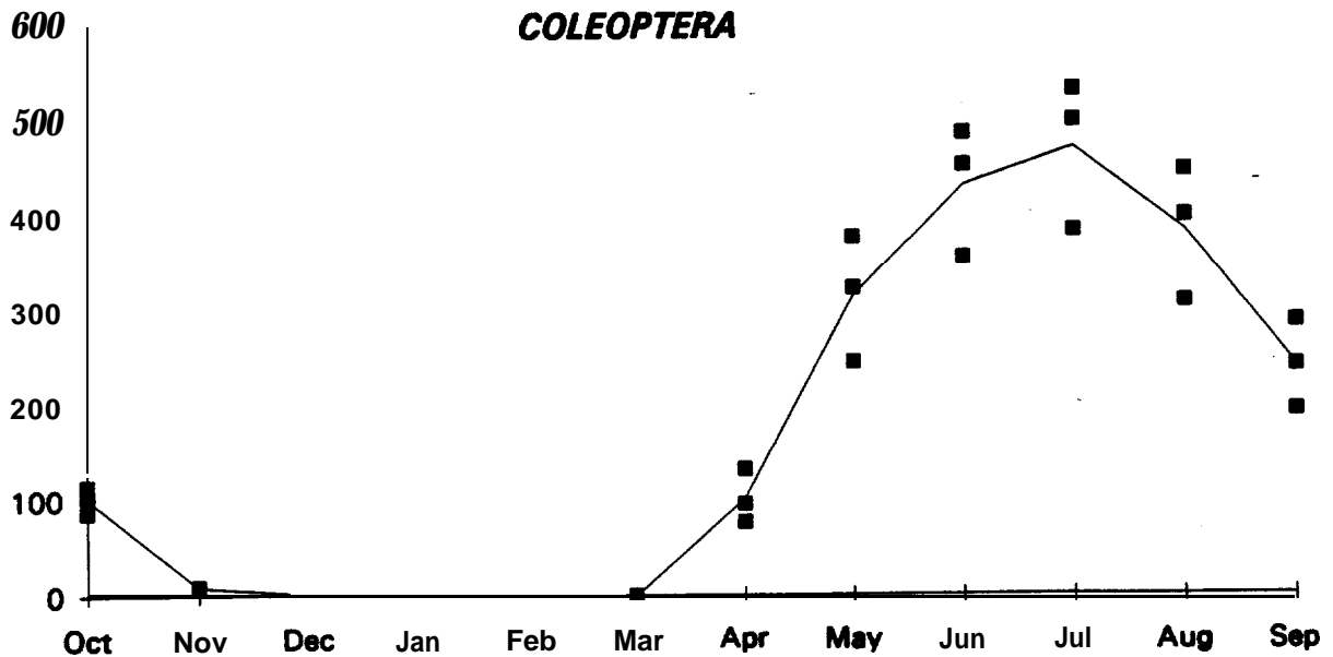
Figure 17. Seasonal distribution of Coleoptera deposited on the reservoir surface from the surrounding landscape. Coleopterian deposition was measurably greater in nearshore (< 100 m) areas at both reservoirs. The line represents average conditions; points reveal the range under normal operating conditions.
