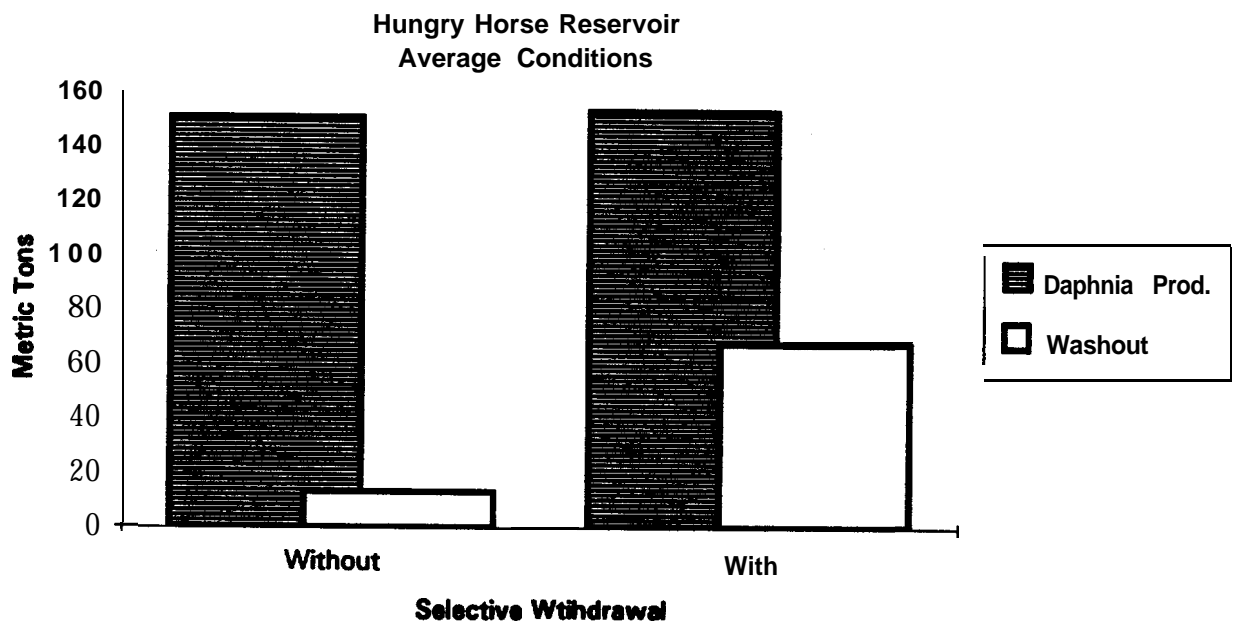
Figure 32. A comparison of daphnia production and washout from the dam under fixed hypolimnetic discharge and selective withdrawal. Downstream loss is increased when warm water is withdrawn from productive surface layers. Model simulation indicates that zooplankton production is somewhat higher under selective withdrawal.
