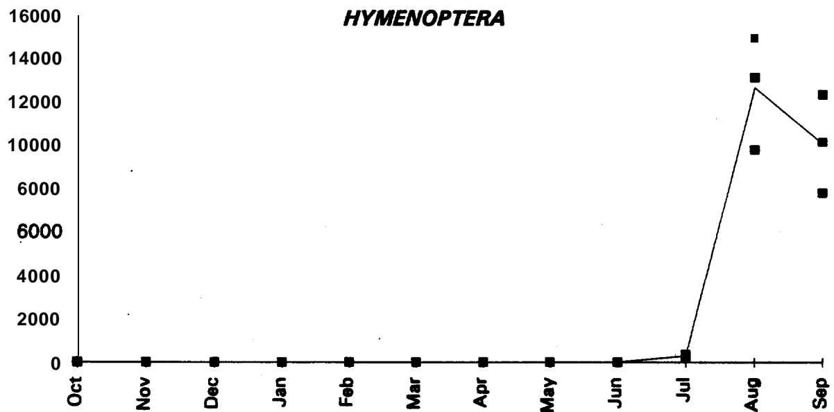
Figure 20. Seasonal distribution of Hymenoptera deposited on the reservoir surface from the surrounding landscape. Hymenopteran deposition was randomly distributed across the reservoir surface. The line represents average conditions; points reveal the range under normal operating conditions.
