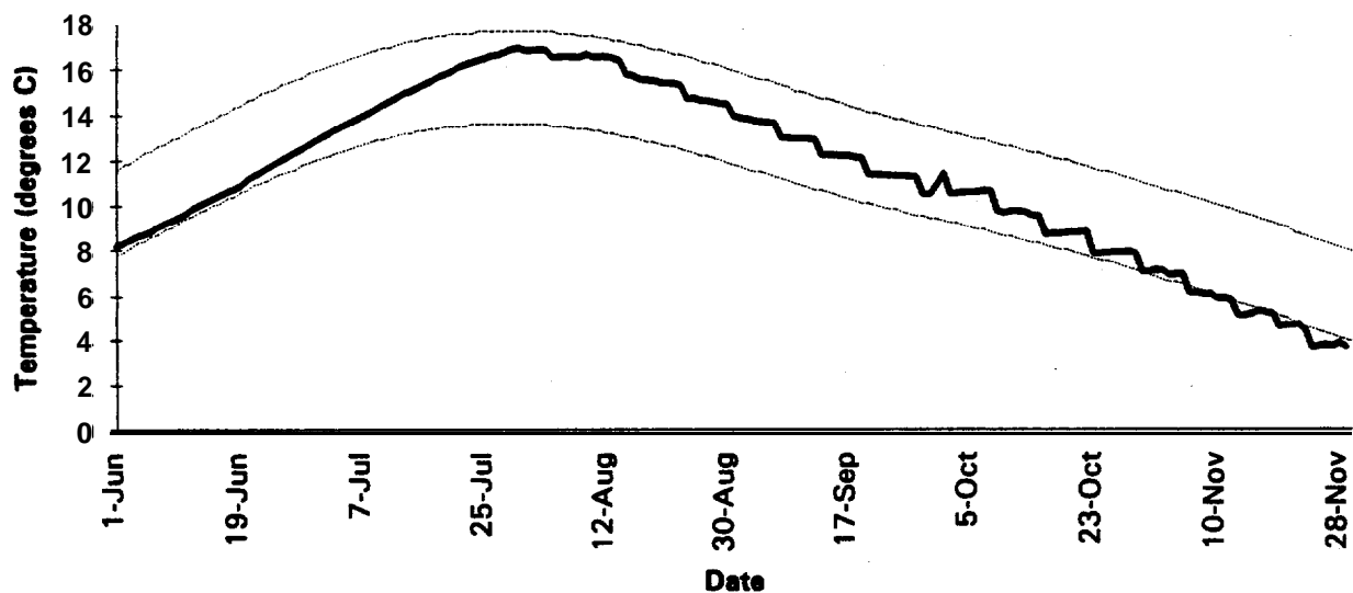
Figure 29. Thermal control resulting from selective withdrawal. Dashed line bracket the natural temperature range during the peak growth period. These results are based on average long-term conditions. Complete control is possible under all water conditions observed historically, 1928 through present.
