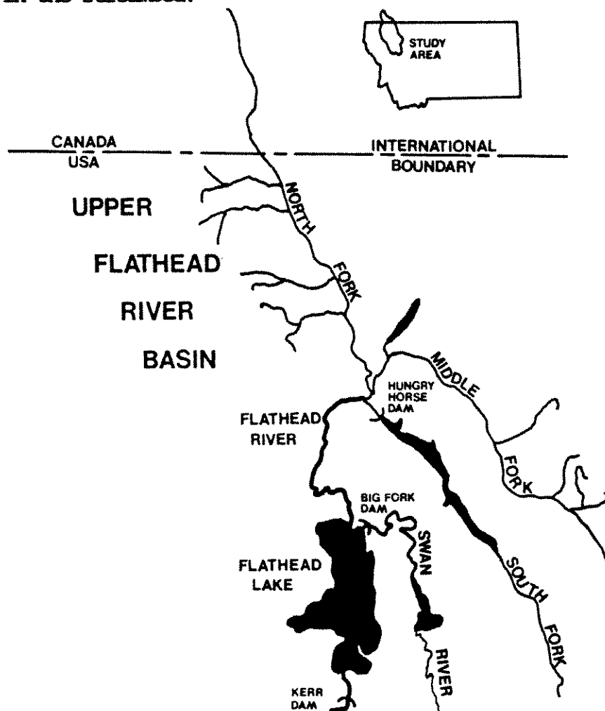
Figure 1. The Upper Flathead Drainage
