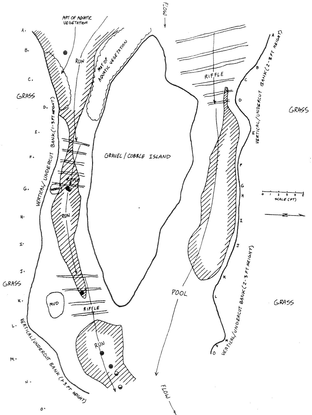
Figure 19. Physical features of intensive-use area "C" on the Big Hole River, indicating riffusable area (area delimited by shading) for YOY Arctic grayling. Solid circles and half-solid circles indicate capture sites for YOY Arctic grayling from the first and second electrofishing surveys, respectively.
