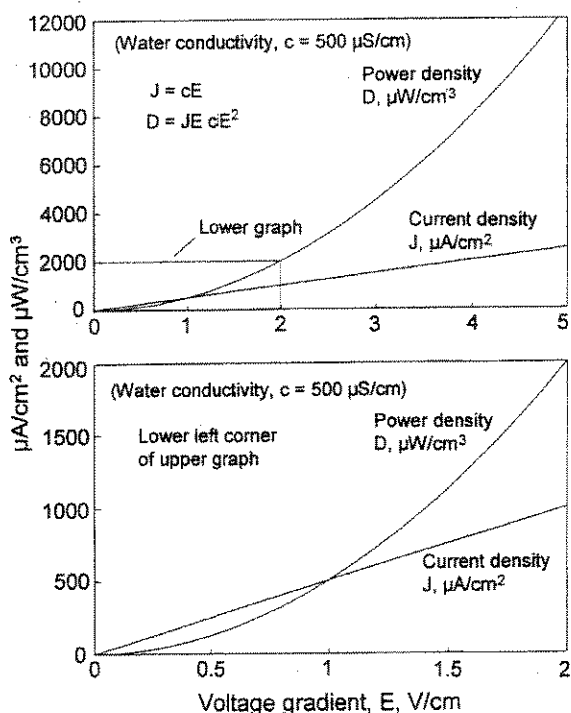
Fig. 8. Changes in current density and power density relative to voltage gradient in water with a conductivity of 500 \cdot \text{S}/\text{cm} . (For other conductivities, adjust the values along the vertical axis in direct proportion to the change in conductivity—e.g., for half the conductivity, 250 \cdot \text{S}/\text{cm} , halve the values along the Y-axis.)
