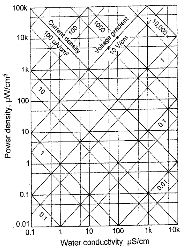
Fig. 6. Four-way logarithmic graph of relations among measures of electrical-field intensity (power density, current density, and voltage gradient) relative to water conductivity. Reproduced with permission from Fig. 7 in Kolz, 1989a; axis labels modified.)
