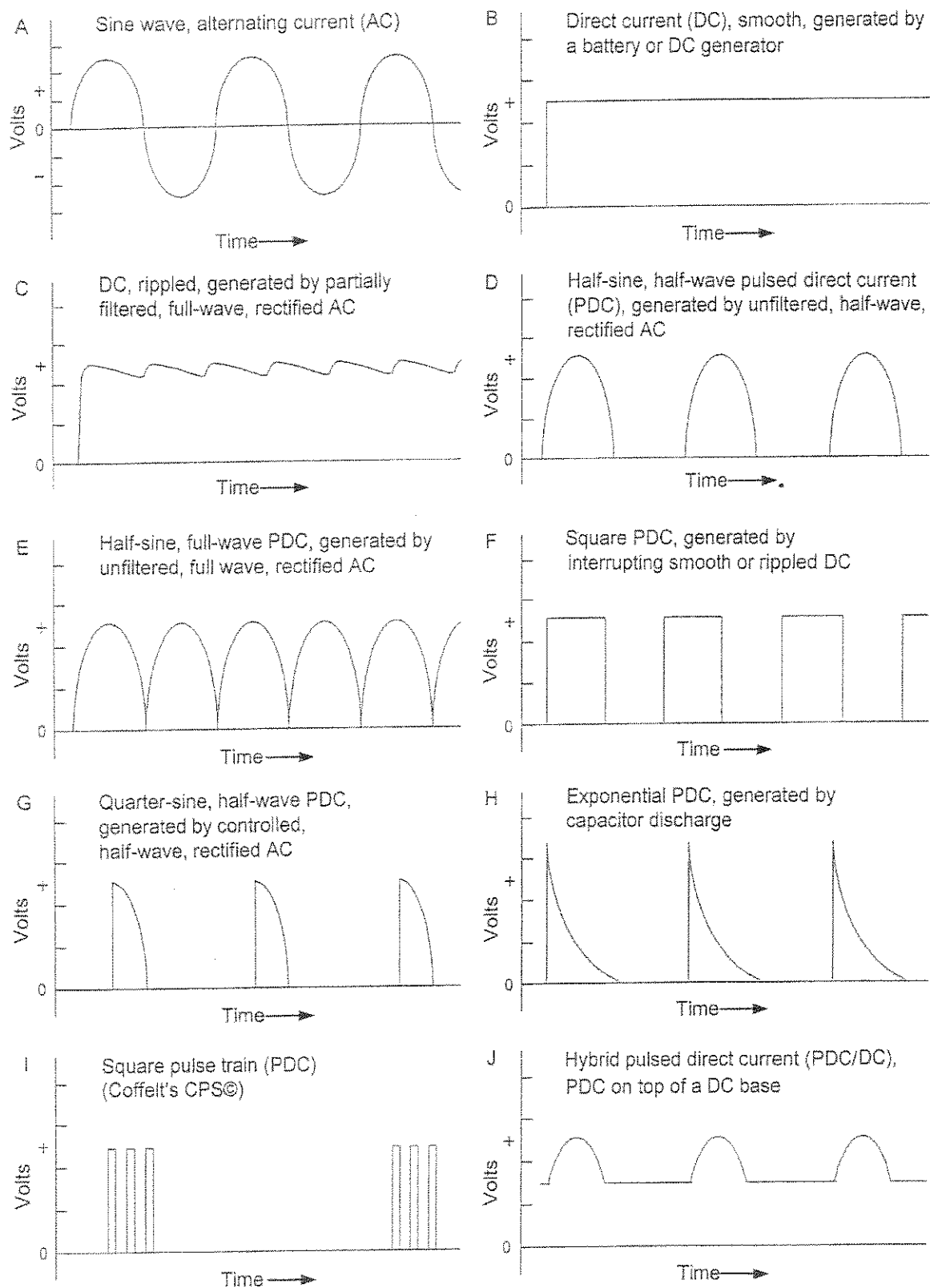
Fig. 5. Selected waveforms used in electrofishing.
