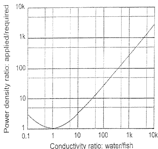
Fig. 12. Power-density-transfer curve. (Represents the relation D_w/D_f = (1 + q)^2/(4q) , where q = c_w/c_f (the conductivity mismatch ratio, water to fish) for predicting the increase in applied power density in water ( D_w ) necessary to maintain a constant transfer of required power density (e.g., that for a desired response) to the fish ( D_f ) as the conductivity ratio ( \bar{a} ) increases or decreases from unity with changes in water conductivity. This relation was derived from concepts of normalized power and load mismatch by Kolz, 1989a and is fundamental to his theory of power transfer for electrofishing. Reproduced with permission from Fig. 1 in Kolz and Reynolds, 1989b; axis labels modified.)
