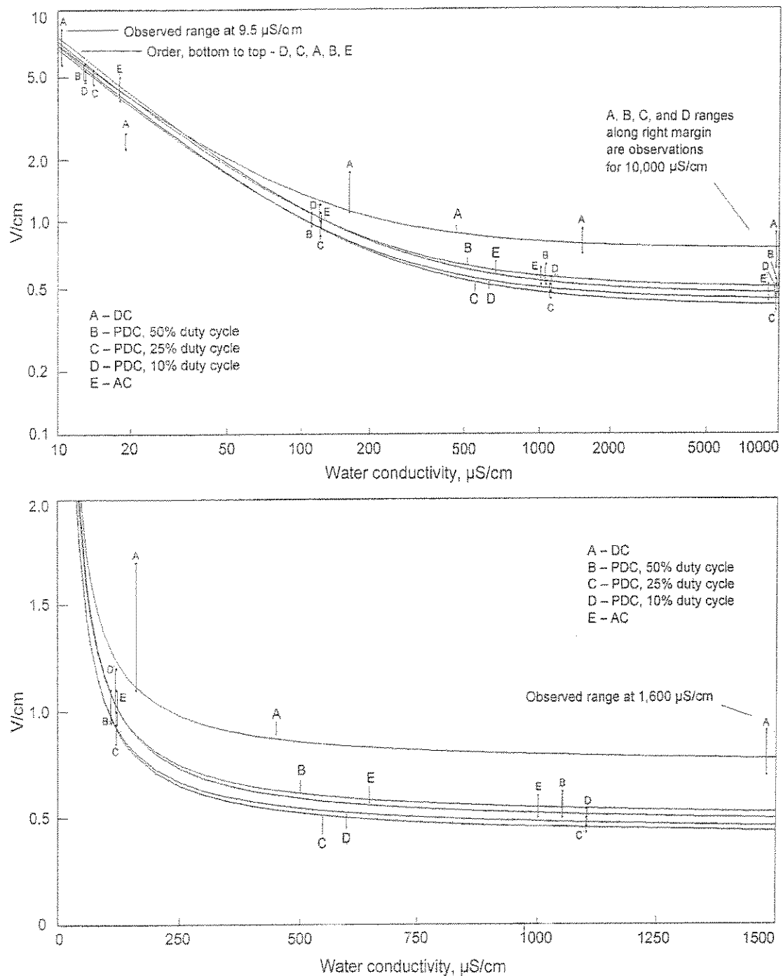
Fig. 14. Peak-voltage-gradient-threshold curves for narcosis (stun) of 6- to 9-cm-TL goldfish ( Carassius auratus ) in homogeneous fields of DC; 50-Hz, square-wave PDC with duty cycles of 50%, 25%, and 10%; and 60-Hz sinusoidal AC. (These in-water curves are an alternative representation of the power-density-transfer curves for narcosis in Figs. 6•40 of Kolz and Reynolds, 1989b. The vertical ranges denoted by small capital letters and associated with each curve approximate the corresponding ranges of experimental threshold data provided in Kolz and Reynolds graphs.)
