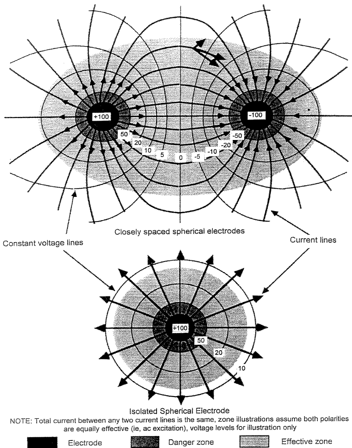
Fig. 9. Hypothetical two-dimensional diagrams of heterogeneous electric fields around and between electrodes. (When electrodes are sufficiently far apart, the field around each is essentially isolated as indicated in the lower diagram. Voltage is relative to that of the water where voltage gradient is minimal. Constant-voltage (isopotential) lines are perpendicular to the radiating lines of current. Contrary to the diagrams, current flows from negative to positive electrodes. Reproduced with permission from Fig. 3.10 in Novotny, 1990.)
