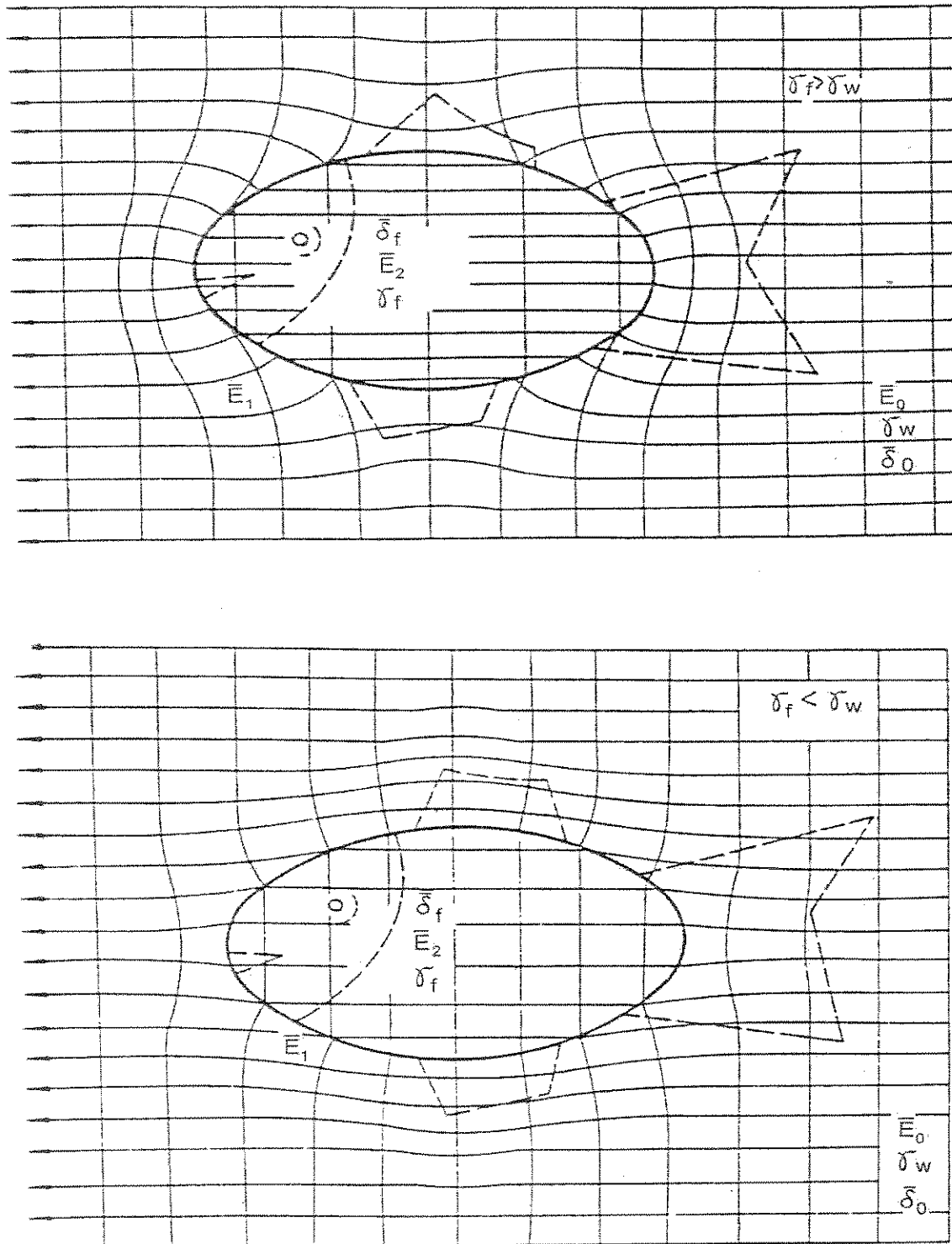
Fig. 10. Distortion of homogenous electric fields around fish in water that is less conductive (top) and more conductive (bottom) than the fish. (Horizontal lines are current (flux) lines and vertical lines are constant-voltage (isopotential) lines. Symbol \bar{\sigma} = conductivity ( c ), E = voltage gradient, and \delta = current density ( J ). Reproduced from Figs. 77 and 78 in Sternin et al., 1976.)
