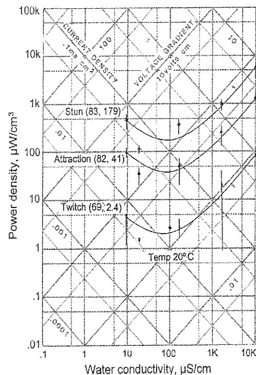
Fig. 13. Power-density-transfer curves fitted to peak-power-density threshold data for twitch, taxis (attraction), and narcosis (stun) in 6- to 9-cm-TL goldfish ( Carassius auratus ) subjected to homogeneous fields of DC. (Range and means of experimental data are represented by vertical bars and associated point symbols, respectively; ma = milliamperes or 1,000 microamperes. Reproduced with permission from Fig. 6 in Kolz and Reynolds, 1989b; axis labels modified.)
