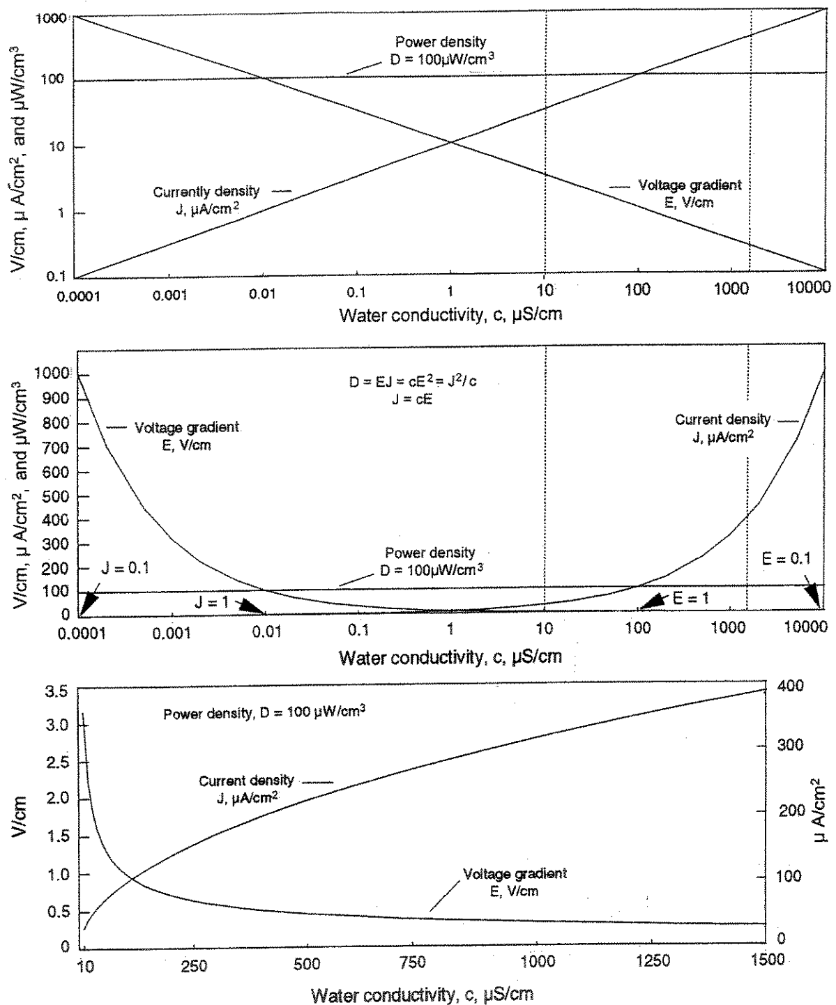
Fig. 7. Changes in voltage gradient and current density relative to water conductivity at a constant power density of 100 \cdot \text{W/cm}^3 . (Top and middle graphs are the same except the Y-axis is logarithmic in the top graph and arithmetic in the middle graph. Bottom graph is limited to the range of conductivities typical of fresh waters and bounded by dotted vertical lines in the upper graphs; both axes are arithmetic with different Y-axis scales for voltage gradient and current density.)
