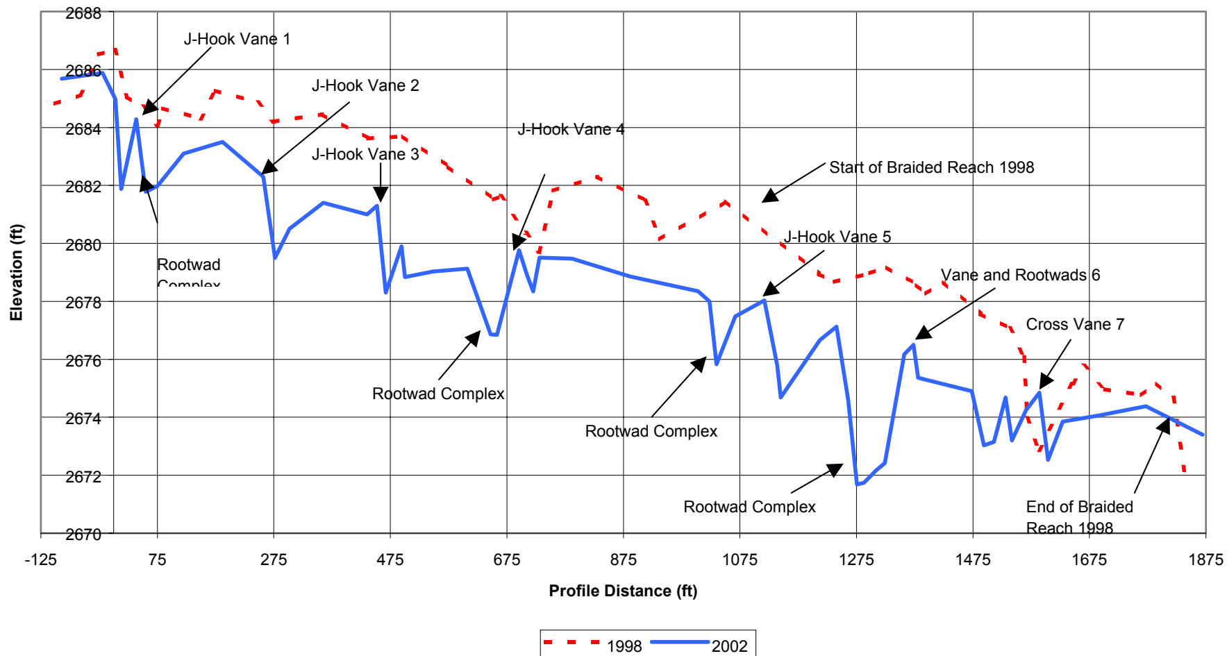
Figure 8. The longitudinal profile survey of the Libby Creek Demonstration Project before (1998) and after (2002) project construction in the fall of 2001.
