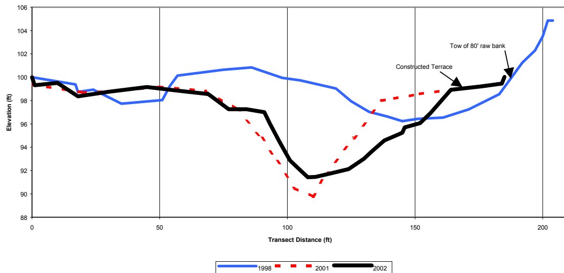
Figure 5. Cross section #1 within the Libby Creek Demonstration Project, surveyed before (1998) and after (2001 & 2002) project construction. This site is located 277 feet below the upper boundary of the project area. Note the constructed terrace that relocated Libby Creek away from an 80 feet high eroding bank that was contributing coarse and fine sediment to Libby Creek during each high flow event.
