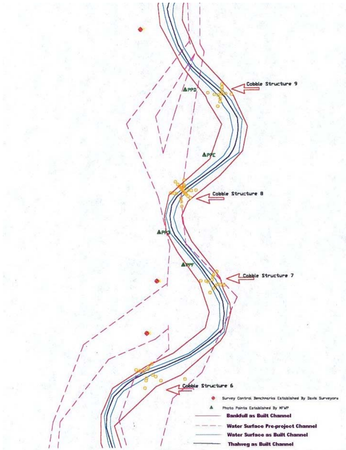
Figure A1 (continued). Plan view of the existing stream channel and constructed stream channel for the Libby Creek Cleveland Restoration Project beginning at approximately station 800 (upper portion of figure) proceeding upstream approximately to station 1600 (lower portion of figure).
