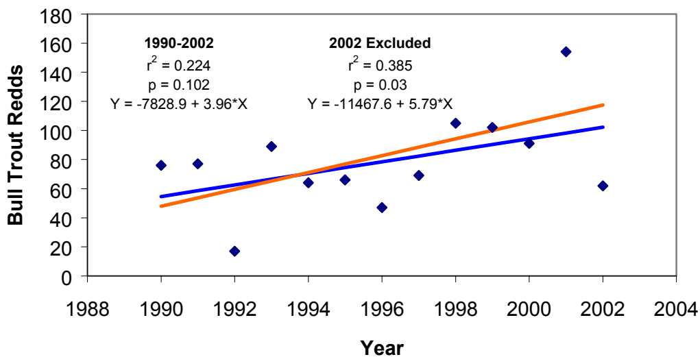
Figure 4. Bull trout redd counts and trend analysis (blue line) for Quartz Creek (including West Fork Quartz) 1990-2002. The 2002 observation was removed and the regression analysis repeated due to the presence of a log jam in the West Fork Quartz Creek in 2002 (orange line).
