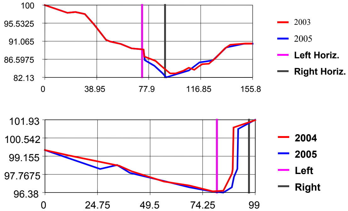
Figure 4. Cross sections 4 and 5B (top to bottom, respectively) on the Libby Creek Demonstration Project.
