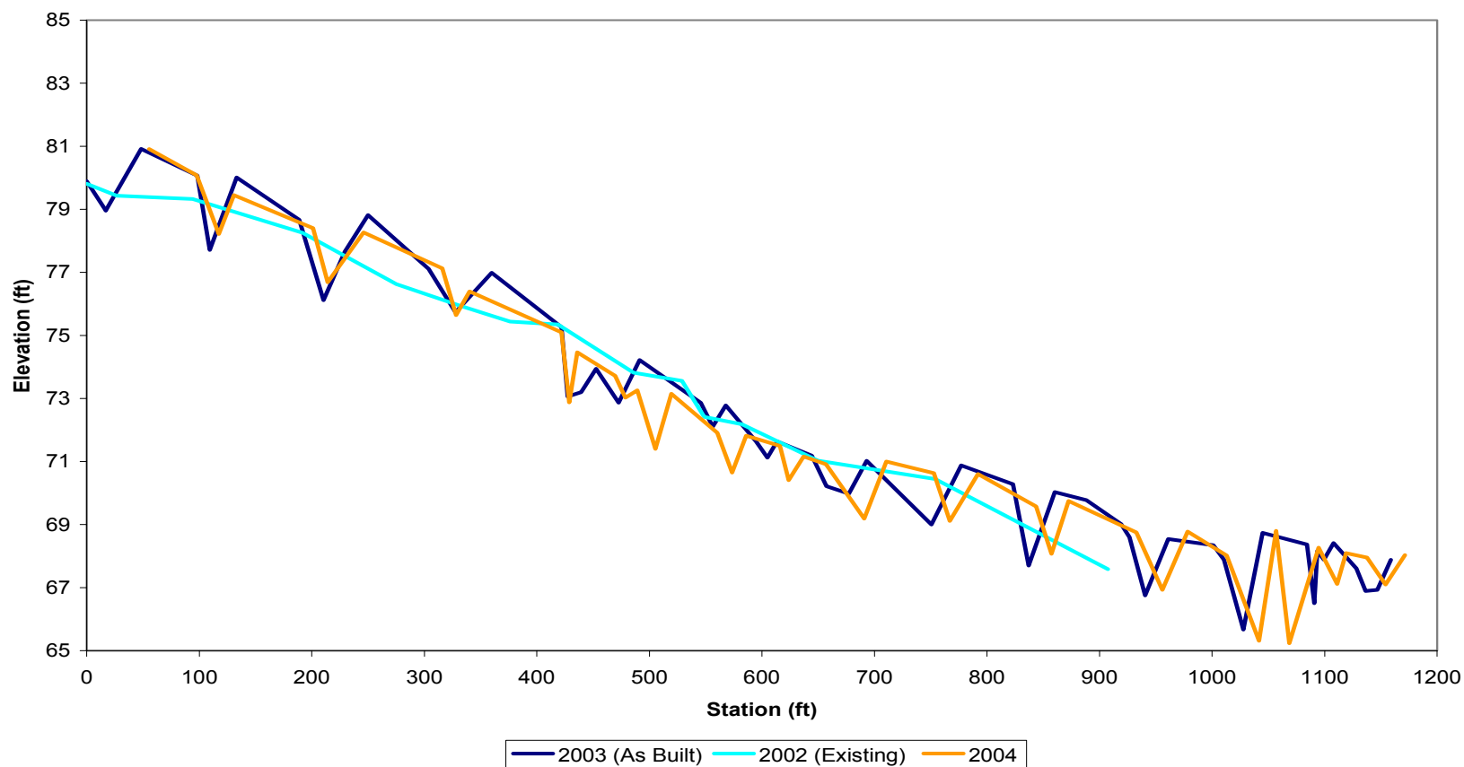
Figure 2. The longitudinal profile of the reach of Young Creek located within the State Lands Restoration Project. The survey was completed in (2002; existing), 2003 (as built) and 2004. The station (longitudinal location measured at the channel thalweg) begins at the upstream boundary of the project. The existing stream channel was approximately 250 feet shorter due to the less meander frequency that existed prior to the restoration activities.
