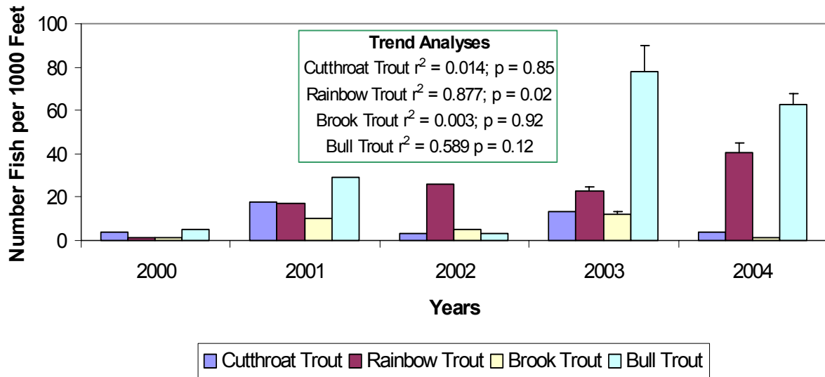
Figure 25. Cutthroat, rainbow, brook, and bull trout abundance estimates (fish per 1000 feet) and linear regression trend analyses within the Grave Creek Demonstration Project monitoring site from 2000-2004 collected by backpack electrofishing. The 2000 and 2001 data were collected using single pass electrofishing, the data collected in 2002 was collected via snorkel counts, and the 2003 and 2004 data was collected using multiple pass electrofishing. Upper 95% confidence intervals are represented by the whisker bars.
