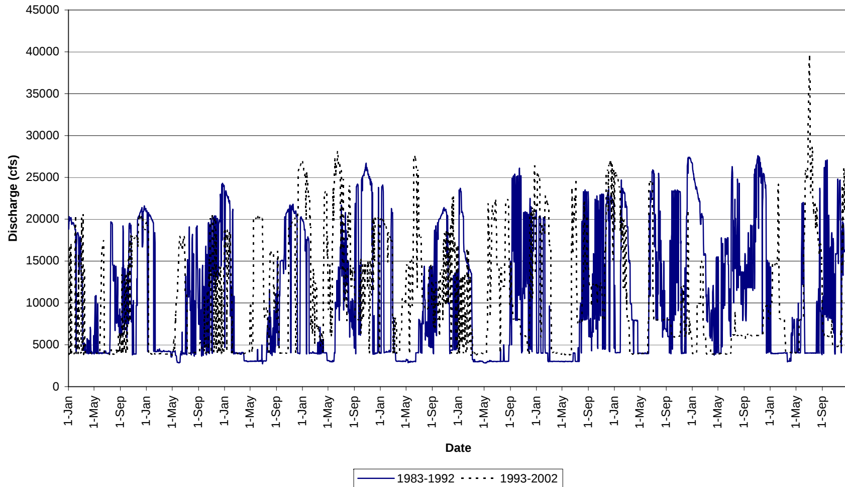
Figure 8. Ten year hydrograph comparing 1983-1992 data to 1993-2002 data.
