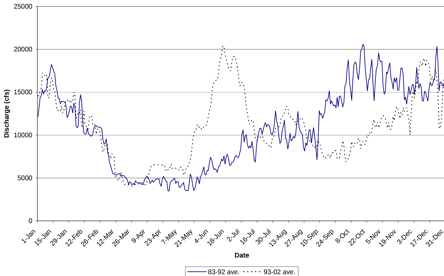
Figure 7. Average annual hydrograph comparing 1983-1992 data to 1993-2002 data.
