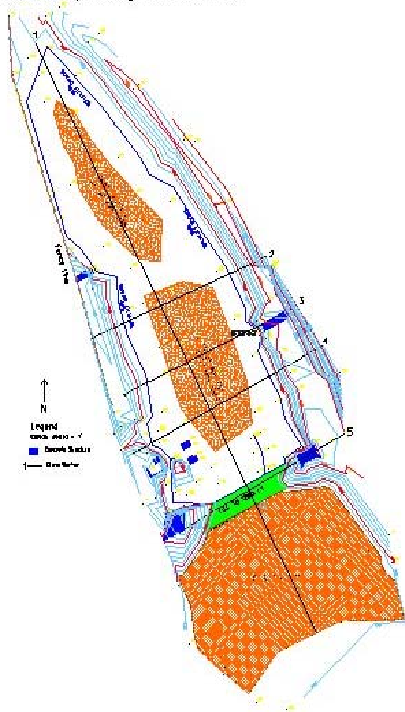
Proposed Troy Fishing Pond Plan View
