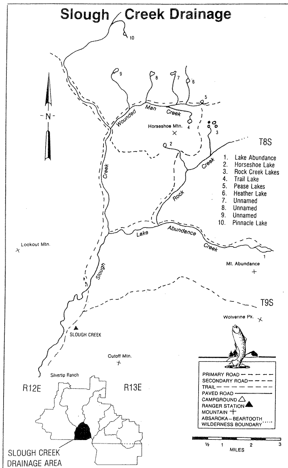
Figure 1. Location of lakes in the Slough Creek Drainage.
