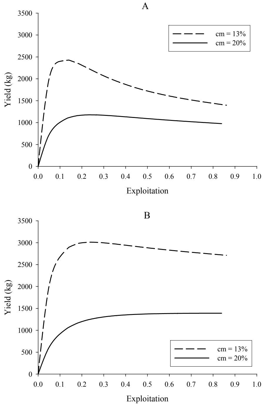
Figure 16. Simulated yields for the lake trout population in Lake McDonald, Glacier National Park with conditional natural mortality (cm) rates of 13% and 20%. Yield was simulated for minimum effective capture sizes of 250 mm total length (A) and 373 mm total length (B).
