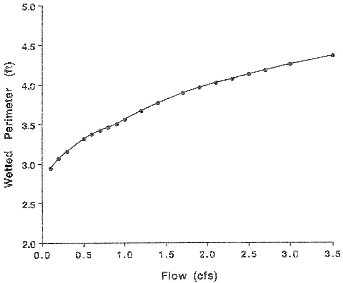
Figure 2-31. The relationship between wetted perimeter and flow for a composite of three riffle cross-sections in the West Fork of Dyce Creek.
