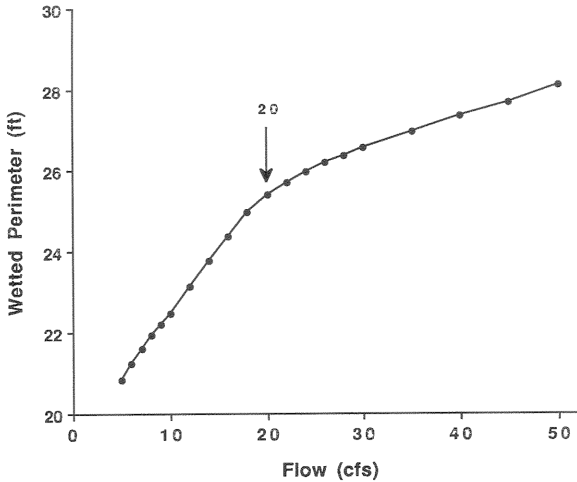
Figure 2-25. The relationship between wetted perimeter and flow for a single riffle cross-section in Bloody Dick Creek.
