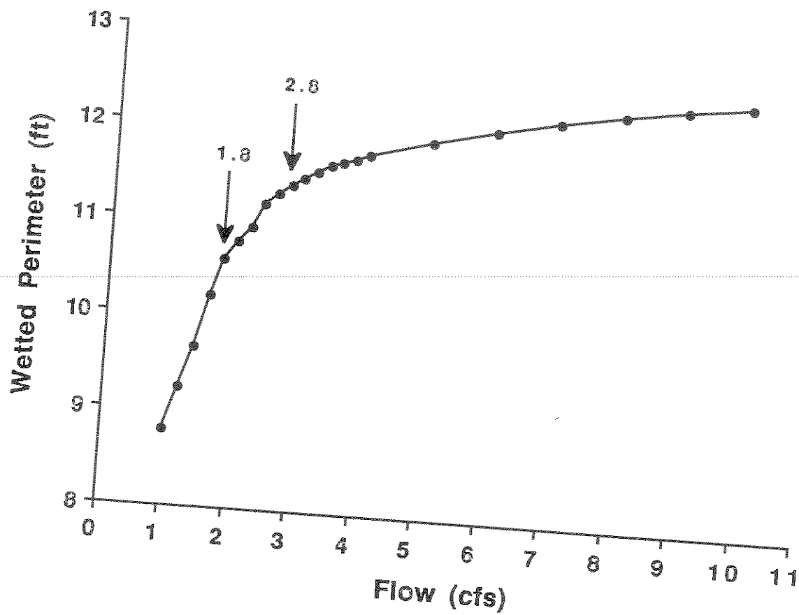
Figure 2-77. The relationship between wetted perimeter and flow for a composite of four riffle cross-sections in American Creek.
