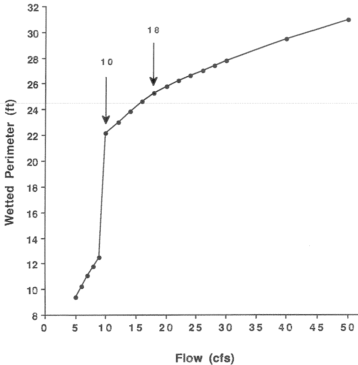
Figure 2-80. The relationship between wetted perimeter and flow for a single riffle cross-section in Deep Creek.
