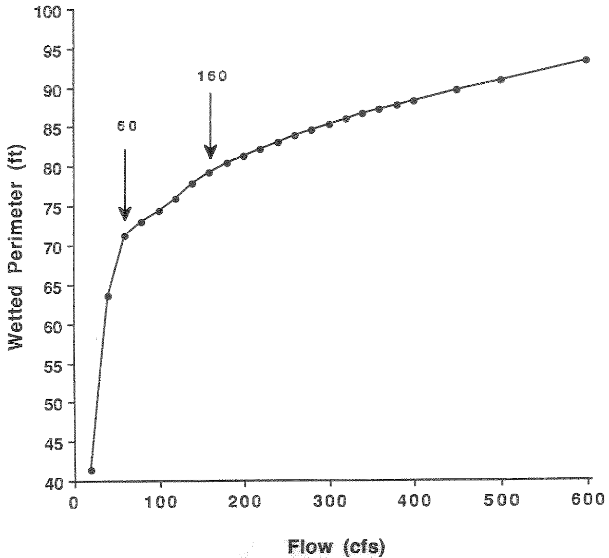
Figure 2-50. The relationship between wetted perimeter and flow for a composite of four riffle cross-sections in Reach #1 of the Big Hole River.
