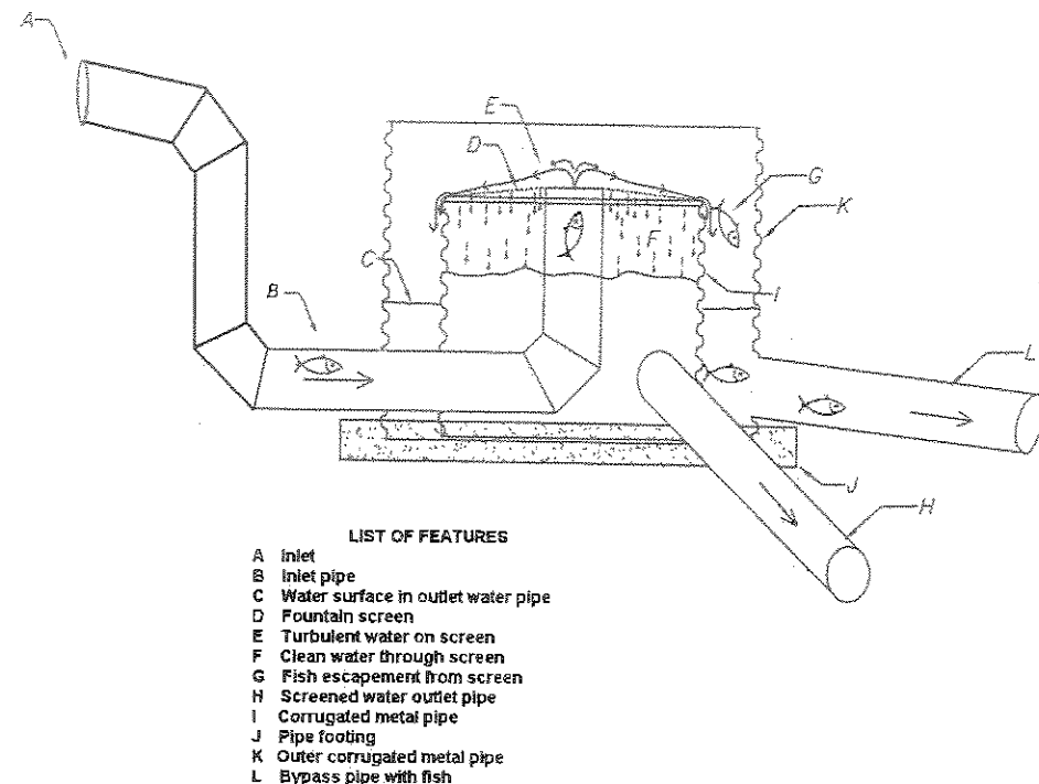
Figure 1. Conceptual design of a turbulent fountain fish screen with bypass to stream.
