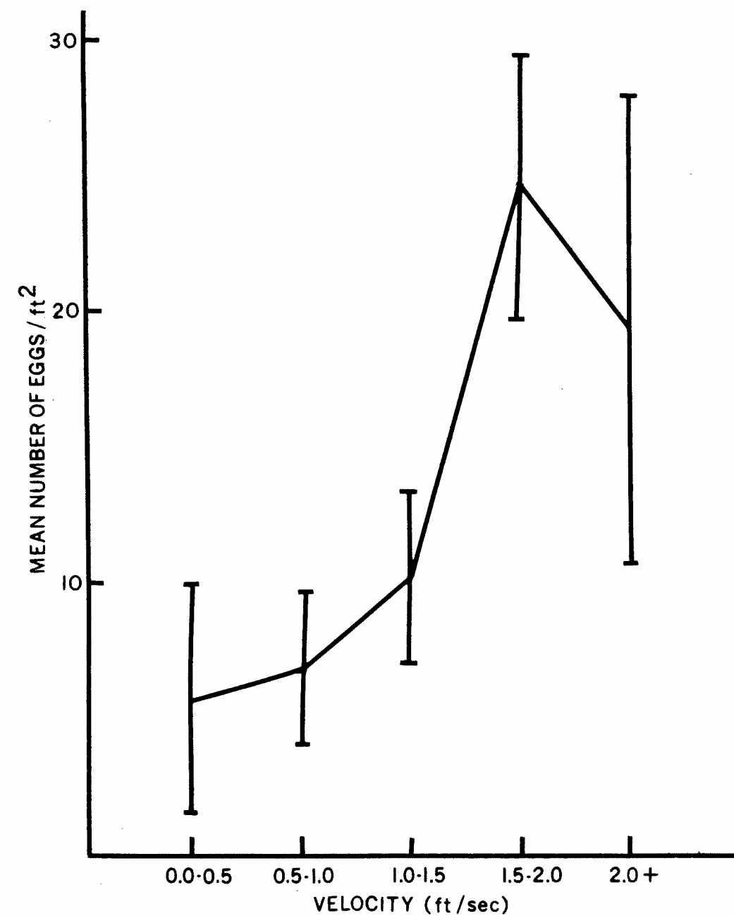
Figure 6. Mean number of eggs recovered and 95% confidence intervals with respect to velocity, Logan River, 1971.
