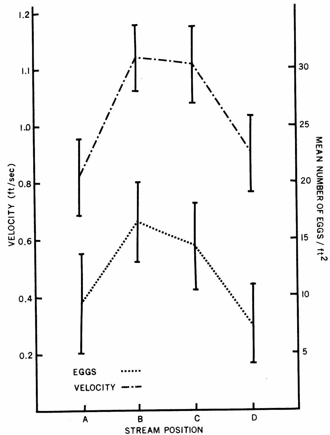
Figure 5. Mean velocities and mean number of eggs recovered from Logan River, 1971 including 95% confidence intervals with respect to stream position.
