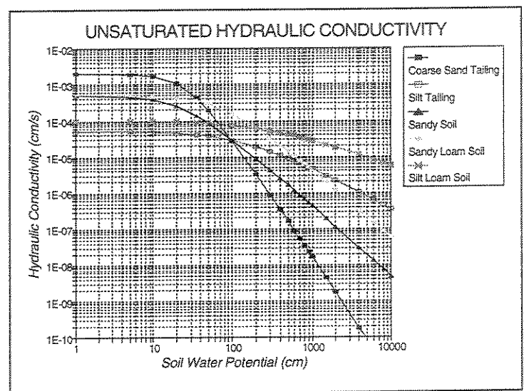
Figure 2. Unsaturated hydraulic conductivity curves for type soils 1 through 5 for the STARS investigation.
