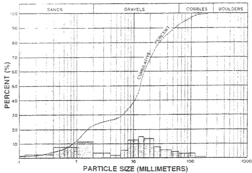
Fig. 7. Channel material sizes showing cumulative and percent distributions.
