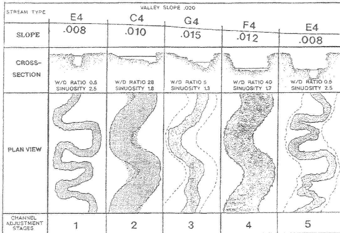
Fig. 9. Evolutionary stages of channel adjustment.
