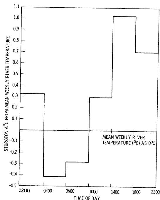
FIGURE 2.—Mean sturgeon environmental temperature deviation ( \Delta^\circ\text{C} ) from mean weekly Columbia River temperatures averaged over 4-h periods within the diel cycle, from 19 June through 20 August 1977.
