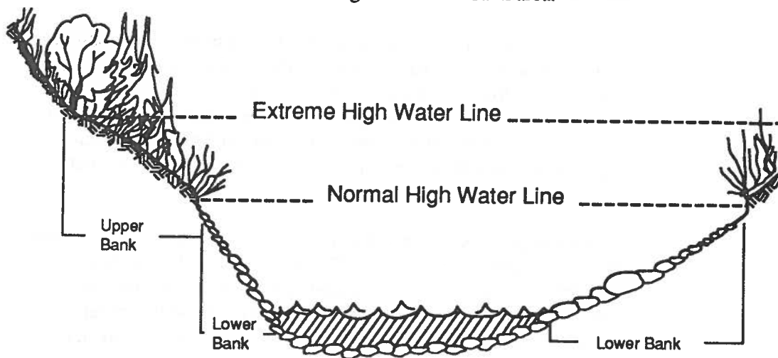
Figure 9. Upper streambank area from Pfankuch (1975).
