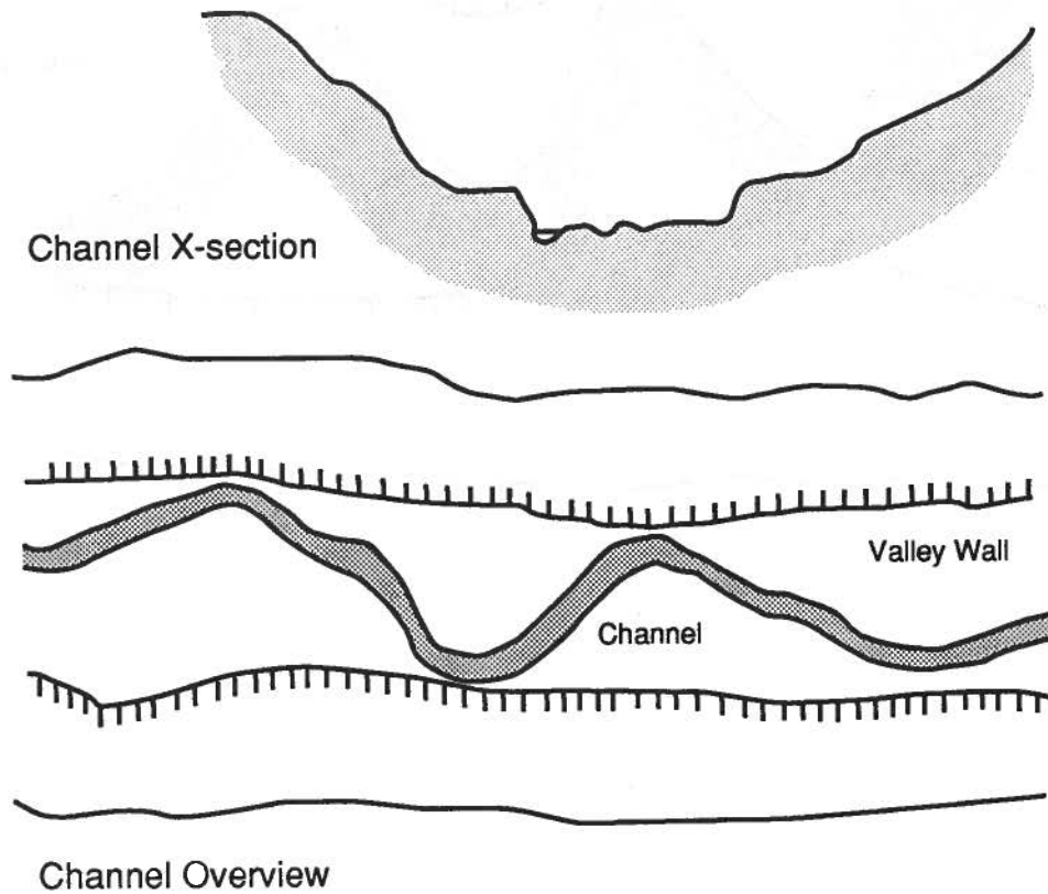
Figure 5. Occasionally and frequently confined channels.
