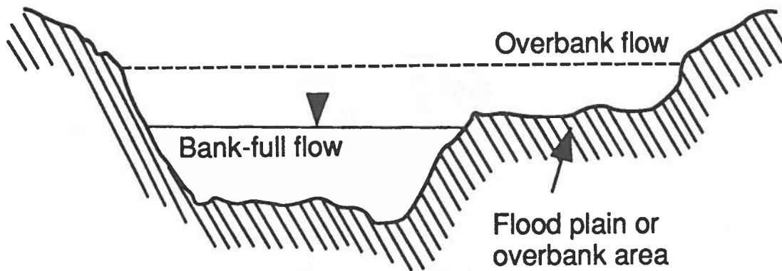
Figure 10. Stream channel cross-section showing approximate stages for bankfull and overbank flows.
