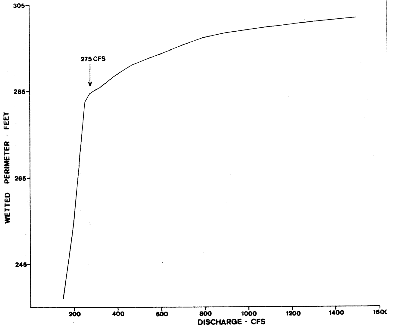
Appendix D6. Wetted perimeter-discharge relationship for a composite of 3 cross sections of a riffle near the Lee Metcalf Wildlife Refuge.
