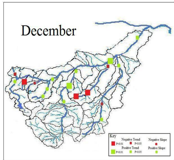
Figure 2.8m Trend analyses of average monthly discharge for December in the YRB.
