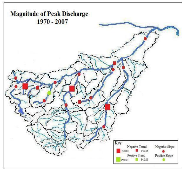
Figure 2.5 Trend analyses for magnitude of peak discharge in the YRB from 1970 to 2007.
