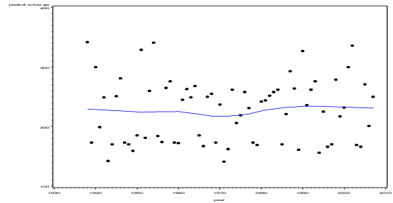
Figures 64-80: Annual Peak Discharge
