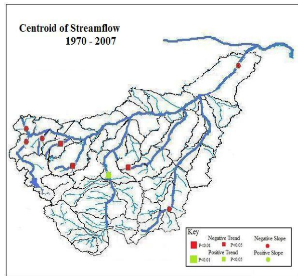
Figure 2.10 Trend analyses for centertime measurement from 1970 to 2007 in the YRB.
