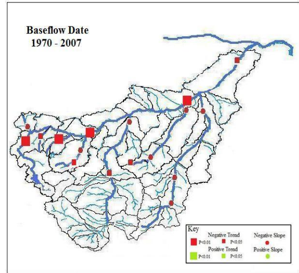
Figure 2.14 Trend analyses for date of return baseflow from 1970 to 2007 in the YRB.
