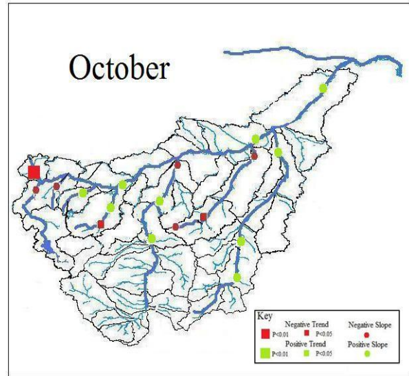
Figure 2.8j Trend analyses of average monthly discharges for October in the YRB.
