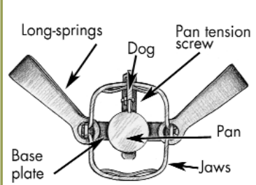
Figure BV9. Double jaw double-longspring trap (open)
