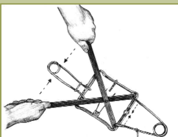
Figure BV4b. Using setting tool
