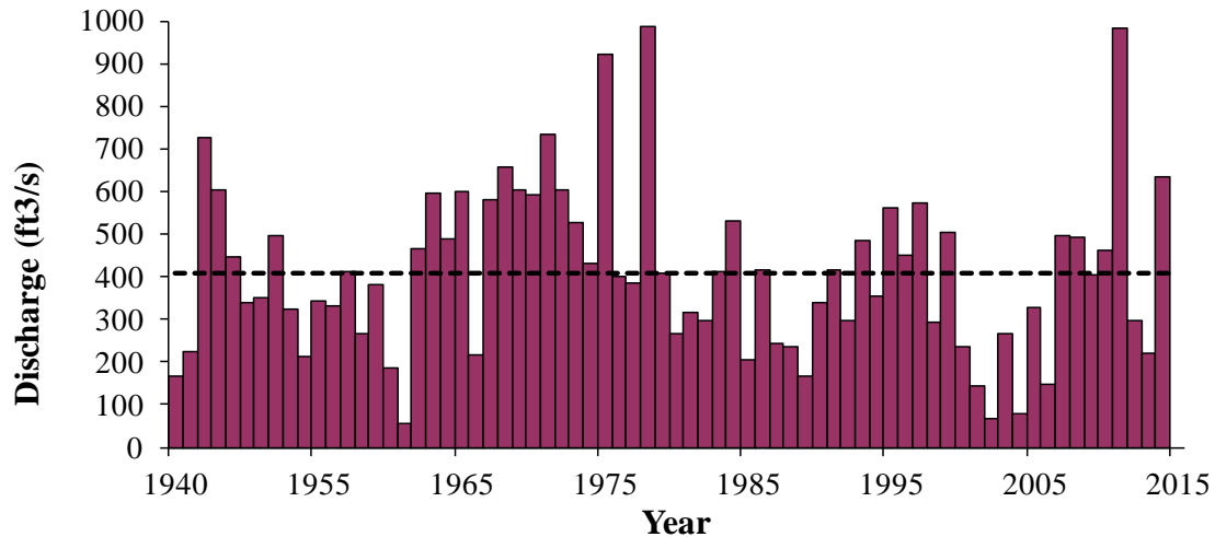
Figure 2. - Mean annual discharge of the Tongue River at Miles City, 1940-2015. Dashed line represents overall mean annual discharge for the period of record.
