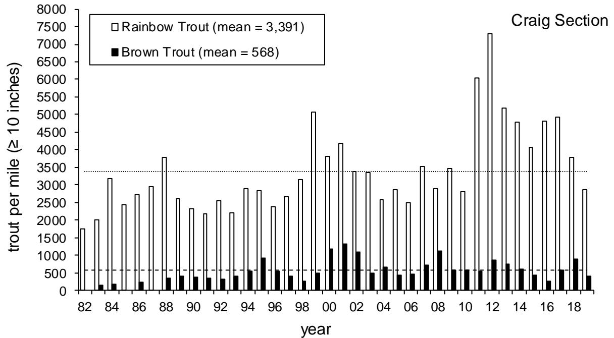
Figure 1. Population estimates of Rainbow Trout and Brown Trout 10 inches and greater per mile in the Missouri River, Montana within the Craig sampling section from 1982 through 2019. Long-term average number of Rainbow Trout and Brown Trout per mile are designated by horizontal lines and 2019 estimates were 2,860 and 390, respectively.
