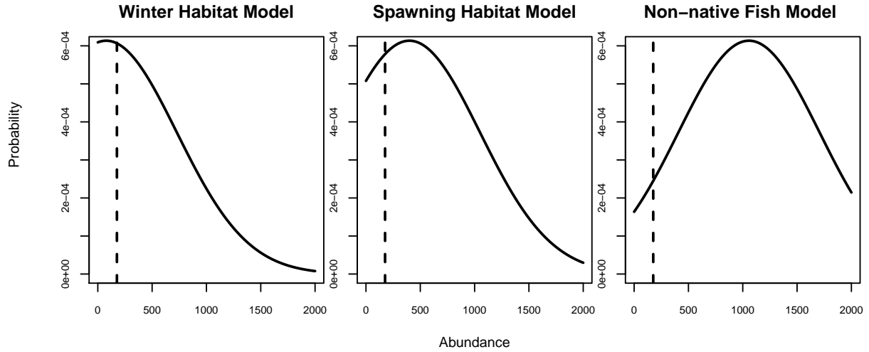
Figure 8. Normal probability density plots for Winter Habitat , Spawning Habitat , and Non-native Fish models with \mu = 78, 400 , and 1057 , respectively. Standard deviation for all plots = 650 . Vertical dashed lines show the observed grayling spawning population, \hat{N} = 176 , in 2017.
