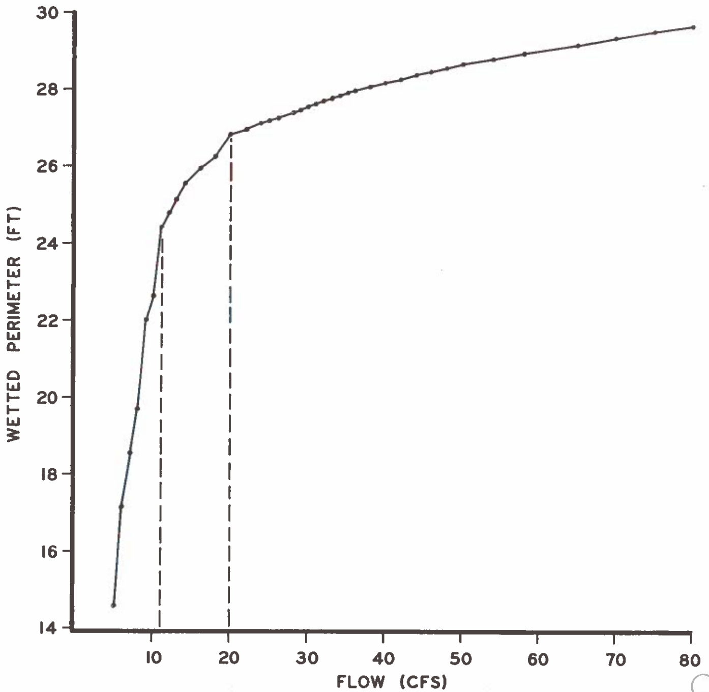
Figure 44. The relationship between wetted perimeter and flow for a composite of two riffle cross-sections in Cabin Creek.
