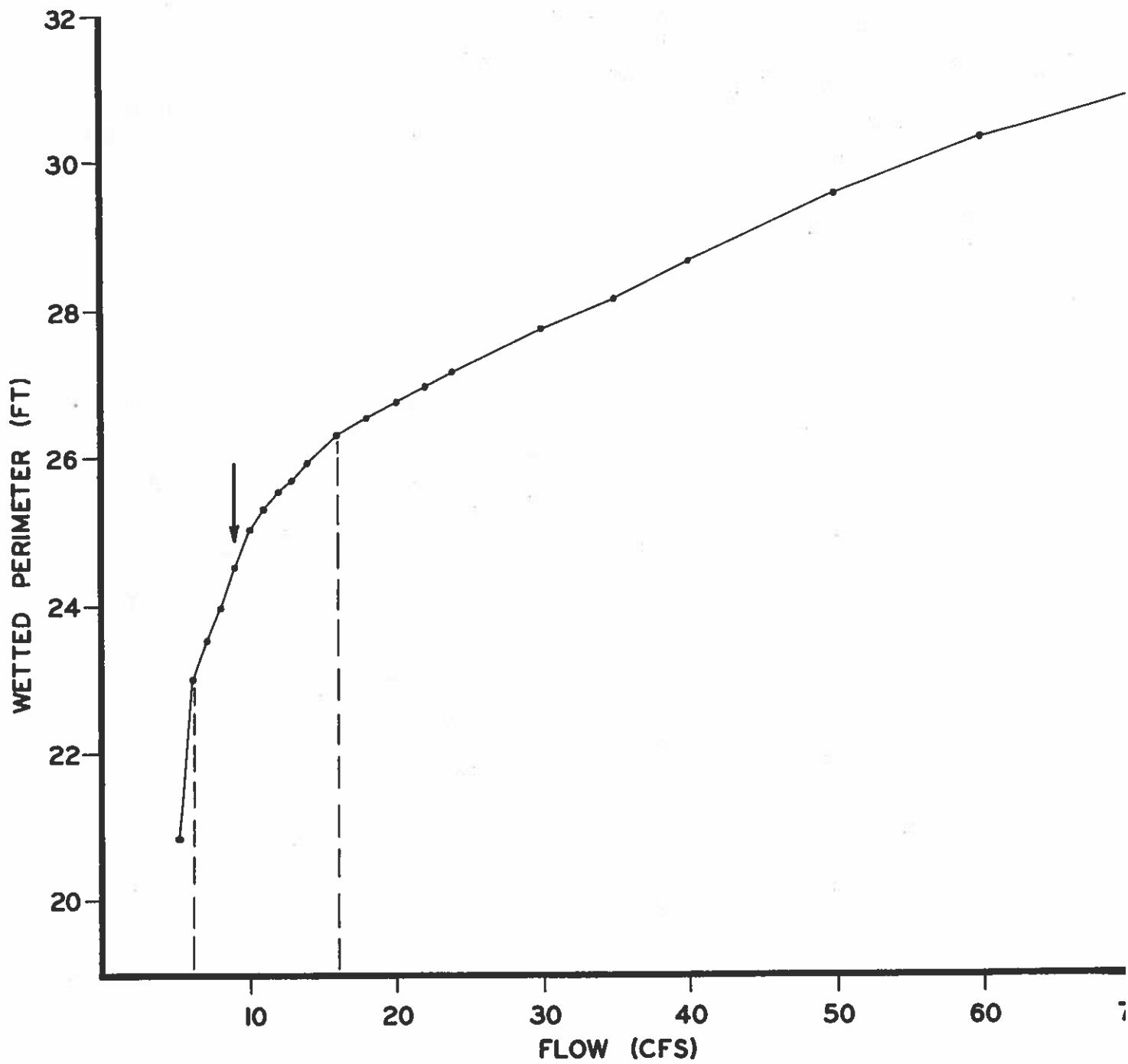
Figure 61. The relationship between wetted perimeter and flow for a composite of two riffle cross-sections in the Middle Fork Ruby River.
