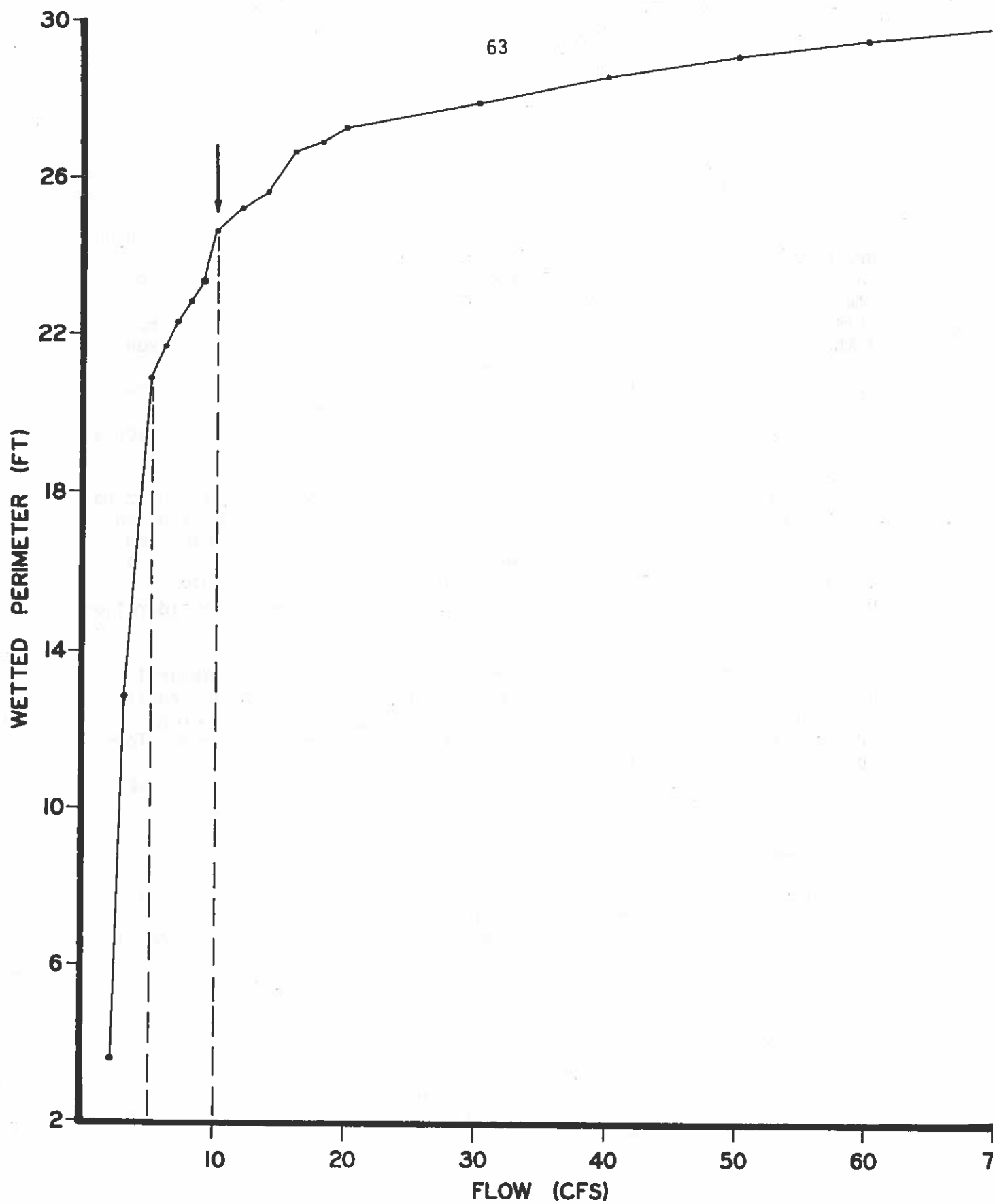
Figure 13. The relationship between wetted perimeter and flow for a composite of two riffle cross-sections in Fishtrap Creek.
