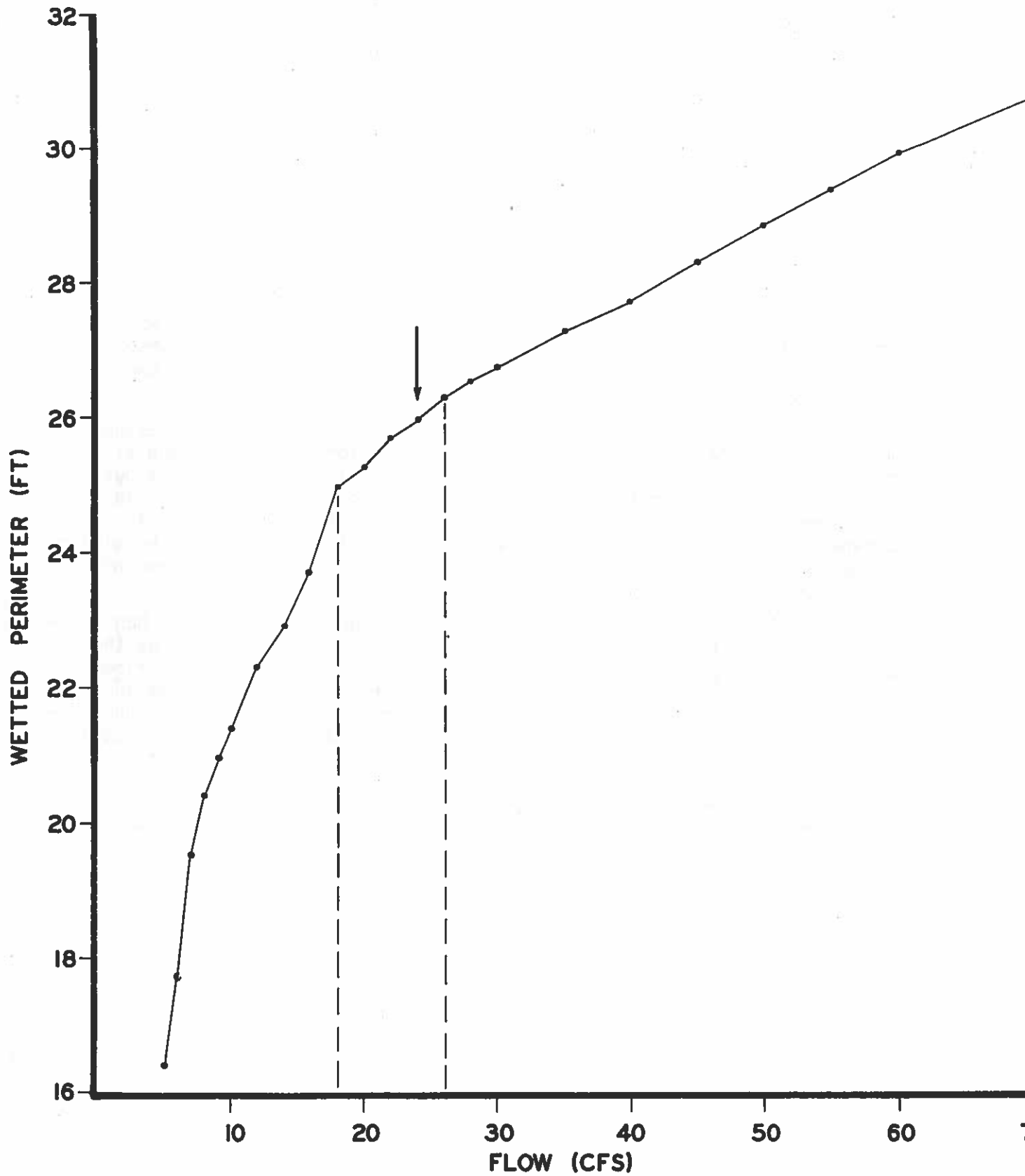
Figure 5. The relationship between wetted perimeter and flow for a single riffle cross-section in Bloody Dick Creek.
