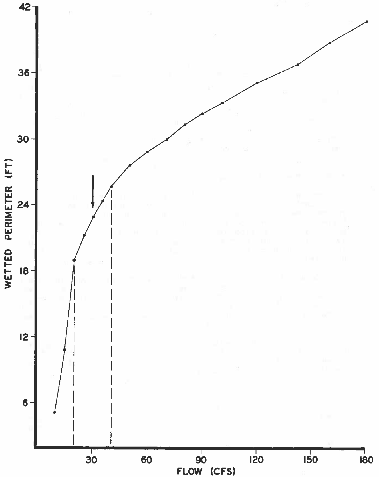
Figure 12. The relationship between wetted perimeter and flow for a composite of two riffle cross-sections in Deep Creek.
