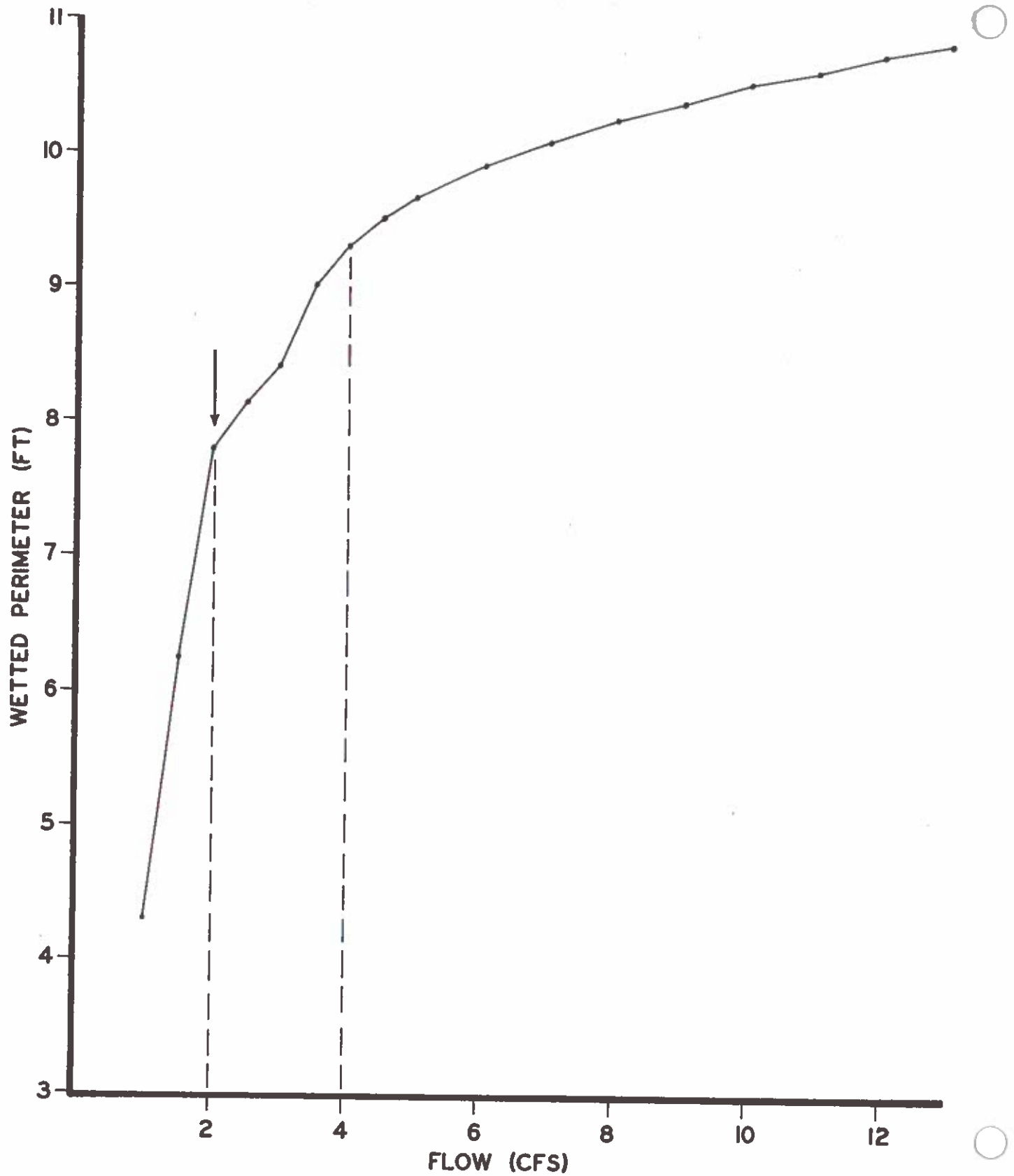
Figure 9. The relationship between wetted perimeter and flow for a composite of two riffle cross-sections in West Creek.
