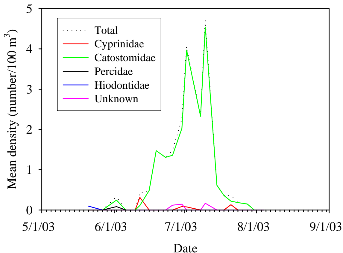
Figure 15. Mean density (number/100 m 3 ) by date of all larval fishes (Total), Catostomidae, Cyprinidae, Percidae, Hiodontidae, and unknown sampled in the Missouri River at the site downstream from Fort Peck Dam during 2003.
