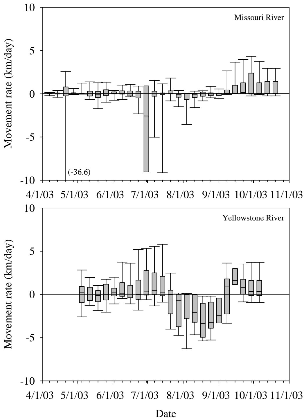
Figure 14. Box and whisker plots of net movement rates (km/day) of shovelnose sturgeon in the Missouri River and Yellowstone River during 2003. Median movement rate is denoted as a line within the box. The box delimits 25 th and 75 th percentiles of the data, and whiskers delimit the 5 th and 95 th percentiles.
