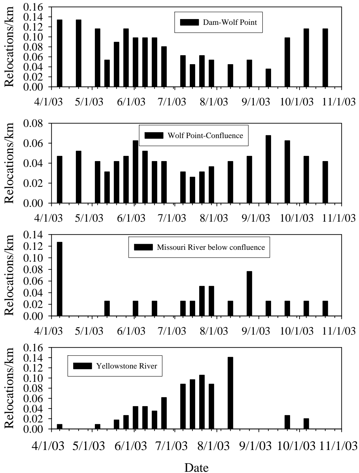
Figure 9. Number of blue sucker relocations per km in reaches of the Missouri River and Yellowstone River during 2003.
