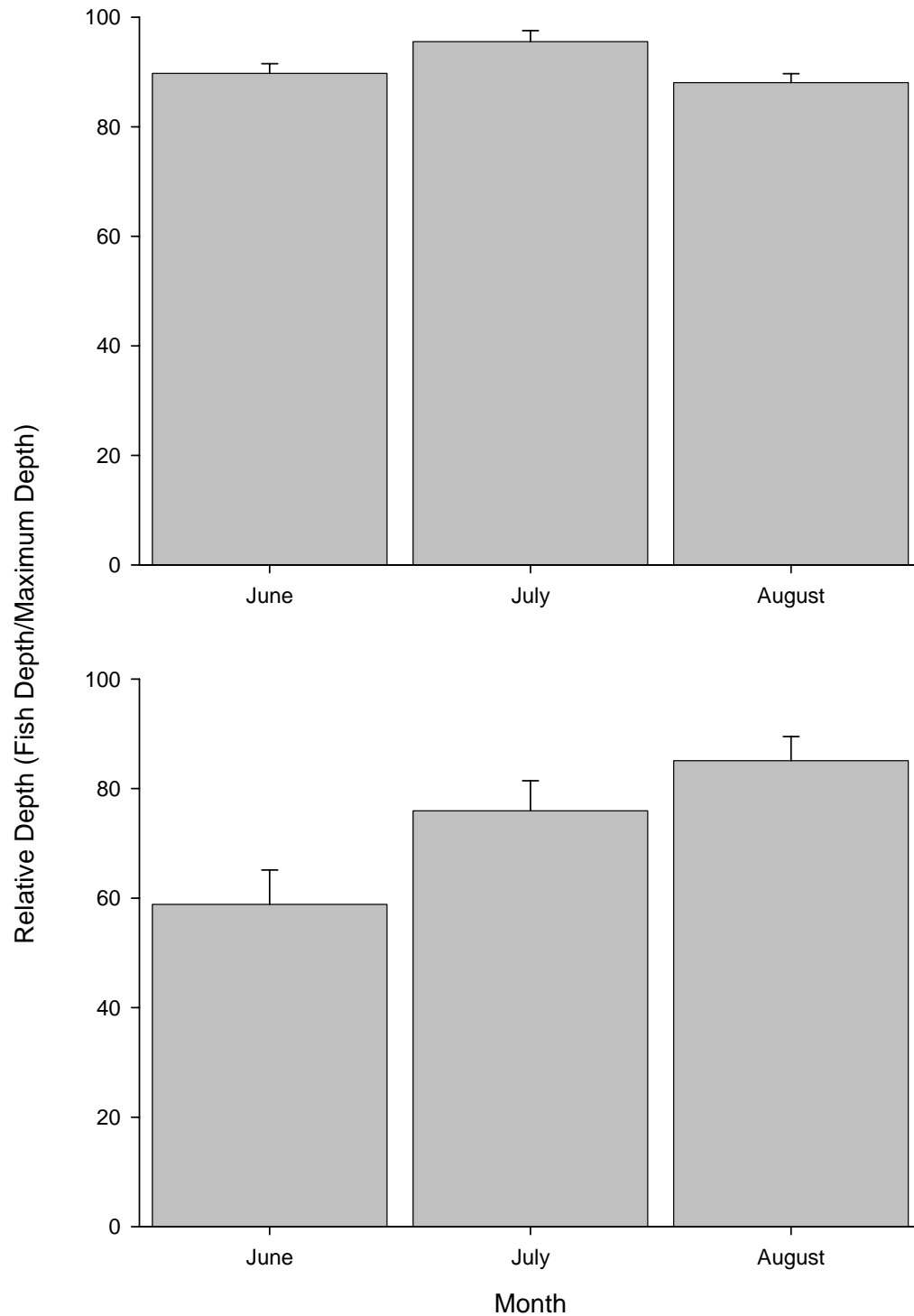
Figure 2. - Mean relative depth by month for HRJPS recorded from longitudinal profiles (top) and cross section profiles (bottom).
