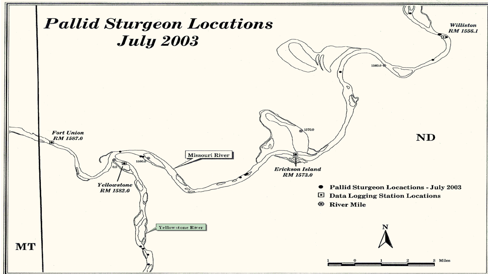
Figure 5. Locations of all pallids in July.
