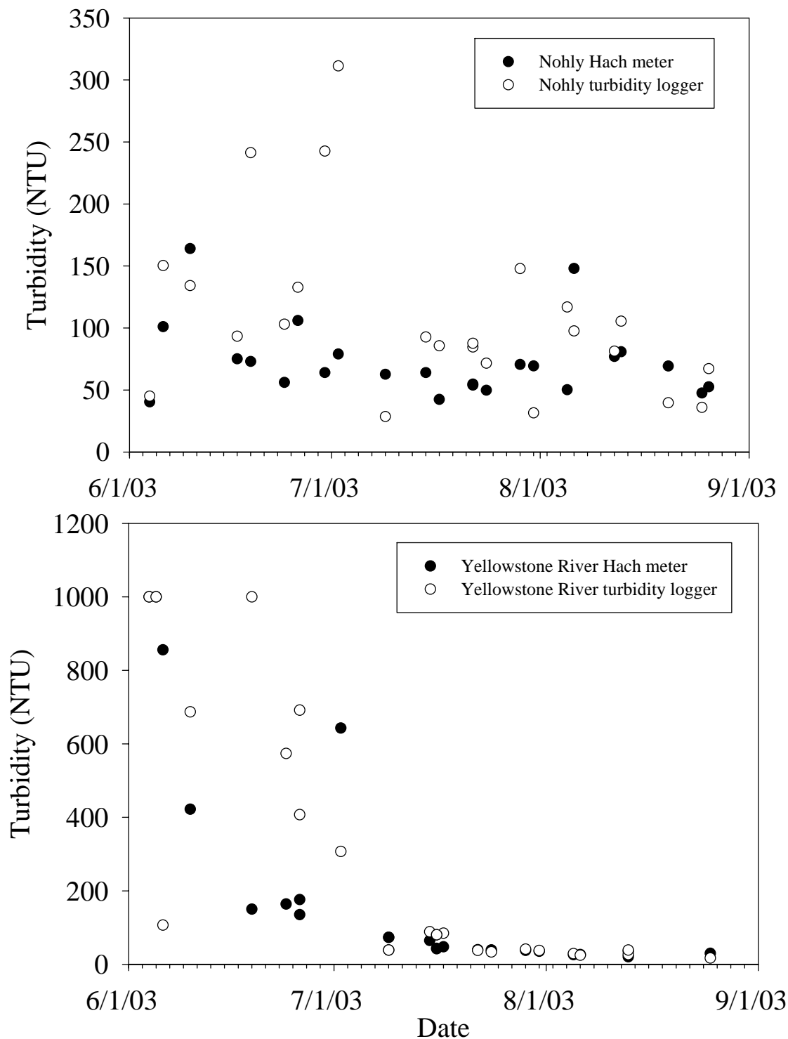
Figure 7. Hour-specific instantaneous turbidities (NTU) by date measured with a Hach meter during sampling activities and turbidity loggers at Nohly (upper panel) and in the Yellowstone River (lower panel).
