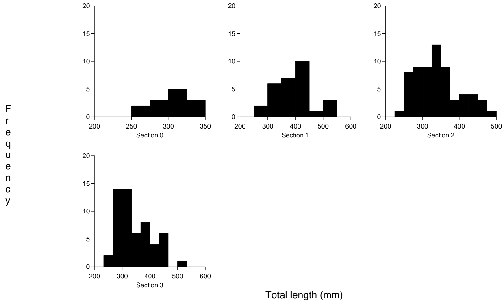
Figure 18. Total length-frequency plots by study section for sauger sampled during 2003.
