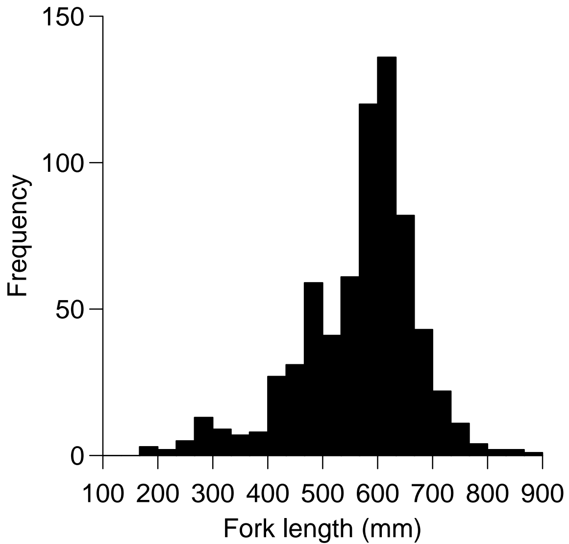
Figure 20. Fork length-frequency plot for shovelnose sturgeon captured in the study area during 2003.
