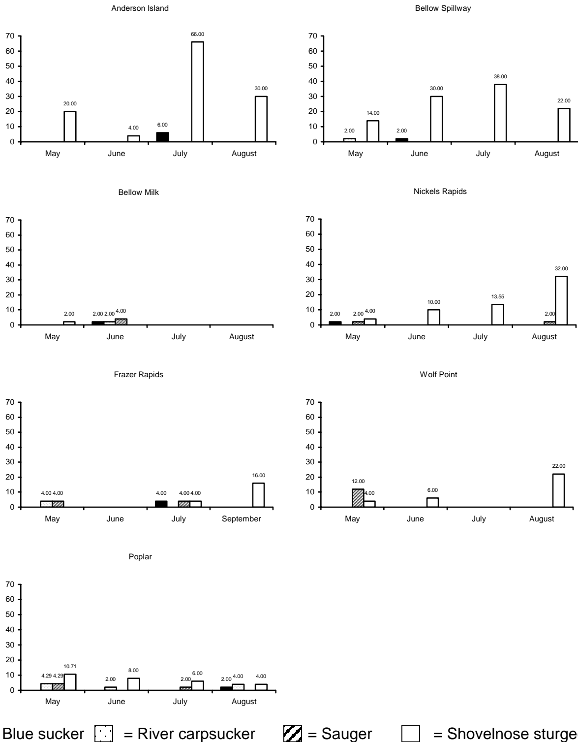
Figure 27. CPUE rates (number per hour sample time) for blue sucker, river carpsucker, sauger, and shovelnose sturgeon sampled in 2.5 cm inner mesh drifted trammel nets at standardized sites on the Missouri River, MT, during 2003.
