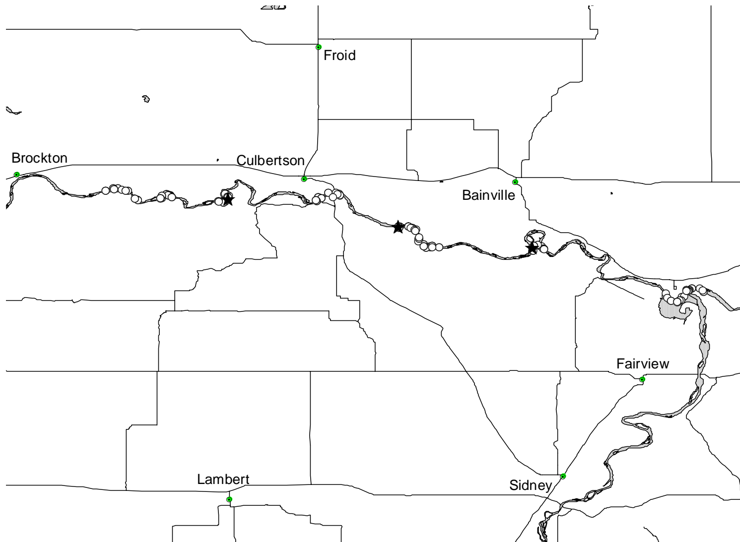
Figure 9. Sites sampled (white circles) with setlines and recapture sites (black stars) of hatchery-reared pallid sturgeon from near Brockton, MT to near to near the confluence of the Missouri and Yellowstone rivers, ND during 2003.
