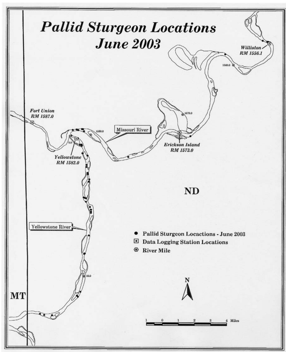
Figure 4. Locations of all pallids in June.
