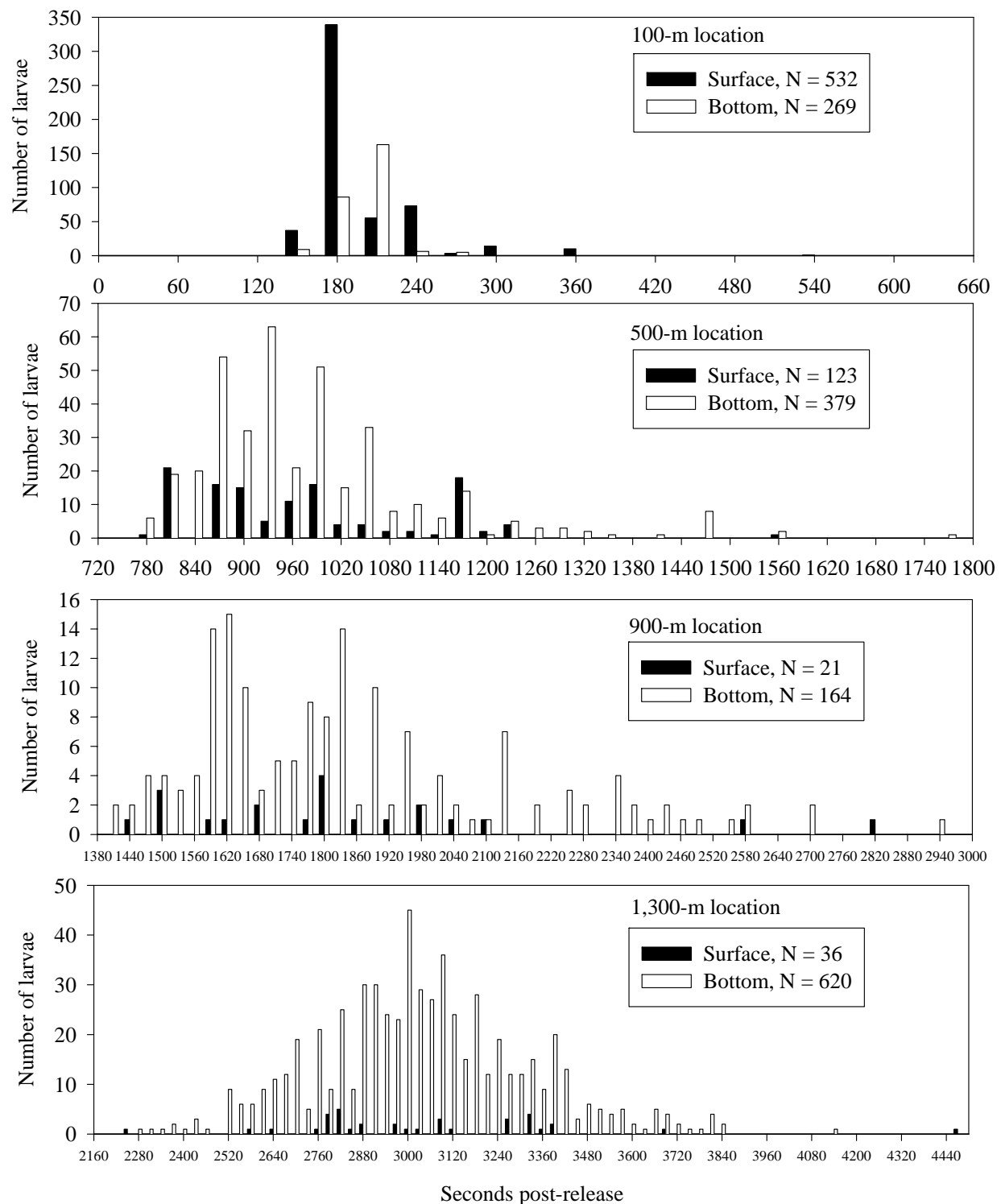
Figure 3. Number of larval shovelnose sturgeon sampled by time in surface and bottom nets at the 100-m, 500-m, 900-m, and 1,300-m sampling locations on June 25. Sampling continued for 900 sec, 1,800 sec, 3,600 sec, and 5,400 sec post-release for the increasing sampling location distances, respectively, but the abscissa is truncated.
