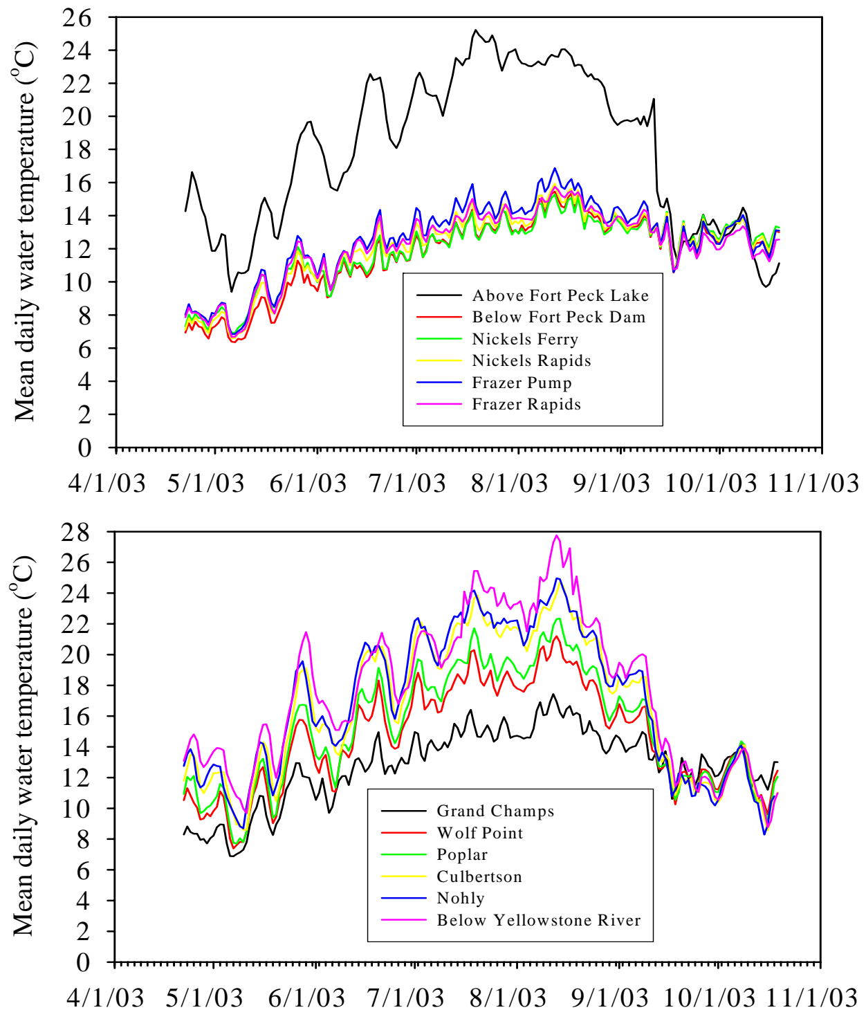
Figure 5. Mean daily water temperature (°C) at 12 sites on the mainstem Missouri River during 2003.
