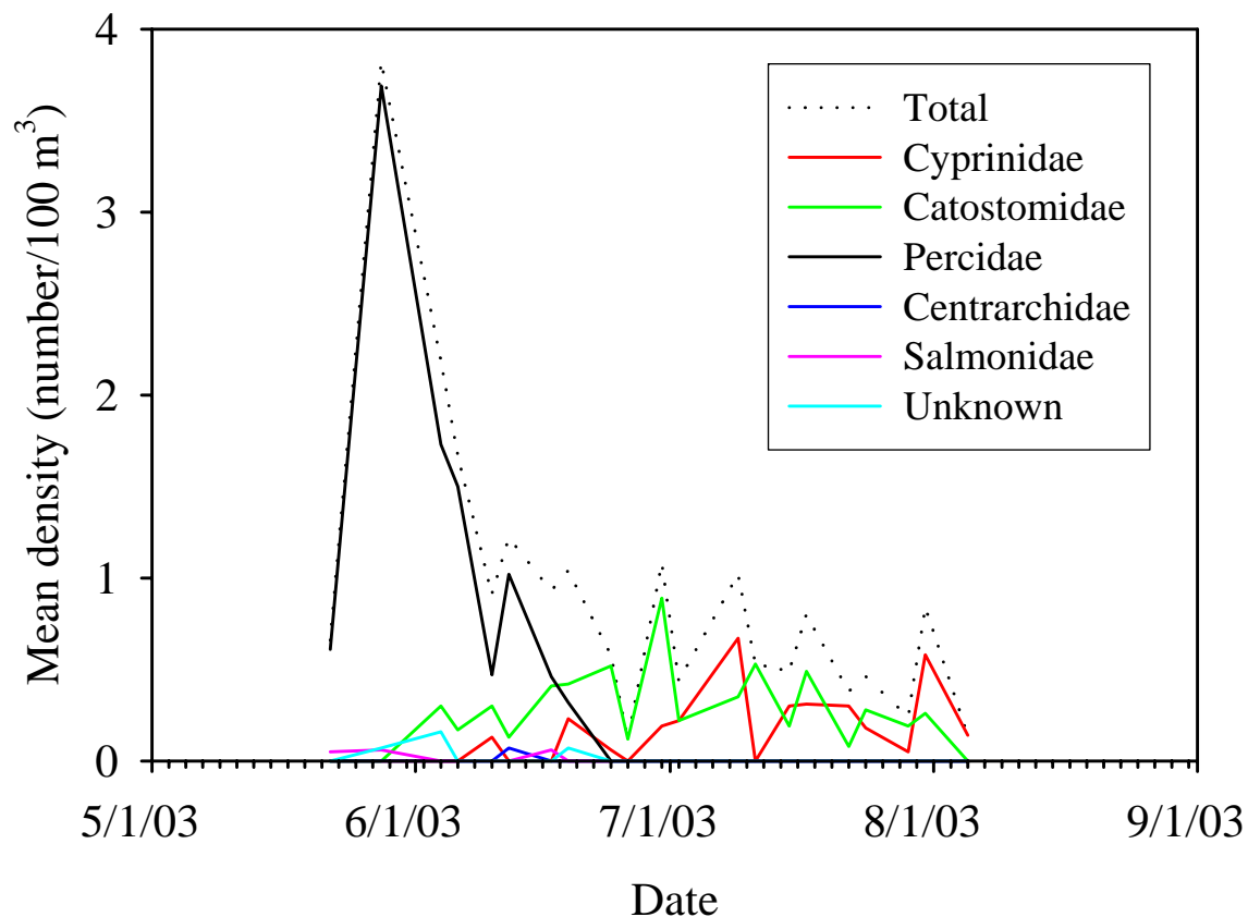
Figure 19. Mean density (number/100 m 3 ) by date of all larval fishes (Total), Catostomidae, Cyprinidae, Percidae, Salmonidae, Centrarchidae, and unknown sampled in the Missouri River near Nohly during 2003.
