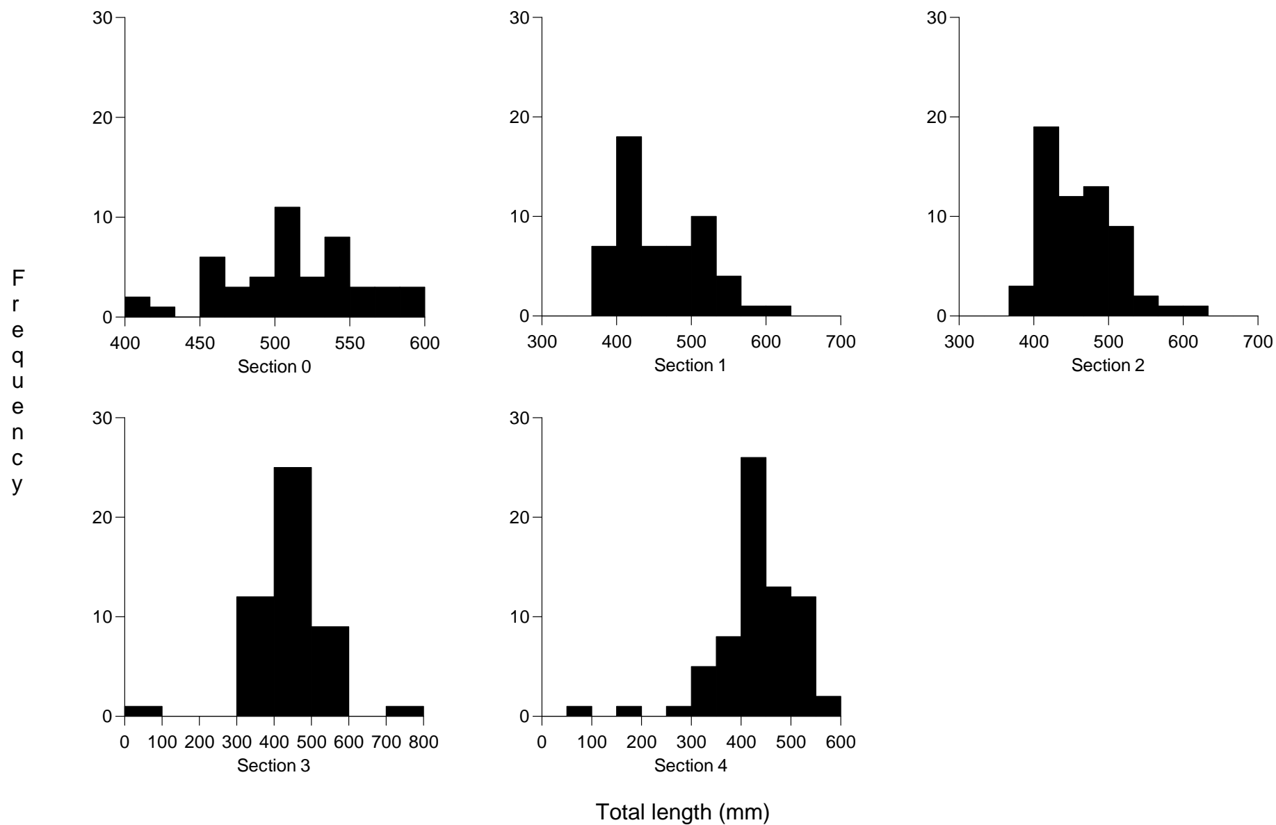
Figure 16. Total length-frequency plots by study section for river carpsuckers captured during 2003
