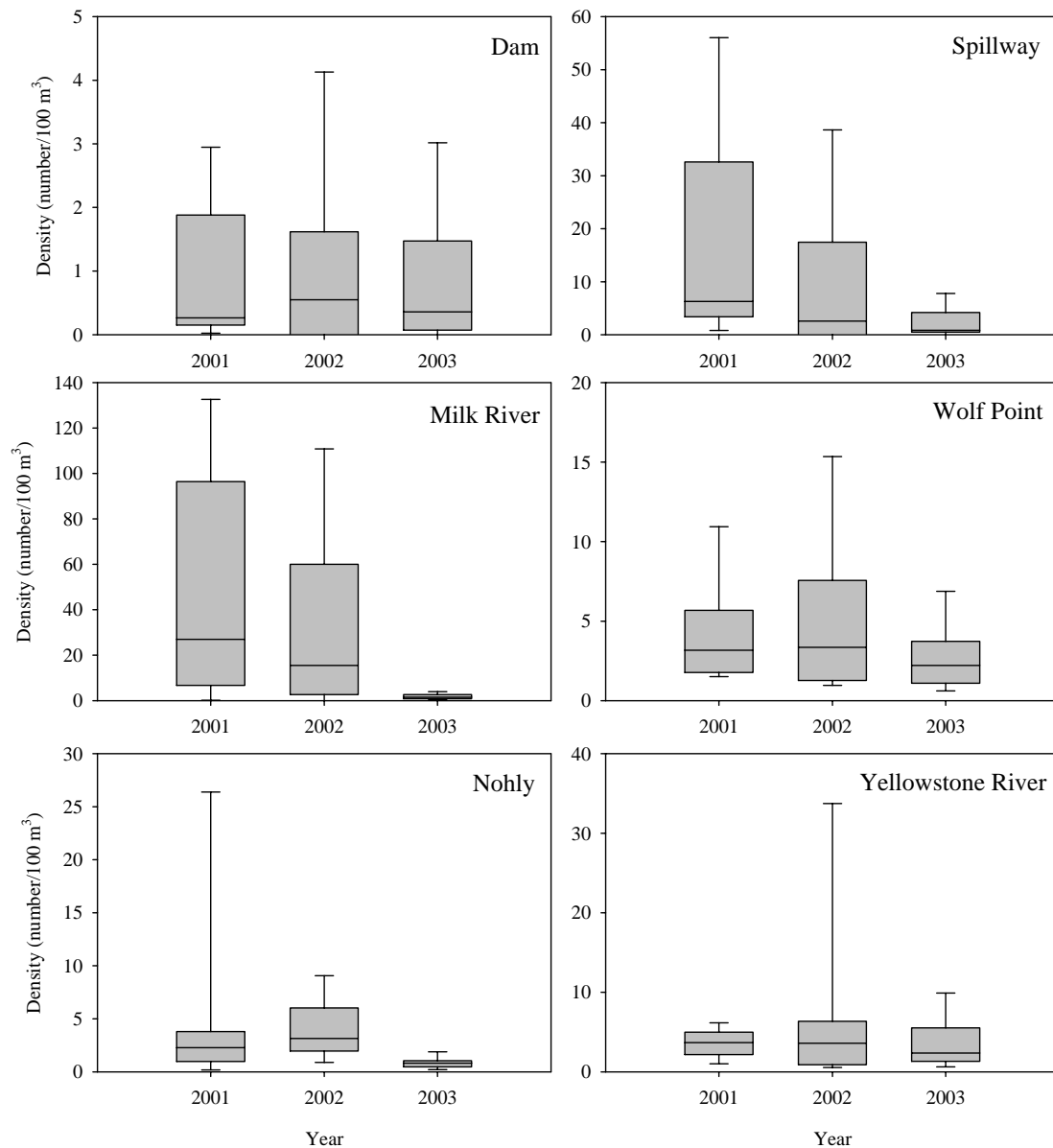
Figure 21. Box and whisker plots of total density (all taxa; number/100 m³) of larval fishes sampled at six sites in 2001, 2002, and 2003. Boxes delimit the 25 th and 75 th percentiles of the data, lines within the boxes denote median density, and whiskers delimit the 5 th and 95 th percentiles.
