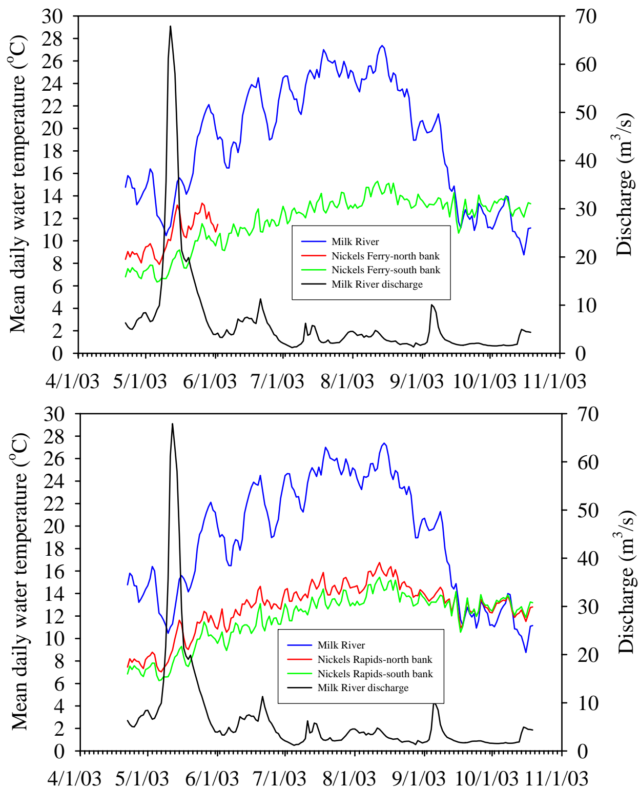
Figure 2. Water temperature profiles and discharge for the Milk River, and water temperatures profiles for the Missouri River at Nickels Ferry and Nickels Rapids during 2003.
