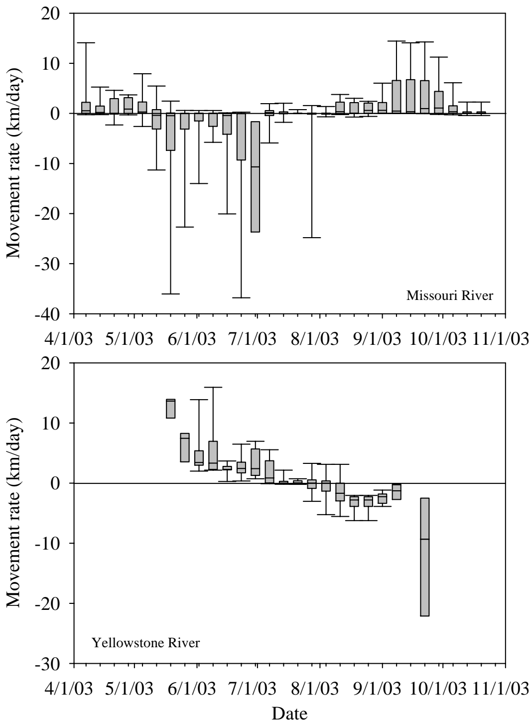
Figure 10. Box and whisker plots of net movement rates (km/day) of blue suckers in the Missouri River and Yellowstone River during 2003. Median movement rate is denoted as a line within the box. The box delimits 25 th and 75 th percentiles of the data, and whiskers delimit the 5 th and 95 th percentiles.
