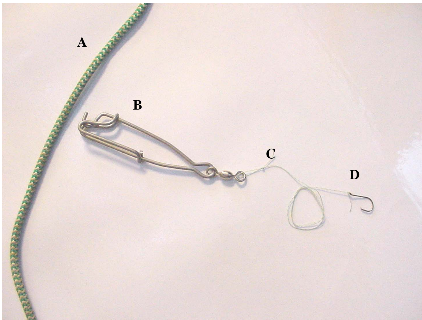
Figure 4. Digital image of setline components. (A) A section of main leaded line; (B) a trotline swivel clip; (C) an 45.72 cm, 9.072 kg test Dacron leader; (D) a circle hook.
