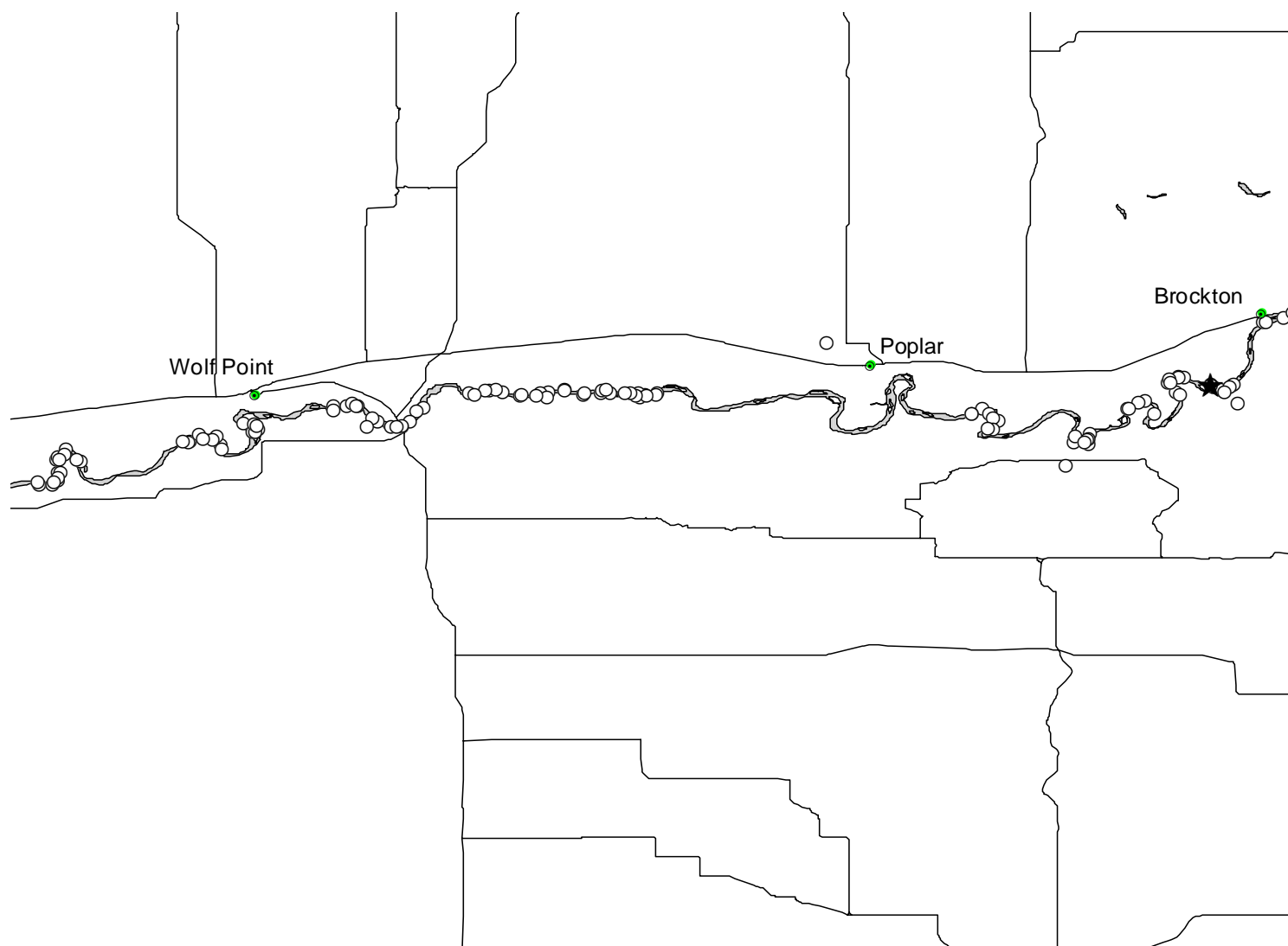
Figure 6. Sites sampled (white circles) with drifted trammel nets and recapture sites (black stars) of hatchery-reared pallid sturgeon in the Missouri River from near Oswego to near Brockton, MT during 2003.
