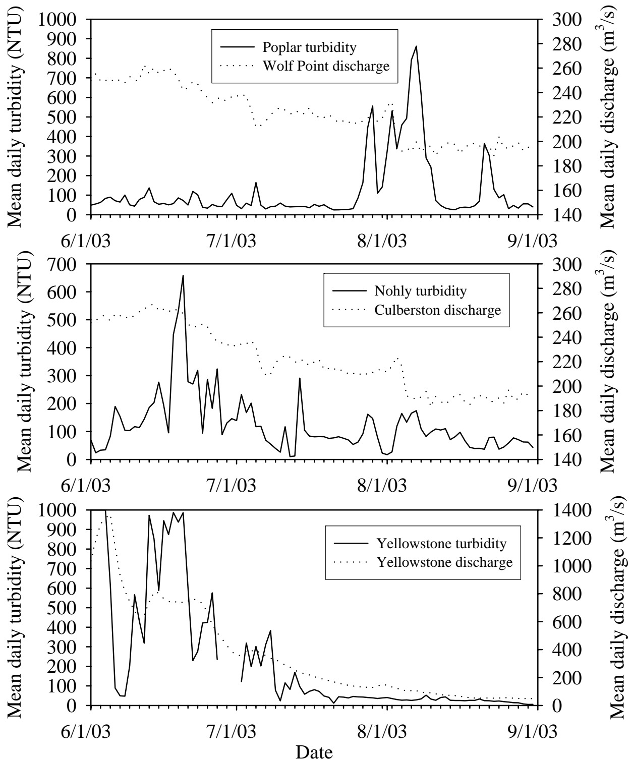
Figure 8. Mean daily turbidity (NTU; solid line) from turbidity loggers and discharge ( \text{m}^3/\text{s} ; dotted line) in the Missouri River near Poplar (upper panel), Nohly (middle panel), and in the Yellowstone River (lower panel) during 2003.
