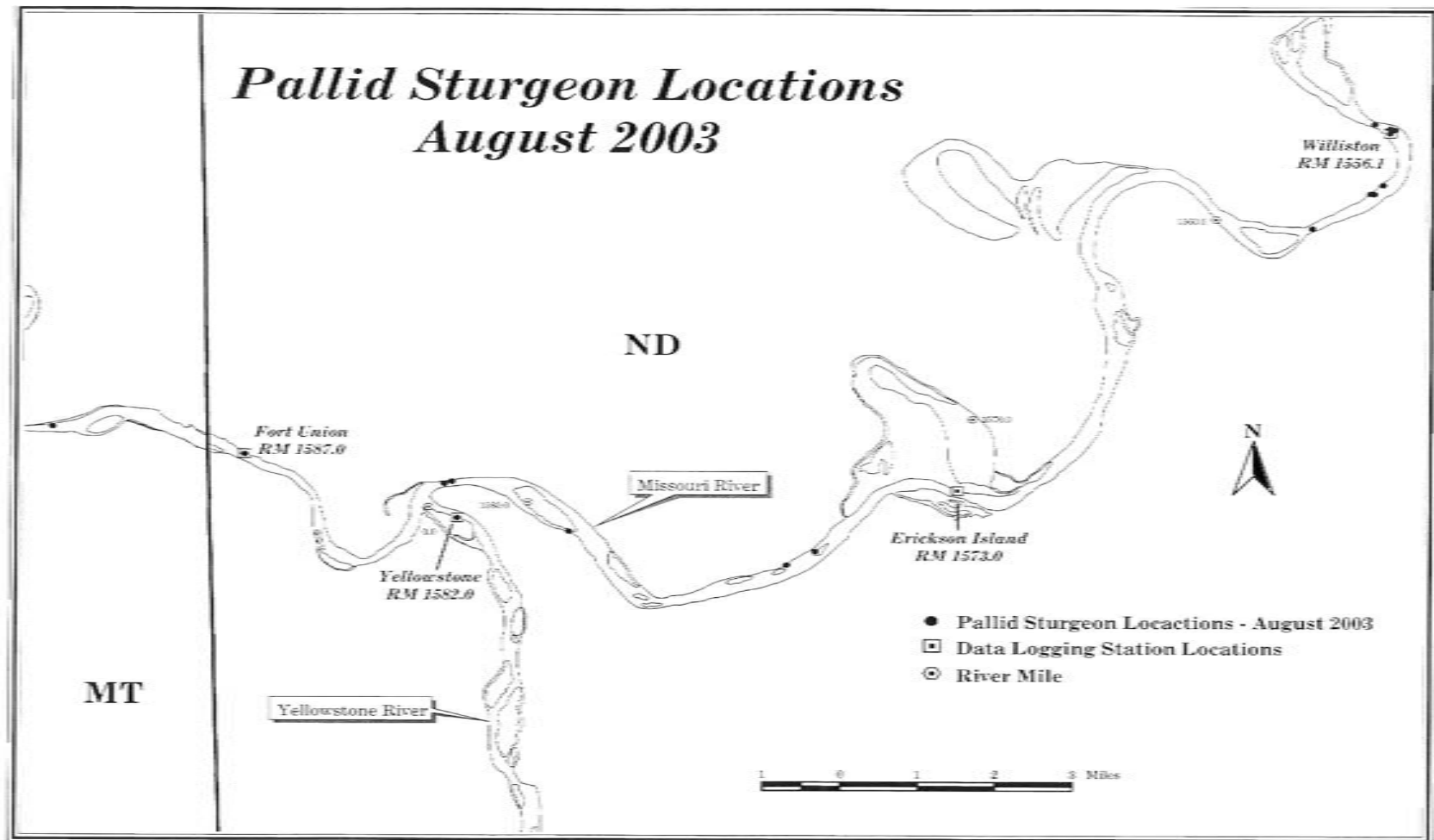
Figure 6. Locations of all pallids in August.
