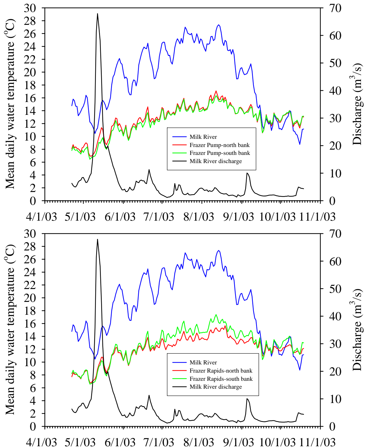
Figure 3. Water temperature profiles and discharge for the Milk River, and water temperatures profiles for the Missouri River at Frazer Pump and Frazer Rapids during 2003.
