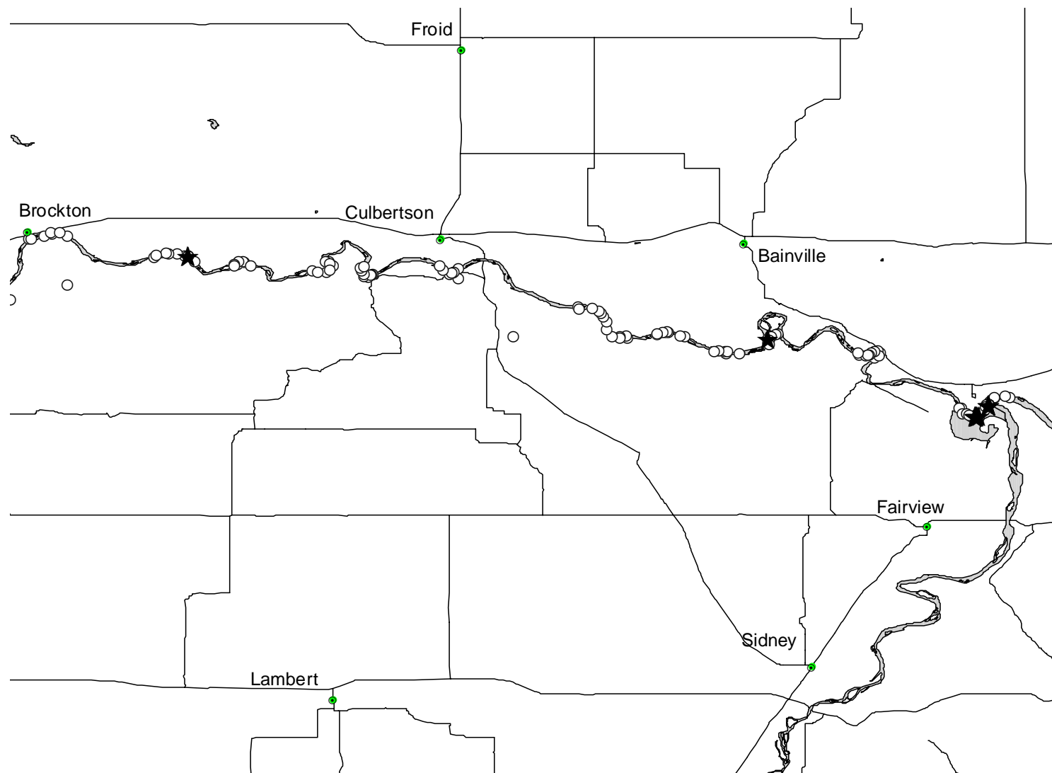
Figure 7. Sites sampled (white circles) with drifted trammel nets and recapture sites (black stars) of hatchery-reared pallid sturgeon from near Brockton, MT to near the confluence of the Missouri and Yellowstone rivers, ND during 2003.
