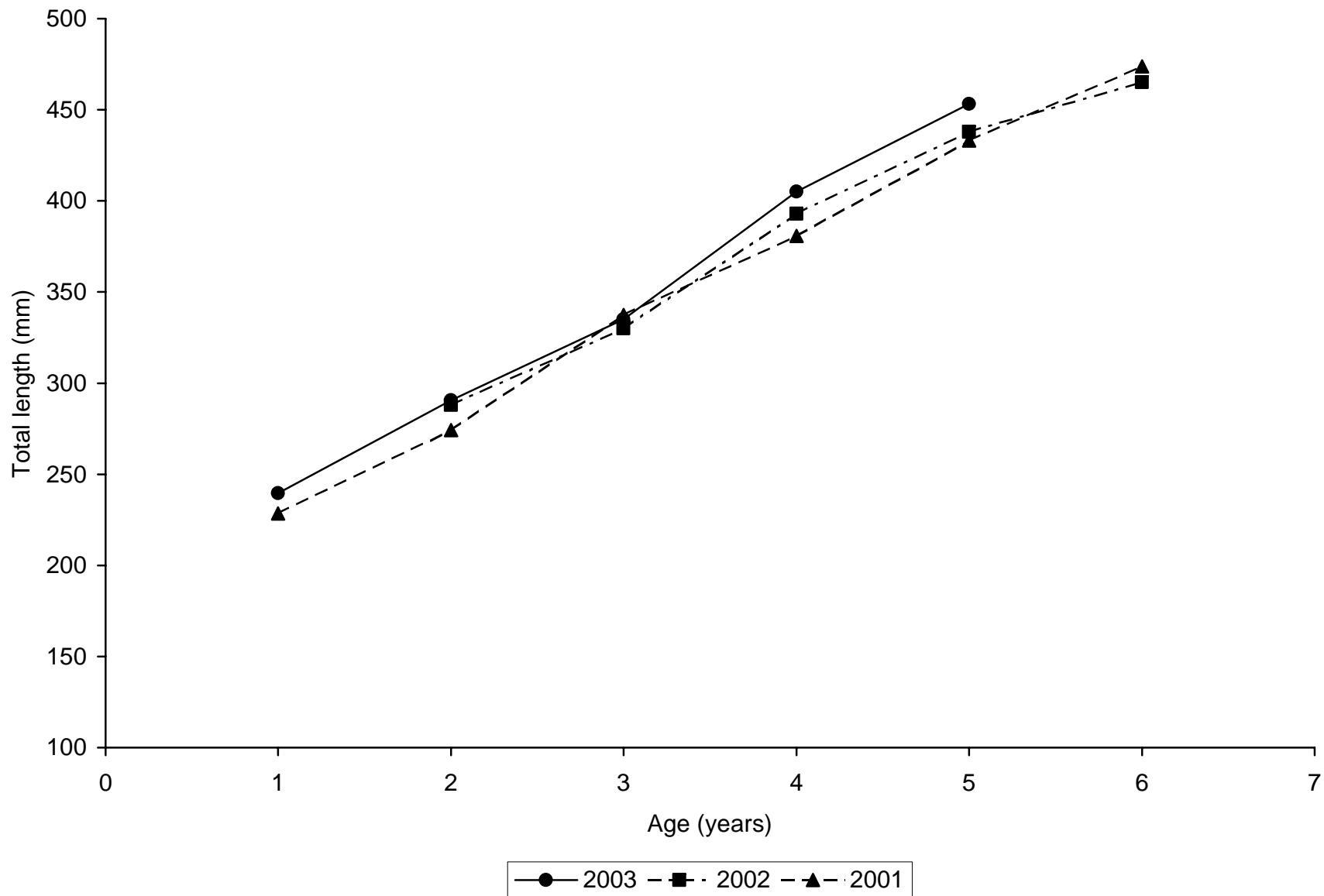
Figure 19. Mean total length at age for sauger sampled in the study area during 2001-2003.
