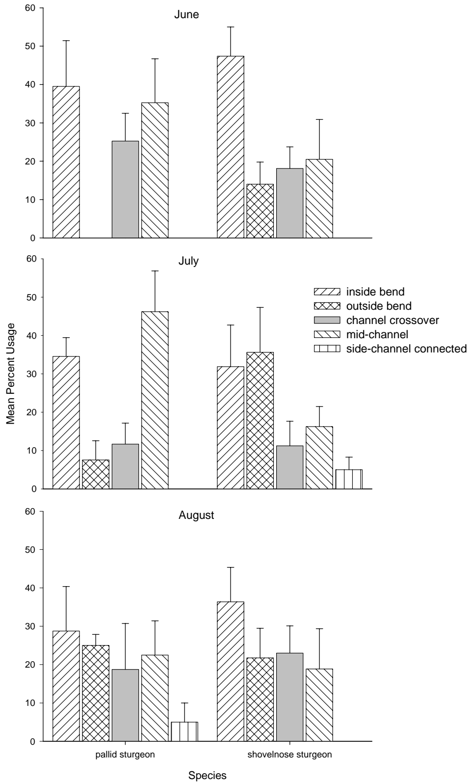
Figure 1. - Mean percent use by macrohabitat and month for HRJPS and JSNS.
