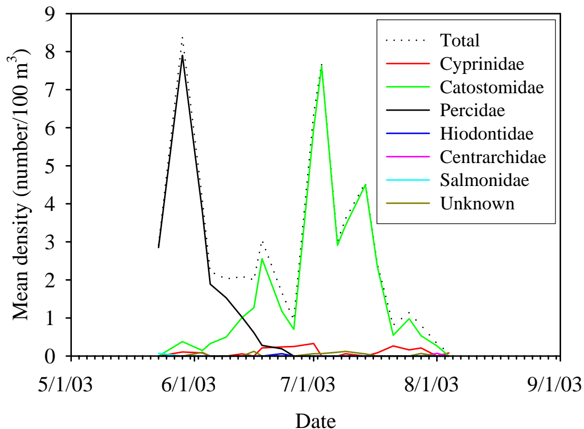
Figure 18. Mean density (number/100 m 3 ) by date of all larval fishes (Total), Catostomidae, Cyprinidae, Hiodontidae, Percidae, Centrarchidae, Salmonidae and unknown sampled in the Missouri River at Wolf Point during 2003.
