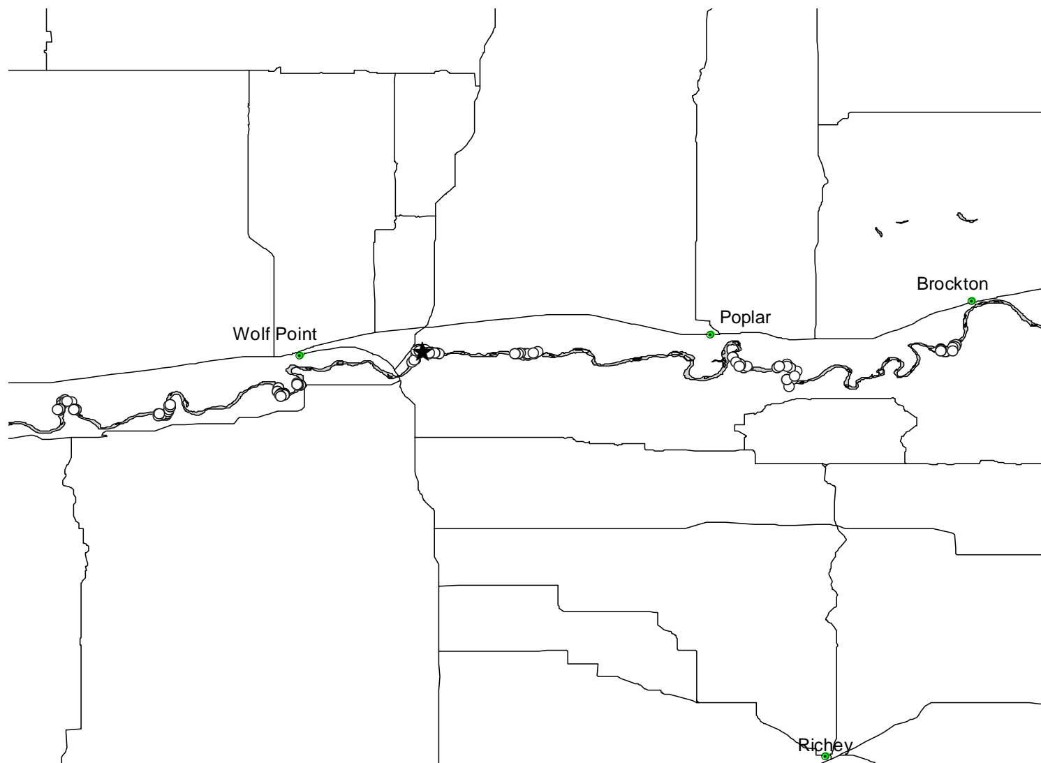
Figure 8. Sites sampled (white circles) with setlines and recapture sites (black stars) of hatchery-reared pallid sturgeon from near Oswego to near Brockton, MT during 2003.
