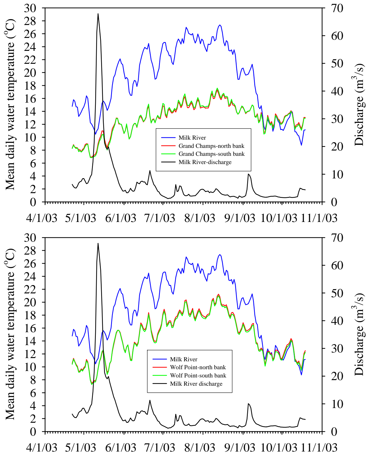
Figure 4. Water temperature profiles and discharge for the Milk River, and water temperatures profiles for the Missouri River at Grand Champs and Wolf Point during 2003.
