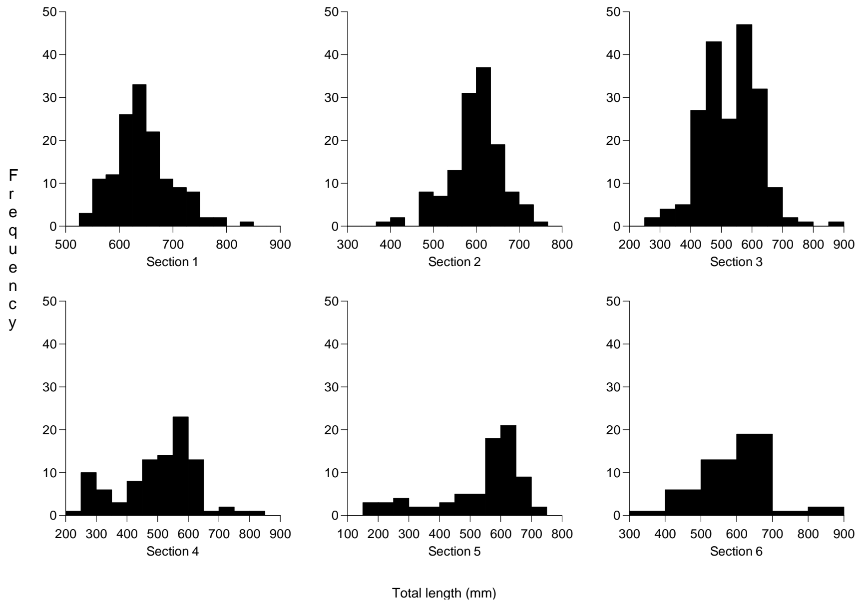
Figure 21. Fork length-frequency plots by study section for shovelnose sturgeon sampled during 2003.
