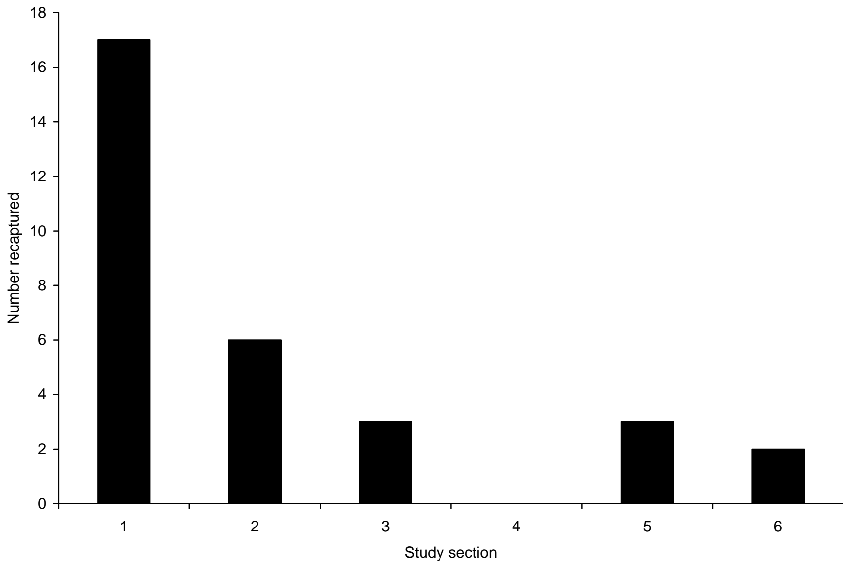
Figure 22. Number of previously tagged shovelnose sturgeon recaptured by study section during 2003.
