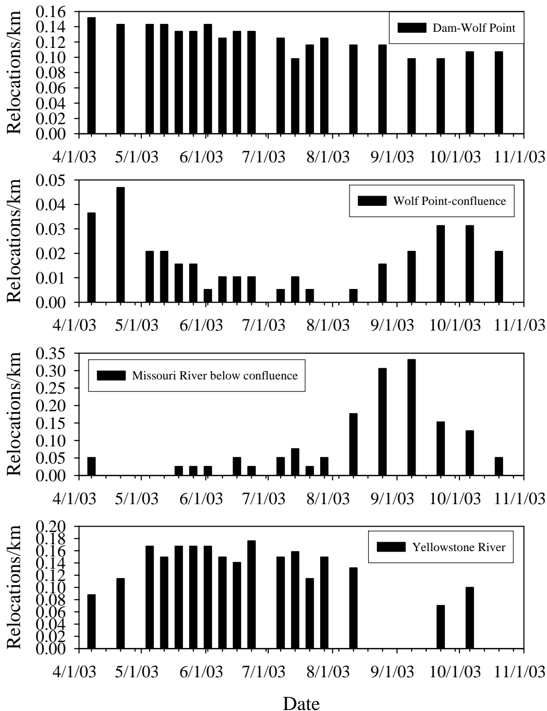
Figure 13. Number of shovelnose sturgeon relocations per km in reaches of the Missouri River and Yellowstone River during 2003.
