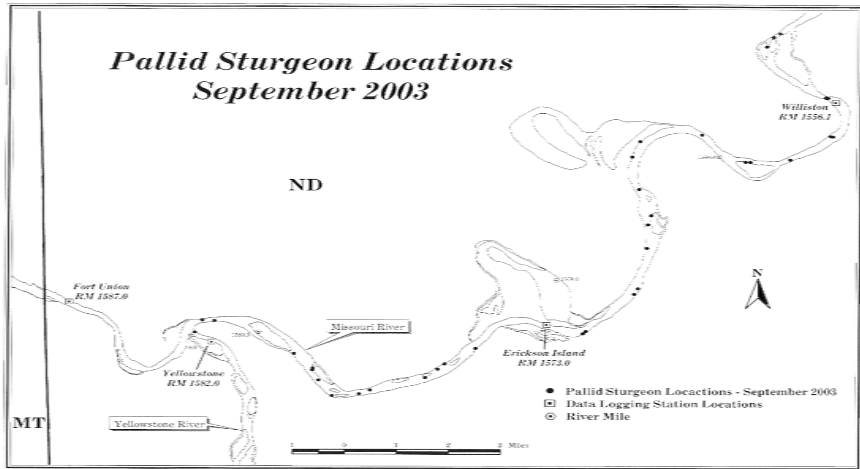
Figure 7. Locations of all pallids in September.
