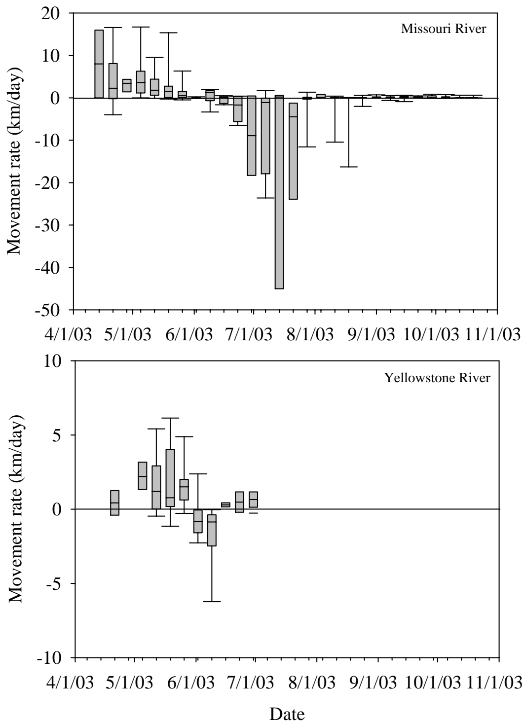
Figure 12. Box and whisker plots of net movement rates (km/day) of paddlefish in the Missouri River and Yellowstone River during 2003. Median movement rate is denoted as a line within the box. The box delimits 25 th and 75 th percentiles of the data, and whiskers delimit the 5 th and 95 th percentiles.
