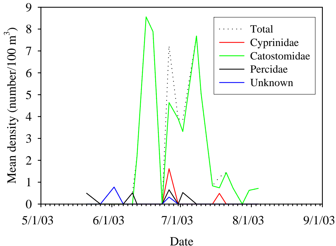
Figure 16. Mean density (number/100 m 3 ) by date of all larval fishes (Total), Catostomidae, Cyprinidae, Percidae, and unknown sampled in the Fort Peck spillway channel during 2003.
