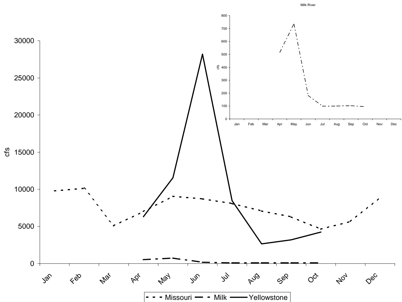
Figure 2. Mean monthly discharges during 2003 for the Yellowstone River at Sidney (solid line), Missouri River below Fort Peck Dam (dashed line), and the Milk River at Nashua (bar-dash-bar line). Inserted graph shows the Milk River data at a smaller scale. Provisional data provided by USGS, Fort Peck Field Office, Fort Peck, MT.
