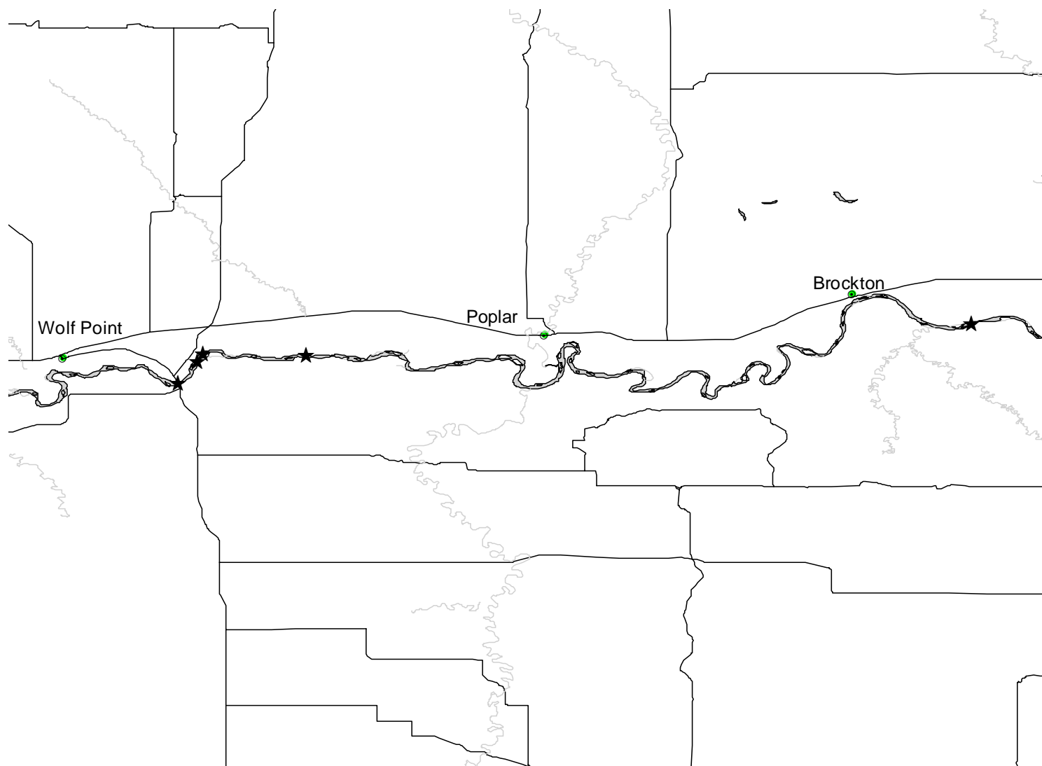
Figure 11. Recapture sites (black stars) of hatchery-reared pallid sturgeon recaptured from near Wolf Point to near Brockton, MT during 6 August-14 October 2003.
