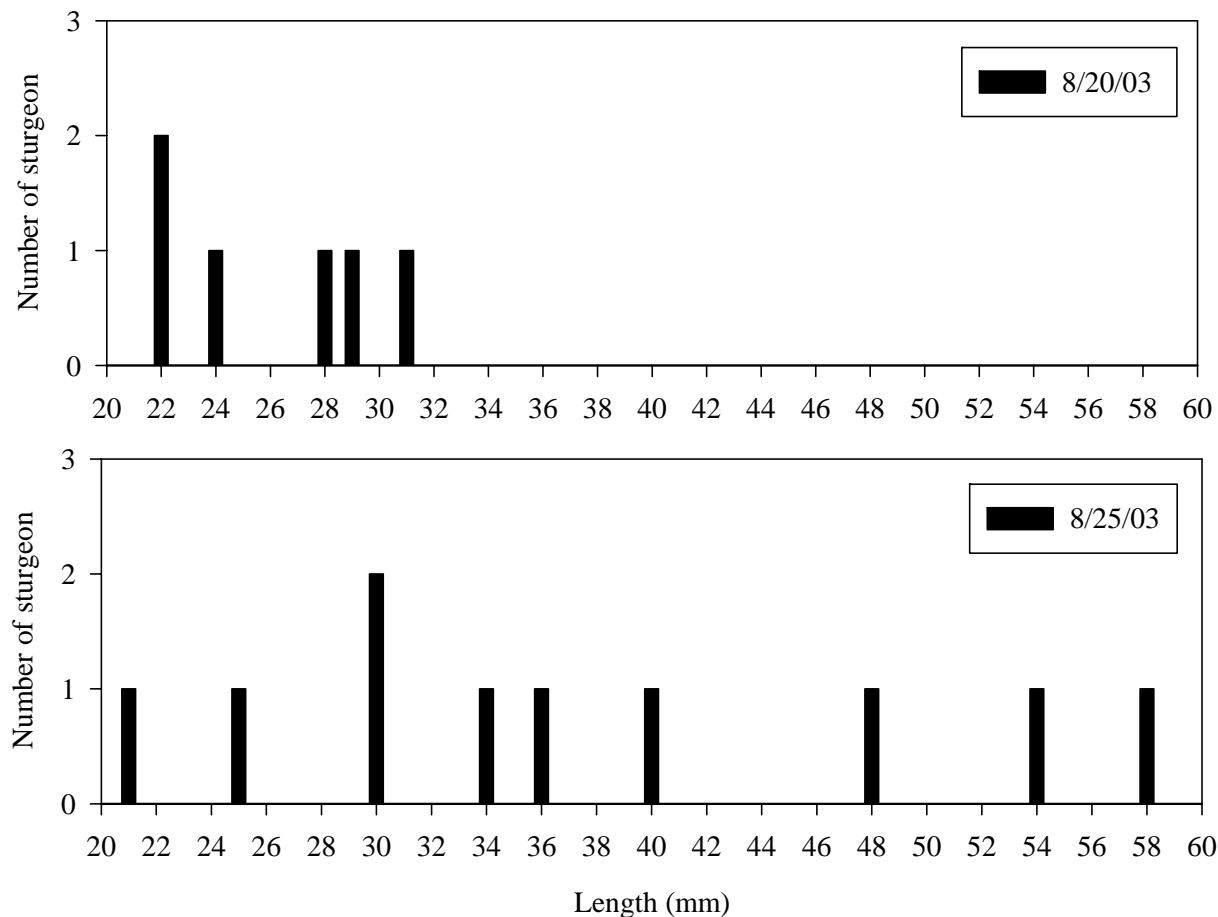
Figure 22. Length distributions of young-of-year sturgeon sampled during 2003 in the Missouri River above the confluence (ATC) of the Yellowstone River.
