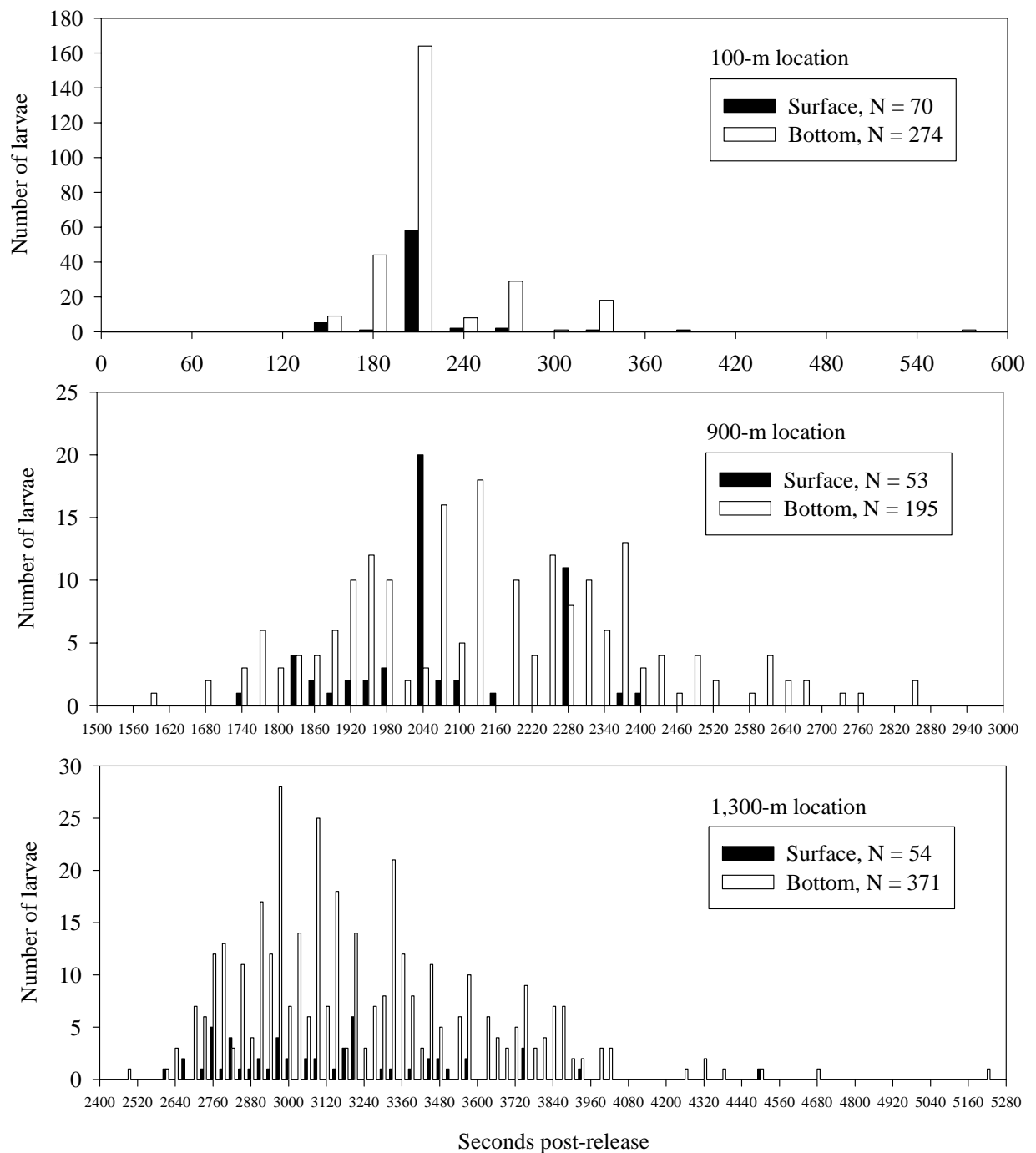
Figure 4. Number of larval shovelnose sturgeon sampled by time in surface and bottom nets at the 100-m, 900-m, and 1,300-m sampling locations on June 27. Sampling continued for 900 sec, 1,800 sec, 3,600 sec, and 5,400 sec post-release for the increasing sampling location distances, respectively, but the abscissa is truncated.
