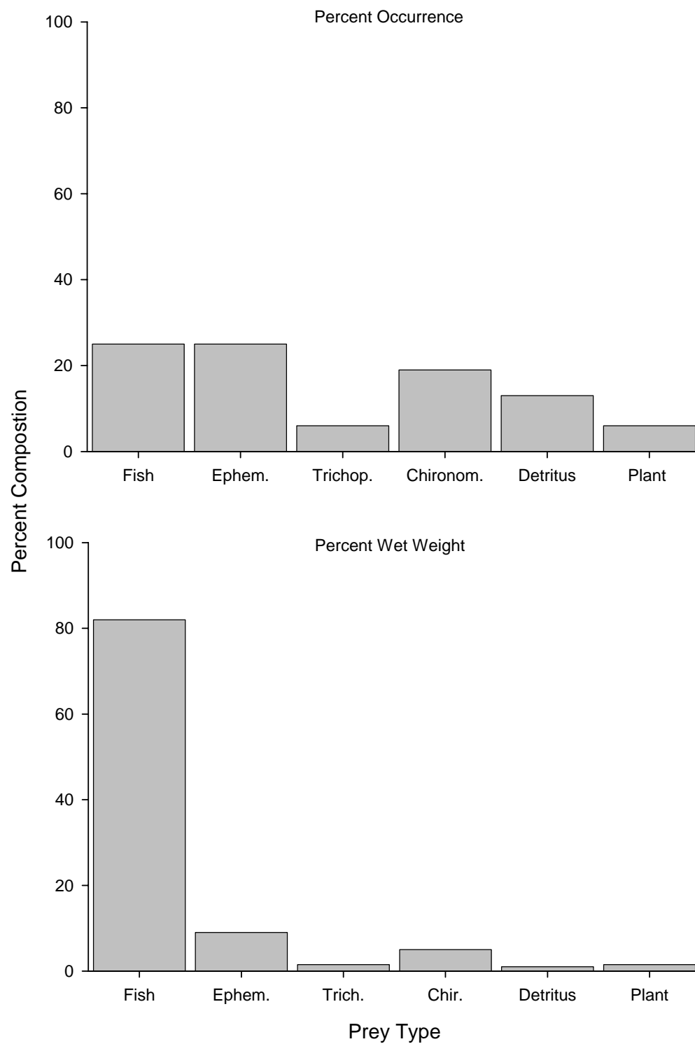
Figure 3. - Percent composition by occurrence and wet weight for HRJPS diets in 2003.
