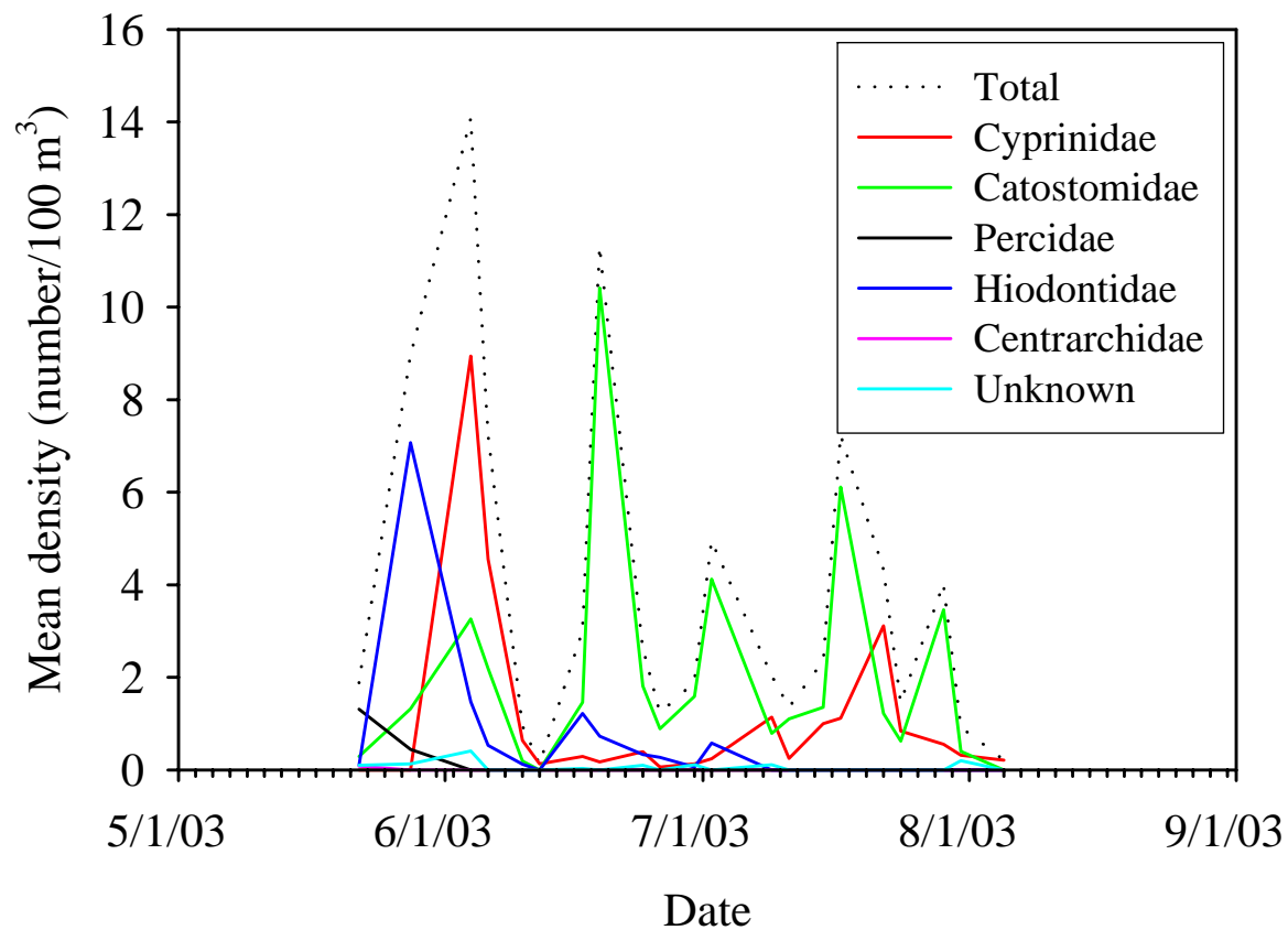
Figure 20. Mean density (number/100 m 3 ) by date of all larval fishes (Total), Catostomidae, Cyprinidae, Hiodontidae, Percidae, Centrarchidae, and unknown sampled in the Yellowstone River during 2003.
