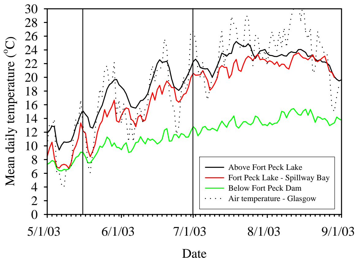
Figure 6. Mean daily water temperature at three sites (Missouri River above Fort Peck Lake, in the spillway bay, below Fort Peck Dam) and mean daily air temperature measured at Glasgow, Montana, during 2003. For reference, the vertical lines delimit dates when the proposed mini-test and full-test are to be conducted when sufficient water levels are available in Fort Peck Lake.
