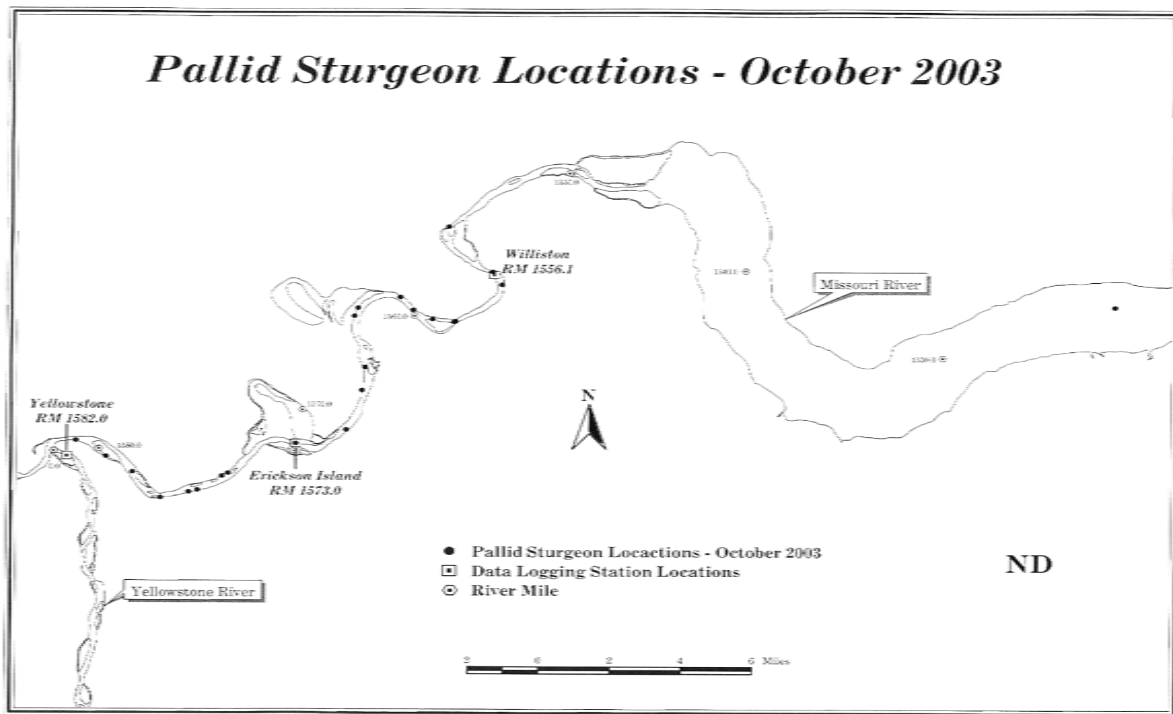
Figure 8. Locations of all pallids in October.
