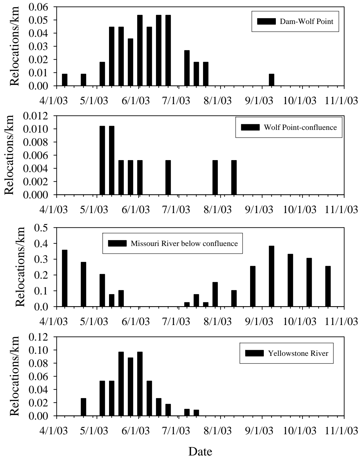
Figure 11. Number of paddlefish relocations per km in reaches of the Missouri River and Yellowstone River during 2003.
