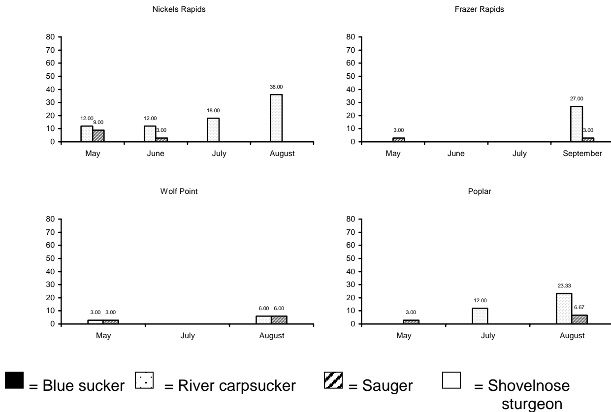
Figure 28. CPUE rates (number per hour sample time) for blue sucker, river carpsucker, sauger, and shovelnose sturgeon sampled in electrofishing runs at standardized sites on the Missouri River, MT, during 2003.
