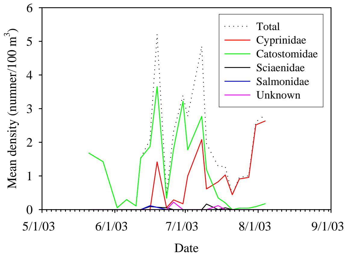
Figure 17. Mean density (number/100 m 3 ) by date of all larval fishes (Total), Catostomidae, Cyprinidae, Sciaenidae, Salmonidae, and unknown sampled in the Milk River during 2003.
