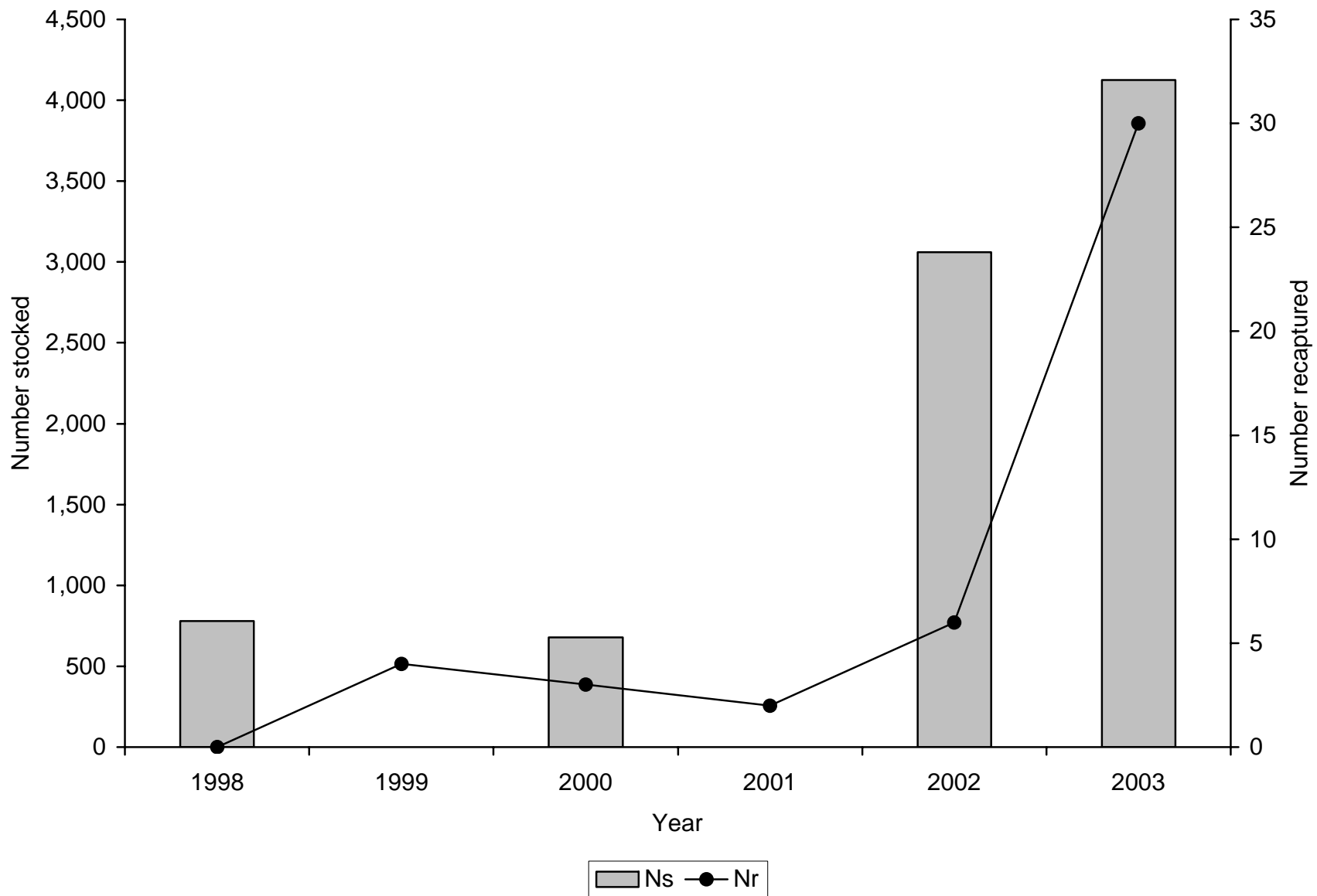
Figure 12. Number stocked ( N_s ) and number recaptured ( N_r ) verses year for hatchery-reared pallid sturgeon in the study area during 1998-2003.
