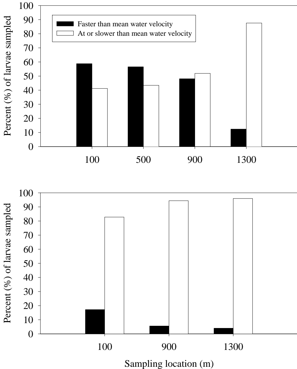
Figure 5. Percent of larval shovelnose sturgeon drifting faster than, and at or slower than mean water velocity by sampling location on June 25 (top panel) and June 27 (bottom panel).
