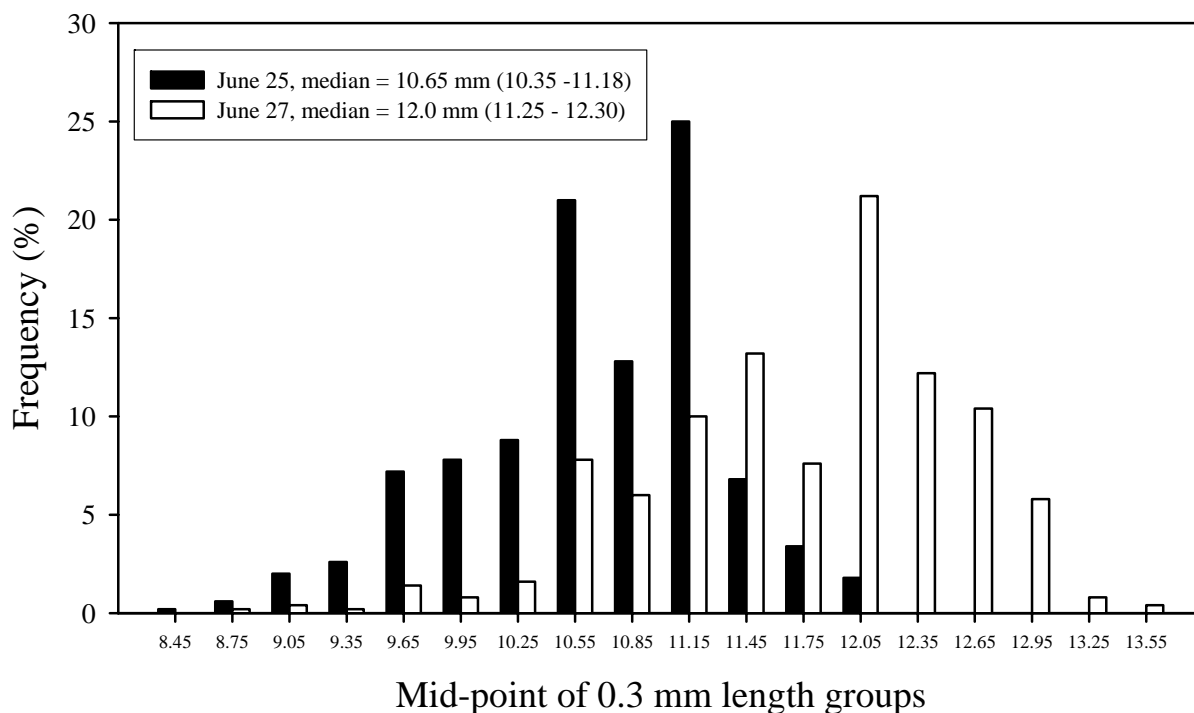
Figure 2. Length-frequency histogram of 500 randomly selected larval shovelnose sturgeon sampled on June 25 and June 27. Hyphenated values in parentheses are the 25% - 75% length quartiles.
