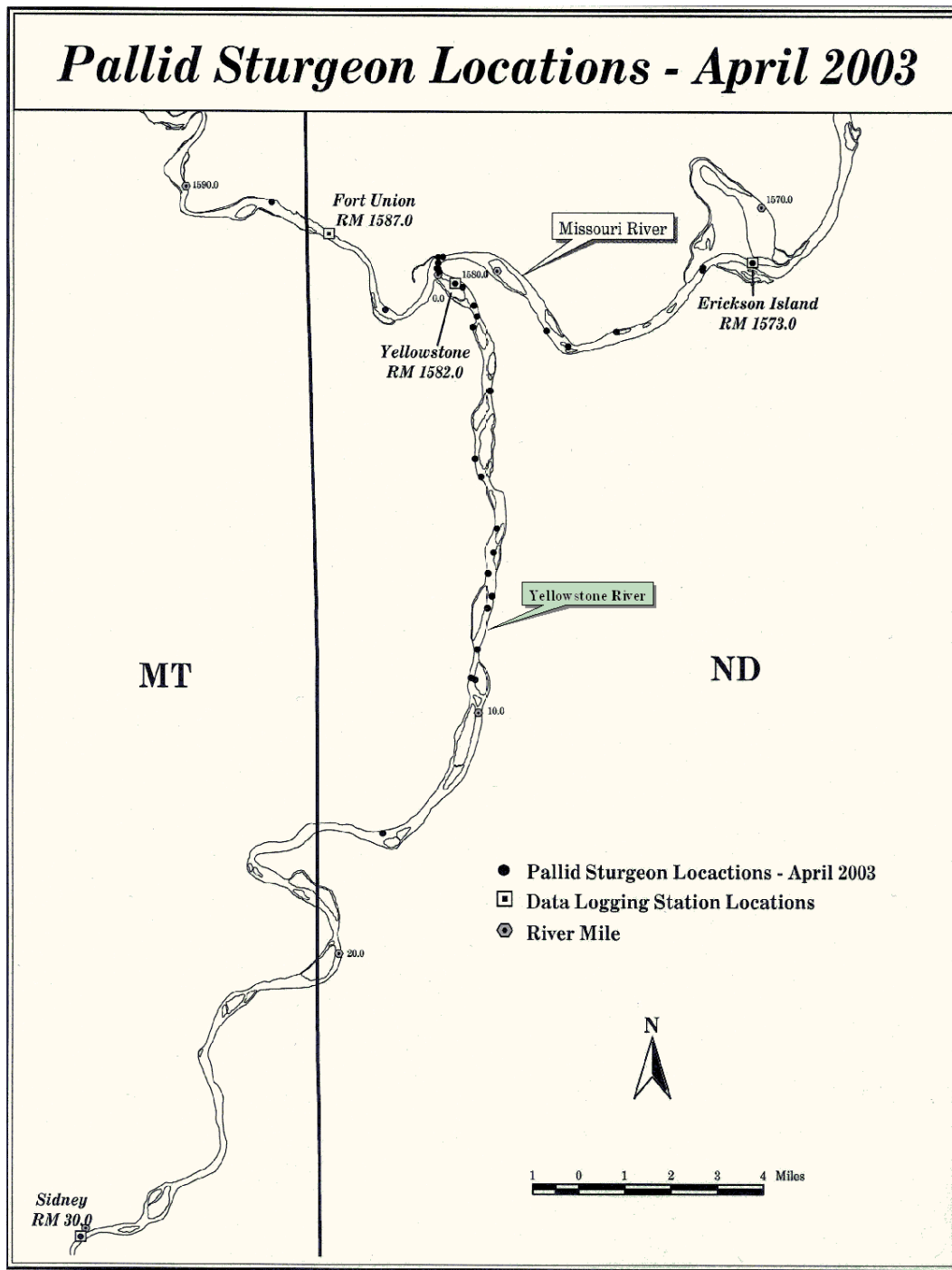
Figure 2. Locations of all pallids in April.
